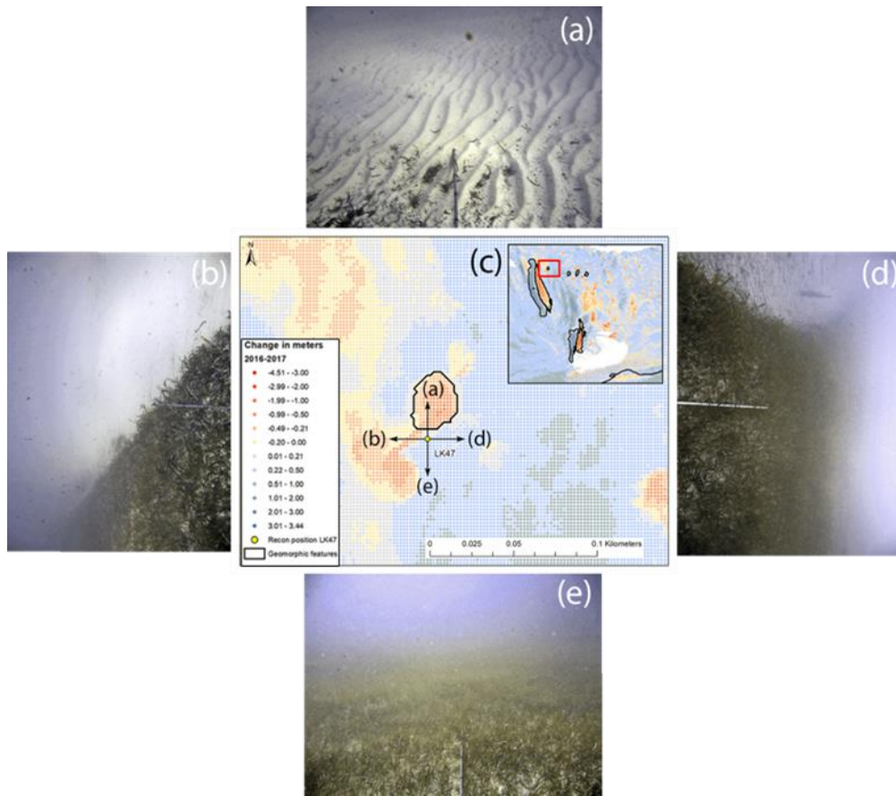
Figure 8. Cardinal orientation imagery (a, b, d, and e represent north, west, east, and south, respectively) and elevation change (c) at a scour mark location used to validate benthic features observed in elevation change data. East and west arrows show the boundaries between seagrass beds and sand flats in the elevation change data (c) and imagery (b and d). High erosion was noted between 2016 and 2017 on the sand flat (western) side of the habitat transition and minimal accretion was noted on the seagrass bed (eastern) side of the habitat transition. Photo credit: Mitch Lemon, Cherokee Nations System Solutions for U.S. Geological Survey.
