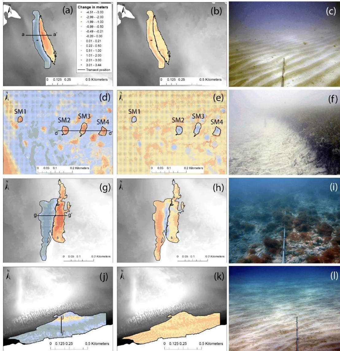
375 Figure 6. Elevation change data and transect positions for each geomorphic feature subarea. Geomorphic features included a sand 380 Figure 6. Elevation change data and transect positions for each geomorphic feature subarea. Geomorphic features included a sand wave (a, b, c), scour marks (d, e, f), western rubble field (g, h, i), and sand lobe subareas (j, k, l). These feature locations and corresponding habitat are also shown in Fig. 4. Elevation-change from 2016 to 2017 (a, d, g, j), 2017 to 2019 (b, e, h, k), and corresponding reconnaissance imagery (c, f, i, l) Transect positions are indicated by black lines and lowercase letters in the elevation change panels (see also Fig. 7). Scour marks in panels d and e are labelled SM1 through 4. Photo credit: Mitch Lemon, Cherokee Nations System Solutions for U.S. Geological Survey.
