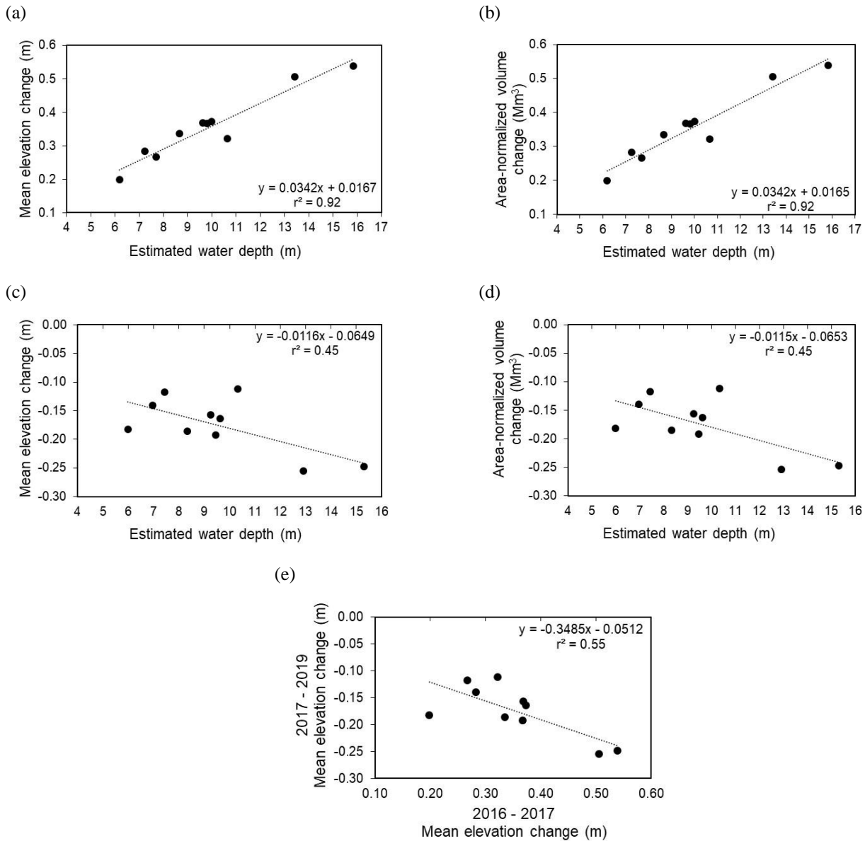
315 Figure 5. Linear relationships between elevation change, volume change, and water depth. Linear relationships and coefficients of 320 determination between (a) mean elevation change, (b) mean area-normalized volume change, and estimated 2016 mean water depth for seafloor habitats of the Looe Key study site between 2016 to 2017. Linear relationships and coefficients of determination between (c) mean elevation change, (d) mean area-normalized volume change, and estimated 2017 mean water depth for seafloor habitats of the Looe Key study site between 2017 to 2019 (a, b). Linear relationship between 2017 to 2019 mean elevation change and 2016 to 2017 mean elevation change (e).
