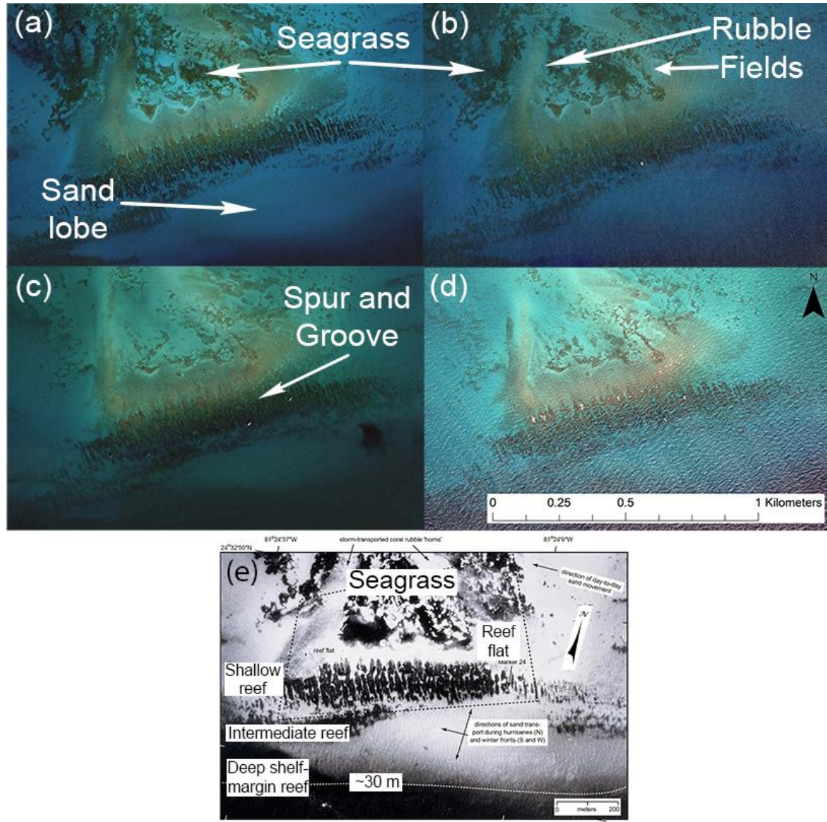
510 Figure 9. Historical satellite and aerial imagery of Looe Key Reef. Imagery from (a) 17 December 2014, before Hurricane Irma; (b) 18 March 2017, before Hurricane Irma; (c) 30 December 2017, 3 months after Hurricane Irma; (d) 2019, 16.5 months after Hurricane Irma; and (e) from 1975 (Lidz et al., 2016). Panels a, b, and c source: Maxar 2023 via Google Earth Pro 7.3.6.9345, downloaded 11 September 2023. Panel d source: 2019 NOAA National Geodetic Survey via NOAA Digital Coast, downloaded 11 September 2023, https://www.fisheries.noaa.gov/inport/item/63292 .
