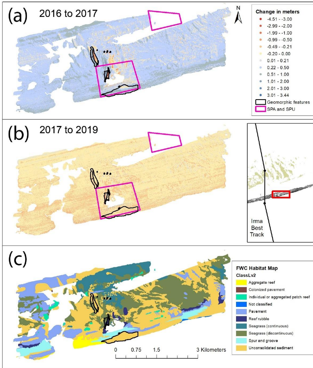
260 Figure 4. Elevation-change results for 4,007,961 point-locations at Looe Key Reef. Elevation change between (a) 2016 to 2017 (13.5 265 months before and 3 to 6 months after Hurricane Irma) and (b) between 2017 to 2019 (from approximately 3 to 16.5 months after Hurricane Irma), and (c) corresponding seafloor habitats (FWC, 2015). The Hurricane Irma best track data in the panel b's inset is from the NOAA NHC Irma Storm Track resource page (NHC, 2018, see also Figure 2b). Boundaries for the Looe Key Sanctuary Protection Area (SPA) and Special Protection Unit (SPU) are shown as pink polygons. Geomorphic features of interest are indicated with black polygons. Gaps in map areas indicate locations where water depth was too shallow for collection of multibeam bathymetric data.
