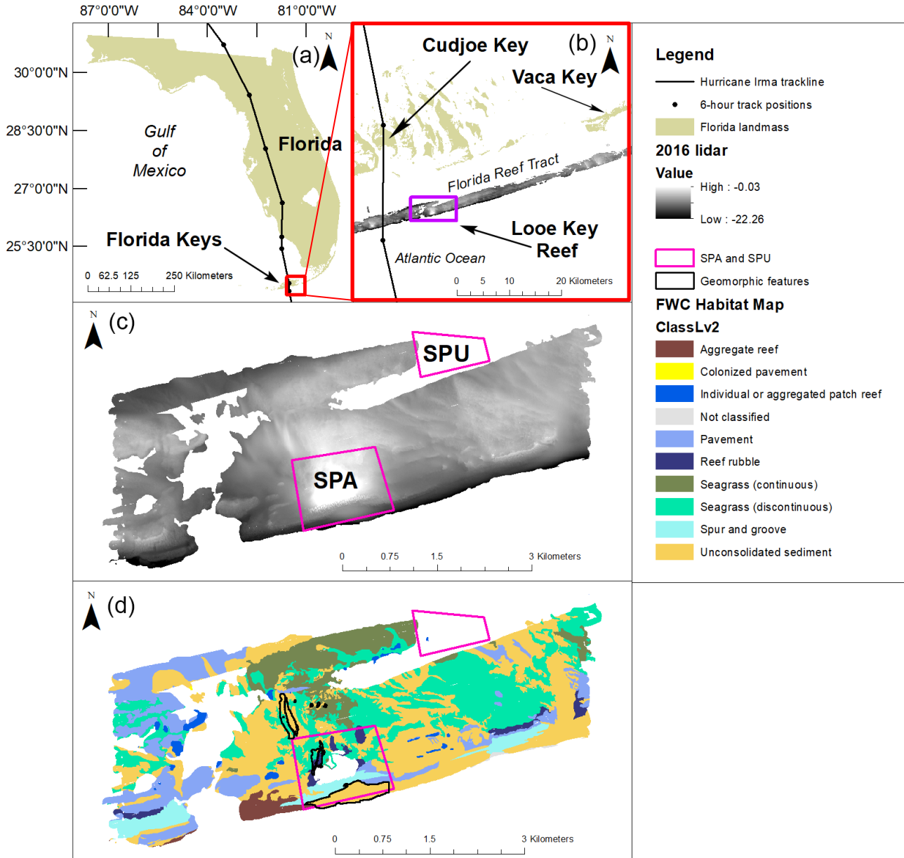
155 Figure 2. Looe Key Reef location, bathymetry, and seafloor habitats. (a) Location of the Florida Keys along the southern coast of Florida, trackline of Hurricane Irma and the location of its landfall (red box). (b) Proximity of Hurricane Irma's trackline to the Looe Key Reef study site (purple box), location of landfall at Cudjoe Key, and location of Vaca Key where the nearest NOAA-NOS (2023) Tides and Currents station was located. (c) 2016 lidar bathymetric map of the Looe Key Reef study site showing location of Florida Keys National Marine Sanctuary Special Preservation Area (SPA), Special Use Area (SPU), and geomorphic features of focused investigation for this study. (d)
