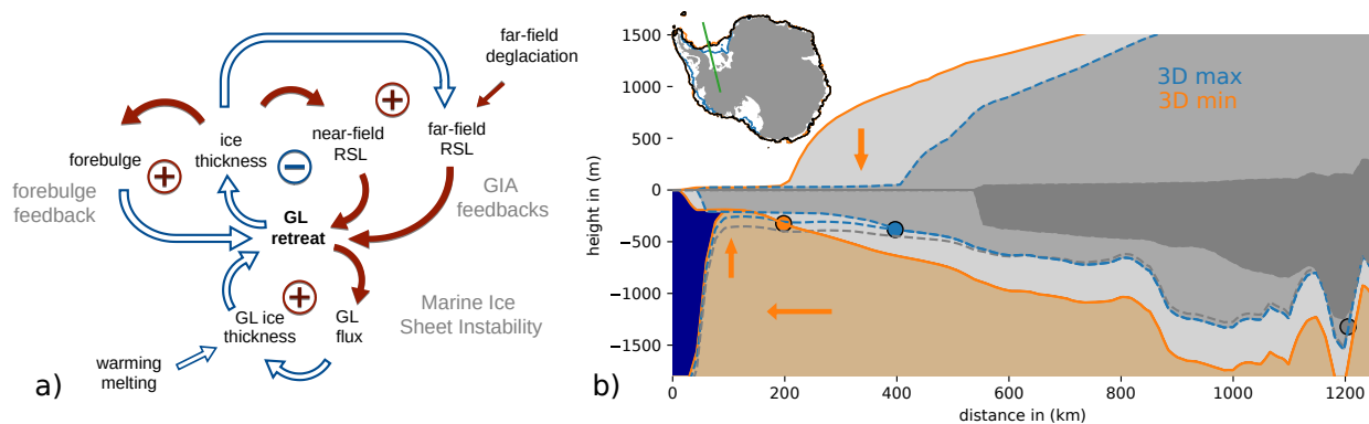
Figure 11. MISI and GIA feedbacks on grounding line migration. a) Feedback loops show the stabilizing near-field RSL feedback on grounding line (GL) retreat (-) and the self-sustaining forebulge feedback (+) as well as the far-field (barystatic) RSL feedback (+). The Marine Ice Sheet Instability (MISI) represents a self-amplifying ice-internal feedback on GL retreat on retrograde slopes (+), which can be triggered by ocean-induced melting. Amplifying effects are indicated by red filled arrows (e.g. GL retreat leads to more GL flux), dampening effect by non-filled blue arrows (e.g. more GL flux results in less ice thickness at the GL). b) Transect shows bedrock elevation and outlines of ice sheet and ice shelf at LGM through Ronne embayment from the continental shelf edge to the present-day GL position for the two Antarctic end members of the reference 3D Earth structure, ‘3D max’ and ‘3D min’. Respective GL positions (dots) are about 200 km apart. Orange arrows indicate additional ice mass, subsidence of the underlying bedrock, lateral displacement of mantle material and subsequent forebulge uplift (see also Video S2). Dark grey shading and dot indicate present-day observed ice sheet configuration and GL position, respectively. Green line in inset indicates transect location.
