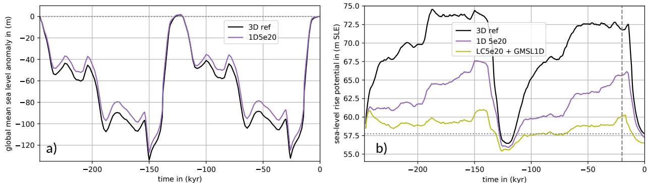
Figure 9. Comparison of global mean RSL a) and SLRP from Antarctica b) over last 246 kyr for Earth models of different complexity. Olive colored for the Lingle-Clark bed deformation model with 100-yr coupling time step, upper mantle viscosity of 5 \times 10^{20} Pa s (‘LC 5e20’) and 88 km lithosphere thickness ( 5 \times 10^{24} Nm flexural rigidity), suggesting a loss of about 3 m SLE in SLRP since LGM. Purple for the coupled PISM-VILMA model with 100-yr coupling time step, a 1D-Earth structure with 88 km thick elastic lithosphere and 5 \times 10^{20} Pa s viscosity in the mantle below (‘1D 5e20’). This simulation also solves for the sea-level equation, yielding a 7 m SLE larger contribution since LGM. The global mean of the sea level is used as forcing for the simulation with the LC model (‘GMSL1D’). In black, the AIS response to the reference 3D Earth structure ‘3D ref’ is shown with more than 14 m SLE change in SLRP since LGM.
