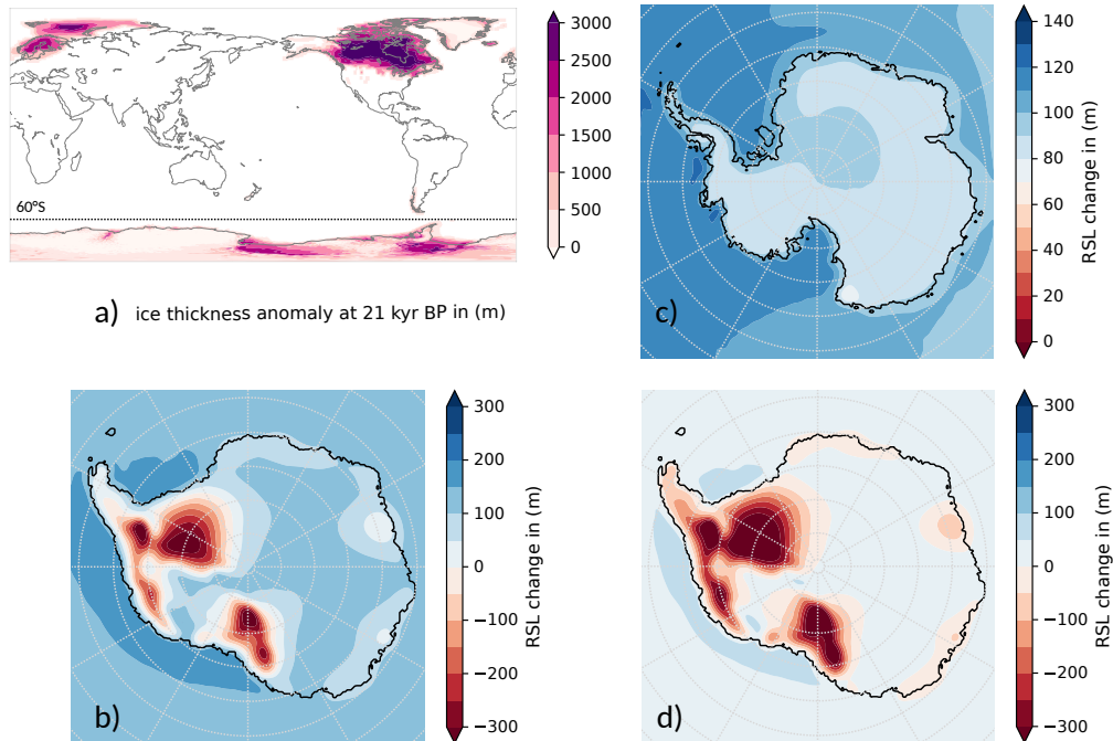
Figure 10. Far-field and near-field contributions to RSL changes in Antarctica since LGM, analogous to Fig. 1 in Gomez et al. (2020)
