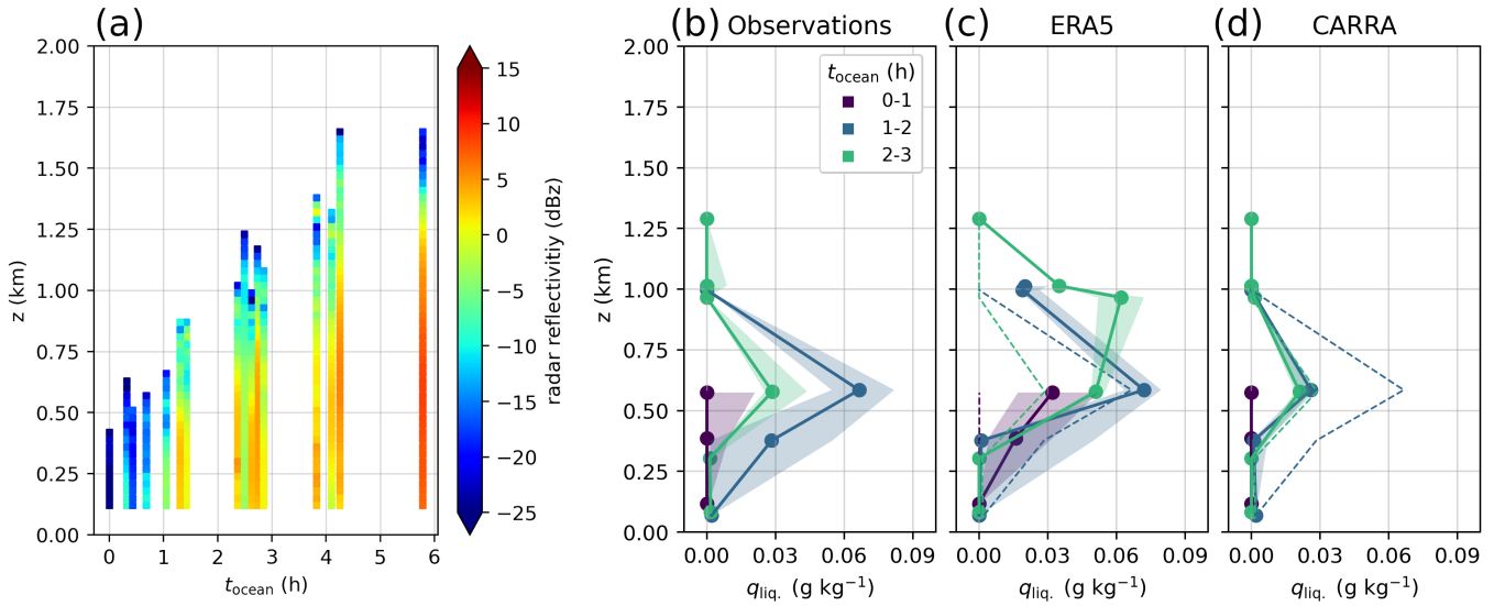
Figure 9. Vertical profiles of cloud structures, sorted by time air masses spent over ice-free ocean. a) Profiles of the HAMP radar reflectivities measured aboard HALO. b) Profiles of cloud liquid water content q_{\text{liq}} , based on a Nevzorov sonde aboard Polar 6, c) q_{\text{liq}} , taken from ERA5, with the observed values as dashed lines, and d) q_{\text{liq}} , taken from CARRA, with the observed values as dashed lines.
