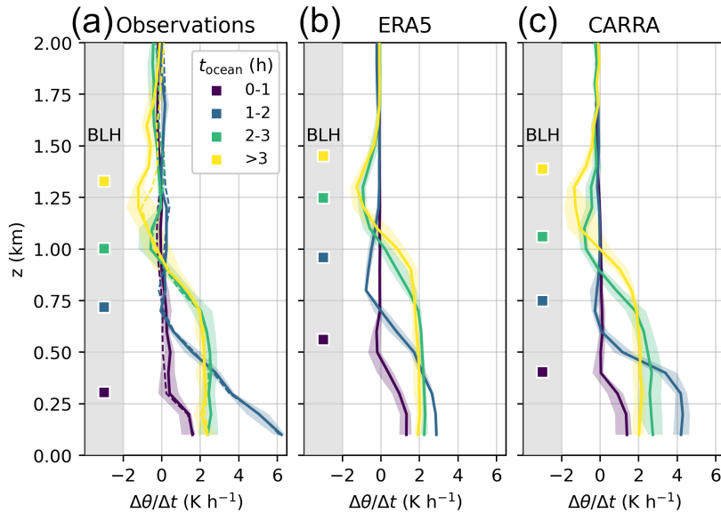
Figure 6. Diabatic heating rates grouped by time air masses spent over the ice-free ocean. On the left side of each panel, the mean BLH in each class is plotted as square. Lines depict the mean values, shading the 25-75 quantiles. a) Heating rates based on the quasi-Lagrangian dropsonde observations. Solid lines are from ERA5 trajectories, the dashed lines show the mean rates from CARRA. b) Corresponding heating rates extracted from ERA5. c) Corresponding heating rates extracted from CARRA.
