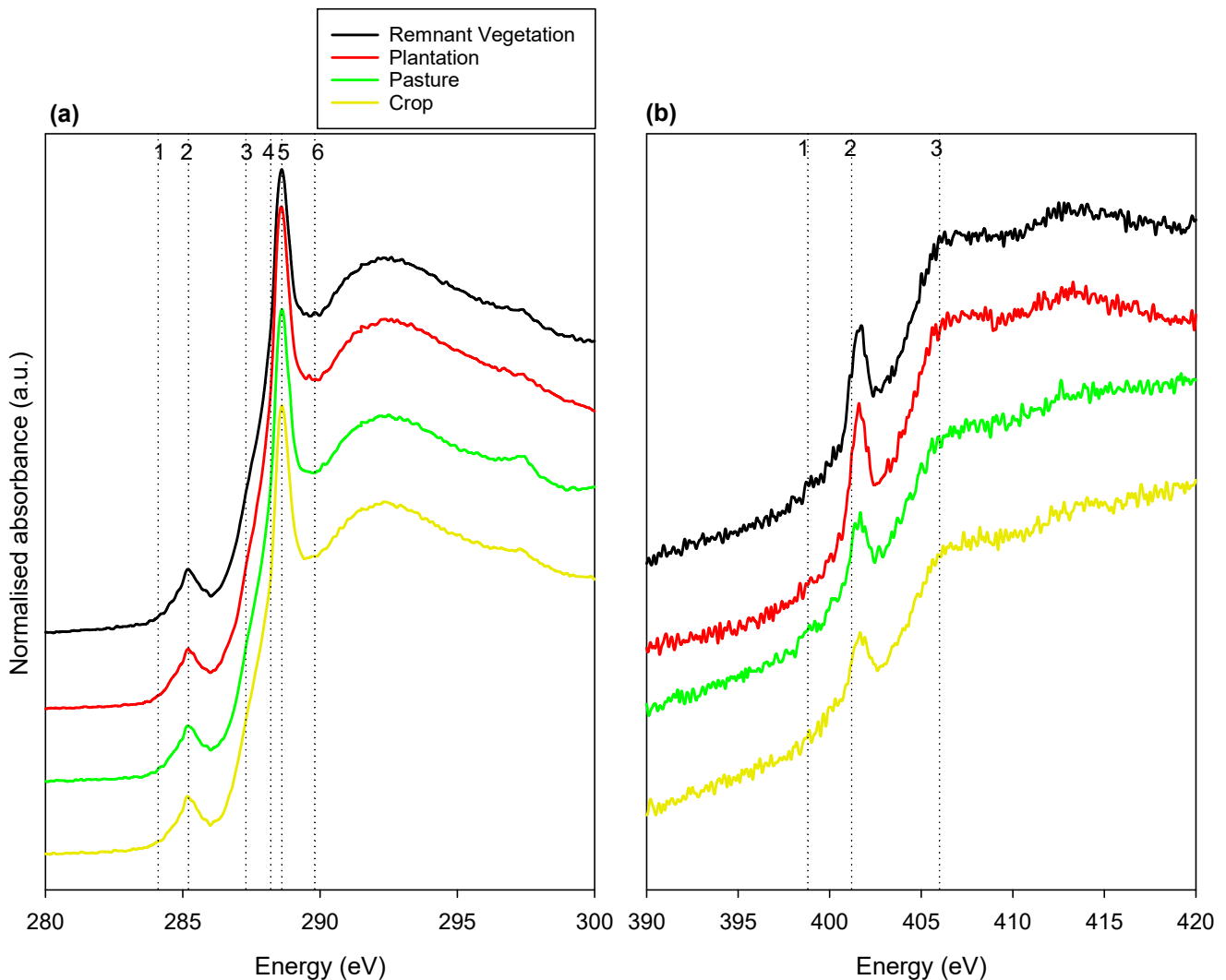
290 Fig. 43: Double normalised (a) C K-edge spectra and (b) N K-edge spectra of finely ground bulk soil samples from each land use produced by near edge X-ray absorption fine structure. Spectra have been stretched in the y direction to visualise each land use. (a) Vertical lines indicate (1) quinones at 284.7 eV, (2) aromatic C at 285.5 eV, (3) aliphatic C/phenolic C-OH at 287.3 eV, (4) aliphatic C at 288.2 eV, (5) carboxyl C-OOH at 289.0 eV and (6) O-alkyl-C carboxyl C-OOH at 289.8 eV. (b) Vertical lines indicate (1) aromatic N in 6-membered rings at 398.8 eV, (2) amide at 401.2 eV, and (3) alkyl-N at 406 eV.
