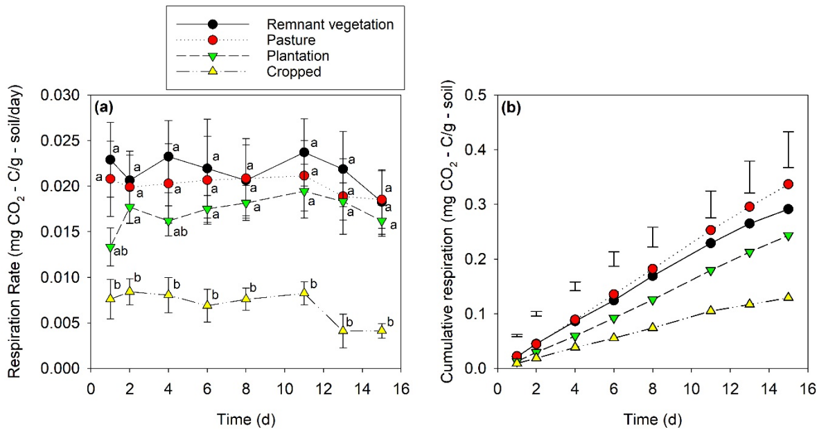
Fig. 24: (a) Mean (with standard error) respiration rates of soil for four land uses. Letters indicate the least significant difference ( P < 0.05 ) between the land uses at each time. (b) Cumulative respiration for four land uses across a 15-d incubation period. Each point represents the mean of five replicates. Error bars indicate least significant differences ( P < 0.05 ) between land uses at each time.
