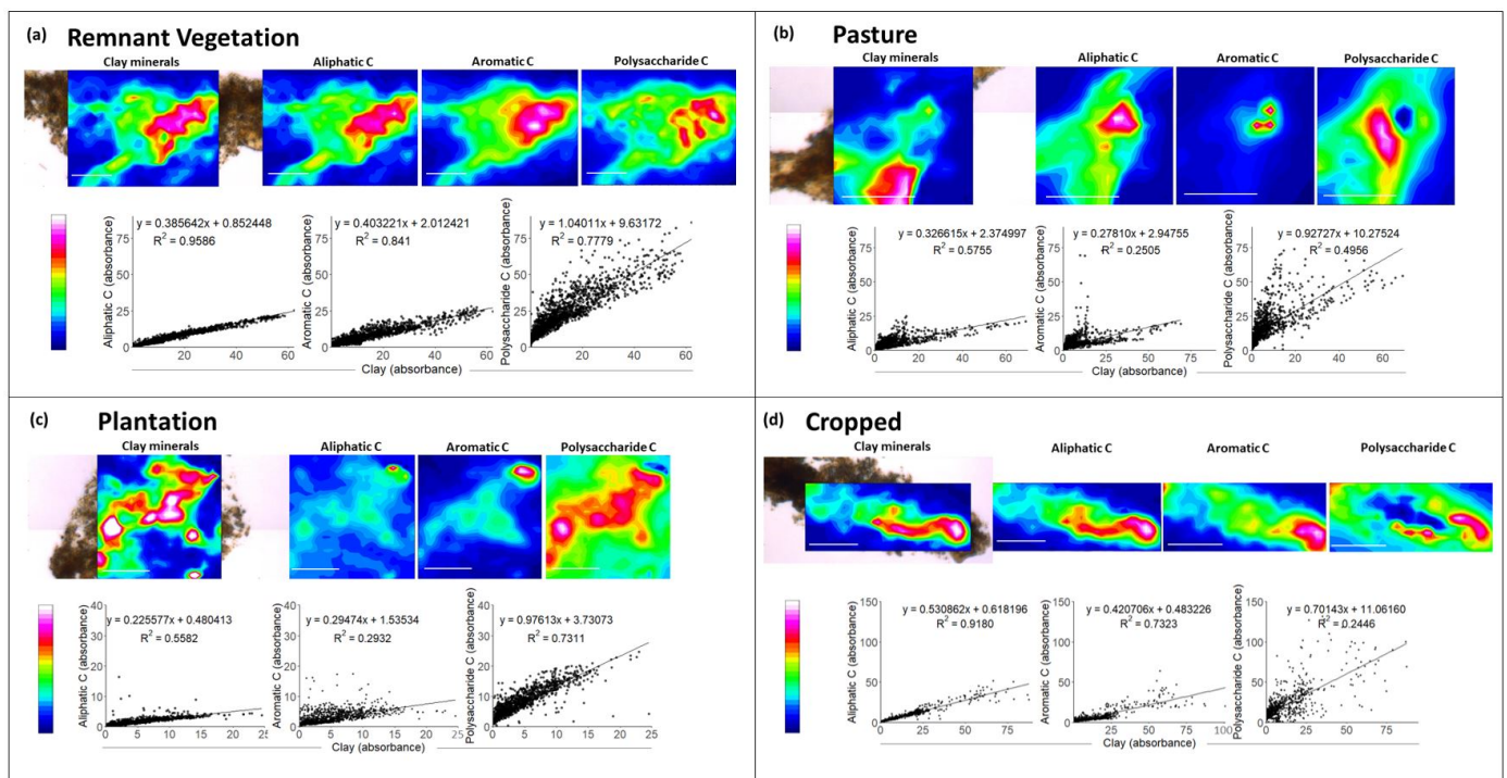
330 Fig. 54: Spectral maps showing the distribution of mineral-OH, aliphatic C, aromatic C and polysaccharide C obtained through synchrotron-based infrared microspectroscopy by analysis of sections (200 nm thickness) obtained from intact microaggregates of soil from four land uses (remnant vegetation, pasture, plantation and cropped) (bars are 25 \mu\text{m} ). The spectral map of one of the two to three replicates analysed for each land use is shown. Maps were obtained from 32 coadded scans (4 \text{cm}^{-1} resolution) with a 2.5 \mu\text{m} step size. The spectra obtained from each map were used to form regression analyses. Pixels where the absorption peak could not be detected above the baseline noise were excluded from regressions.
