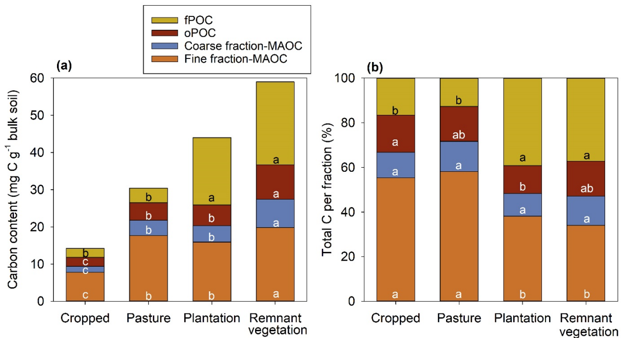
245 Fig. 32: Organic carbon content (a) and the total organic C per fraction (b) for each soil fraction within the bulk soil from topsoils (0-10cm) collected from four land uses. fPOC is free particulate organic carbon, oPOC is aggregate-occluded particulate organic matter, fine fraction-MAOC is coarse grained (> 53 \mu\text{m} ) mineral-associated organic carbon and coarse fraction-MAOC is fine grained (> 53 \mu\text{m} ) mineral-associated organic carbon. Lower-case letters indicate least significant differences ( P < 0.05 ) between the same fractions across land uses— according to REML mixed effects model and Tukey's post hoc testing.
