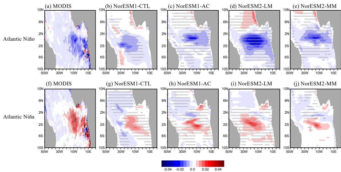
Figure S5 Composite anomalies of primary production for observation and NorESM simulation for (top) Atlantic Niño and (bottom) Atlantic Niña in June-July, respectively.
