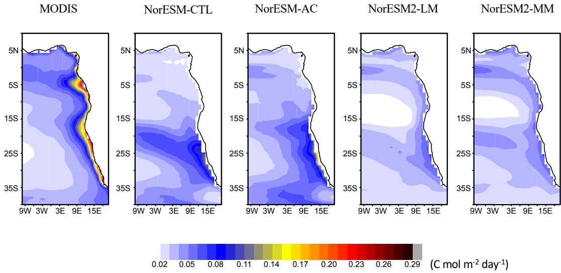
Figure S4 Annual-mean climatology for primary production in observations and each NorESM simulation.
