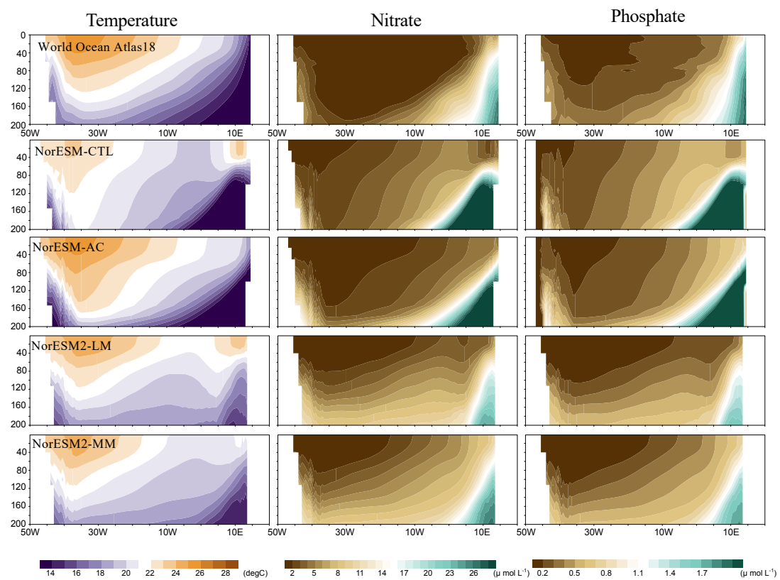
Figure S3 Depth-longitude section of annual-mean climatology for (left) temperature, (middle) nitrate, and (right) phosphate averaged 25°S and 18°S in observations and each NorESM simulation.
