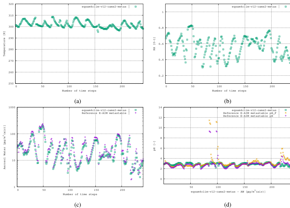
Figure 3. Second case study: Tianjin, China, 9–22 Aug 2015, 241 data points, using the aerosol system: Mg^{2+} , Ca^{2+} , K^+ , Na^+ , HCl+Cl^- , NH_3+NH_4^+ , HNO_3+NO_3^- , H_2SO_4+SO_4^{2-}+HSO_4^- .
