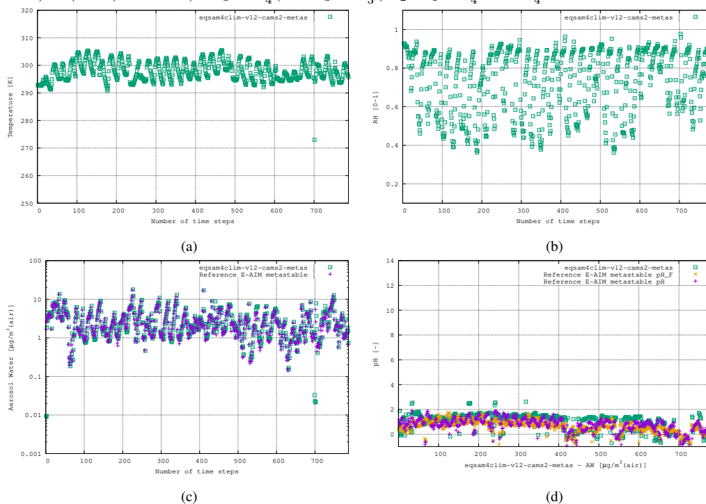
Figure 4. Third case study: SOAS campaign, Centreville, US, 6 Jun–14 Jul 2013, 787 data points, using the aerosol system: Na^+ , HCl+Cl^- , NH_3+NH_4^+ , HNO_3+NO_3^- , H_2SO_4+SO_4^{2-}+HSO_4^- .
