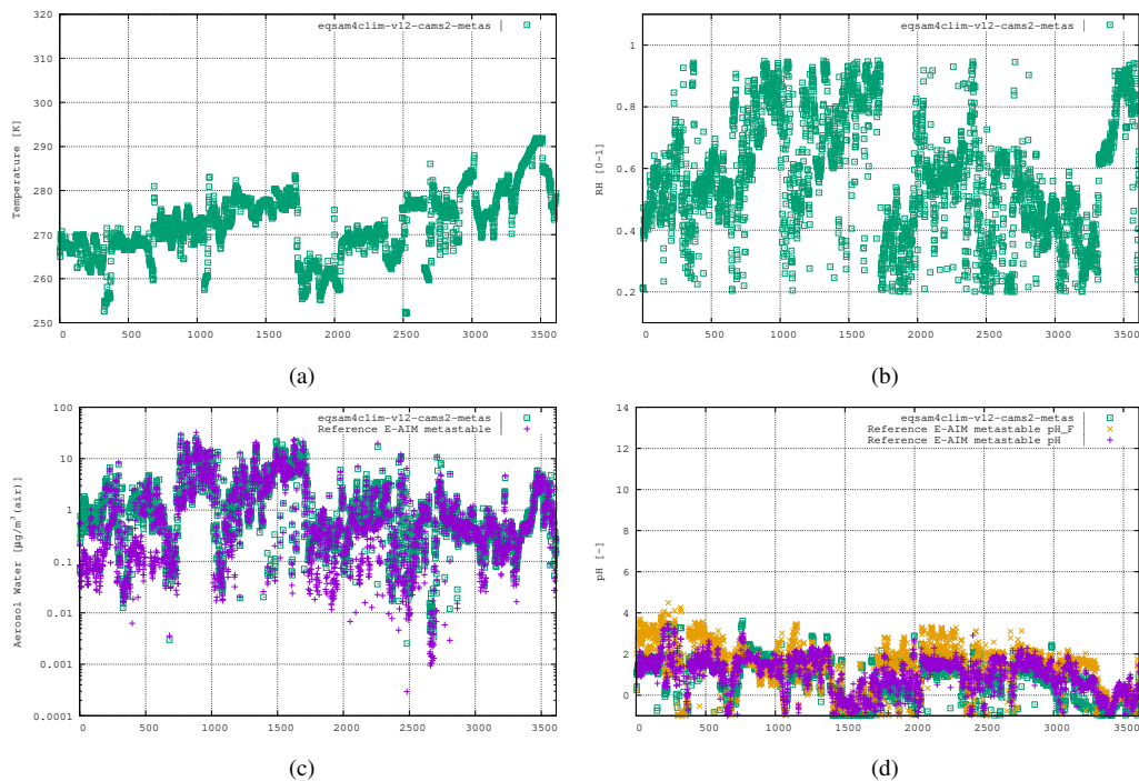
Figure 6. Fifth case study: WINTER campaign, Eastern US aloft, 3 Feb 2015, 3613 data points (real time axis see Supplement), using the aerosol system: \text{HCl}+\text{Cl}^- , \text{NH}_3+\text{NH}_4^+ , \text{HNO}_3+\text{NO}_3^- , \text{H}_2\text{SO}_4+\text{SO}_4^{2-}+\text{HSO}_4^- .
