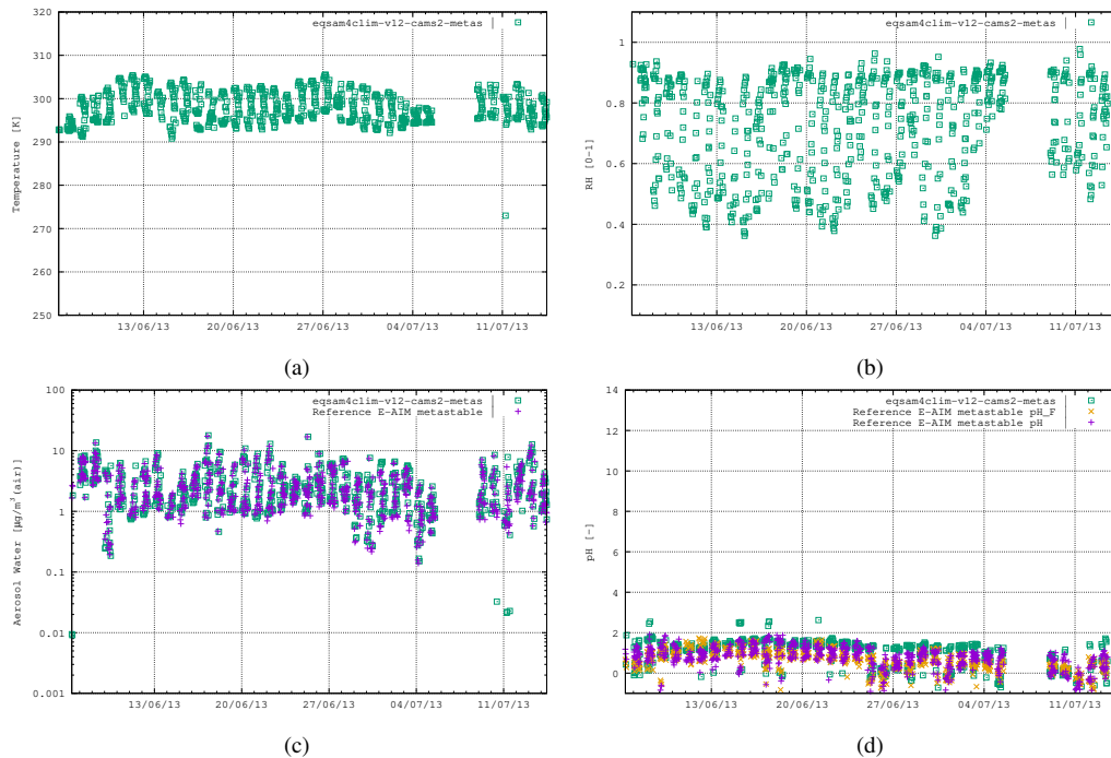
Figure 4. Third case study: SOAS campaign, Centerville, US, 6 Jun–14 Jul 2013 (787 data points), using the aerosol system: \text{Na}^+ , \text{HCl}+\text{Cl}^- , \text{NH}_3+\text{NH}_4^+ , \text{HNO}_3+\text{NO}_3^- , \text{H}_2\text{SO}_4+\text{SO}_4^{2-}+\text{HSO}_4^- .
