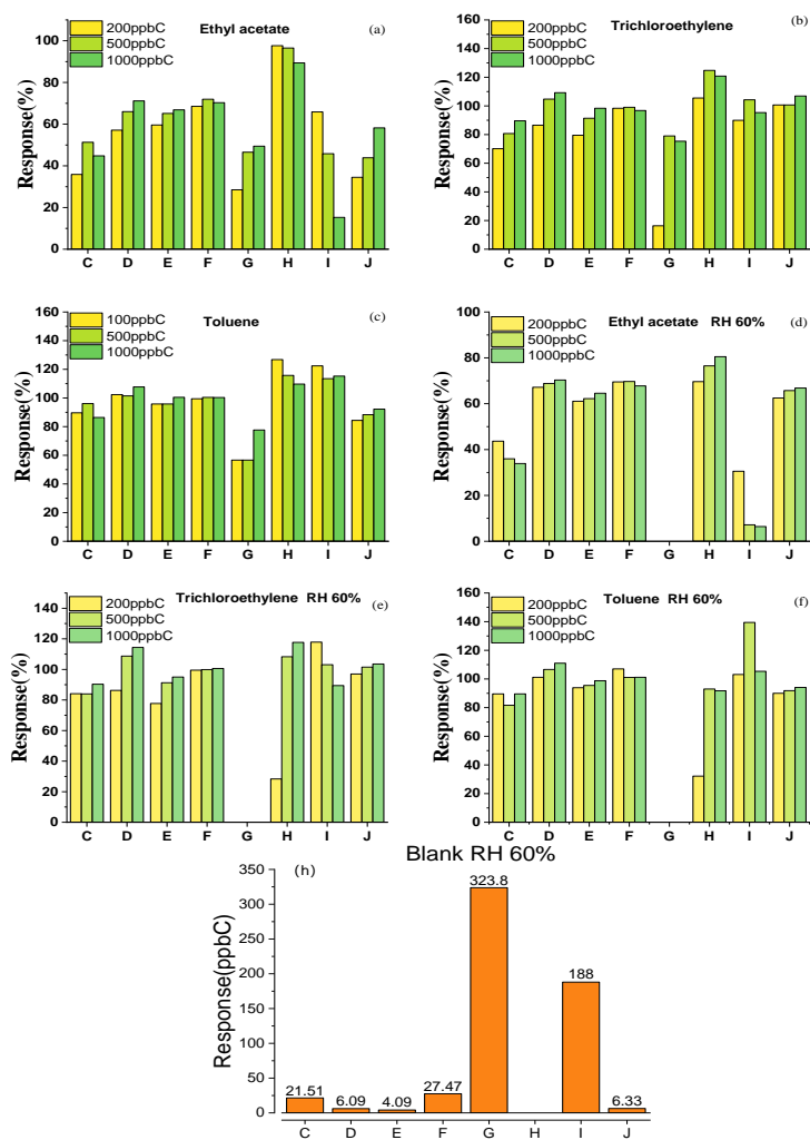
Figure 7: Response of different concentrations of (a-c) dry standard gas, (d-f) wet (RH 60%) standard gas, (h) wet blank (RH 60%) for C-J.
