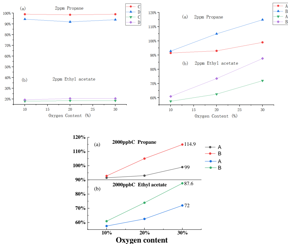
Figure 3: The effect of different oxygen contents on (a) propane and (b) ethyl acetate for A, B,C and D.
