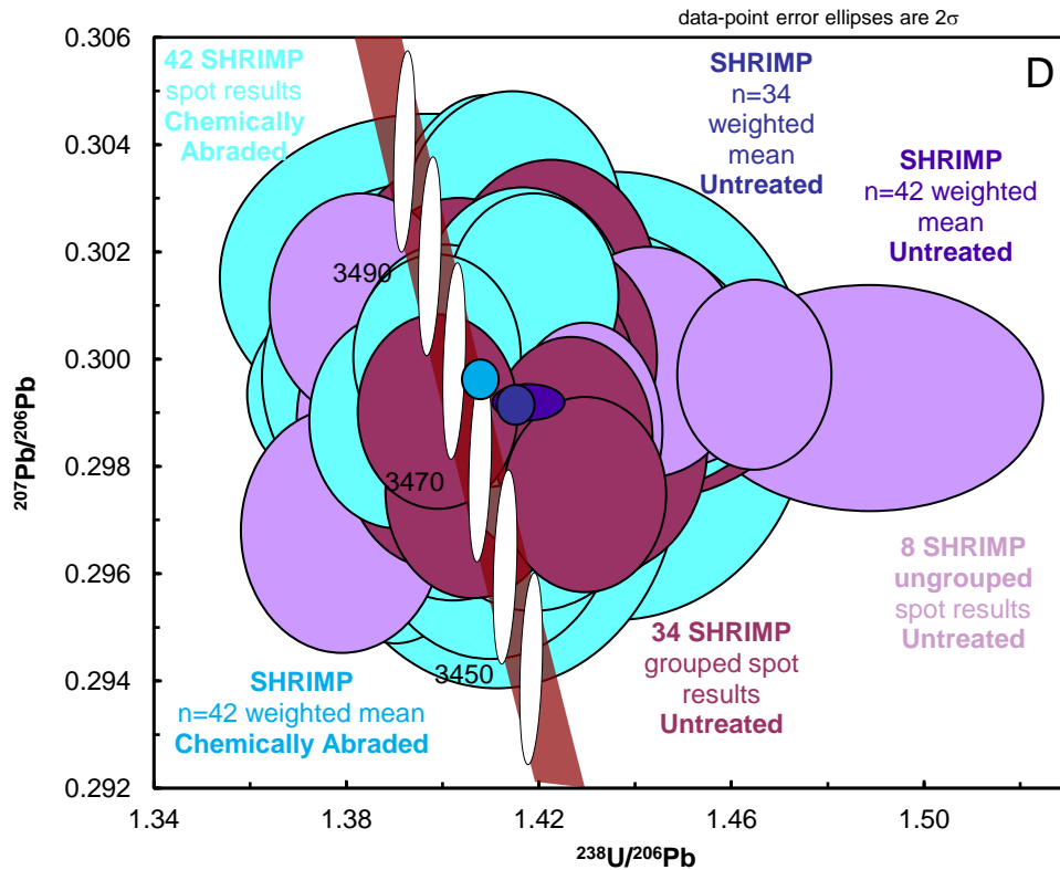
Figure 3: Tera-Wasserburg concordia diagrams for all individual SHRIMP spots, and means, on chemically abraded and untreated reference zircons. A: TEMORA-2. B: 91500. C: QGNG. D: OG1. Reference zircon is QNC for A, T2U for B,C,D.
