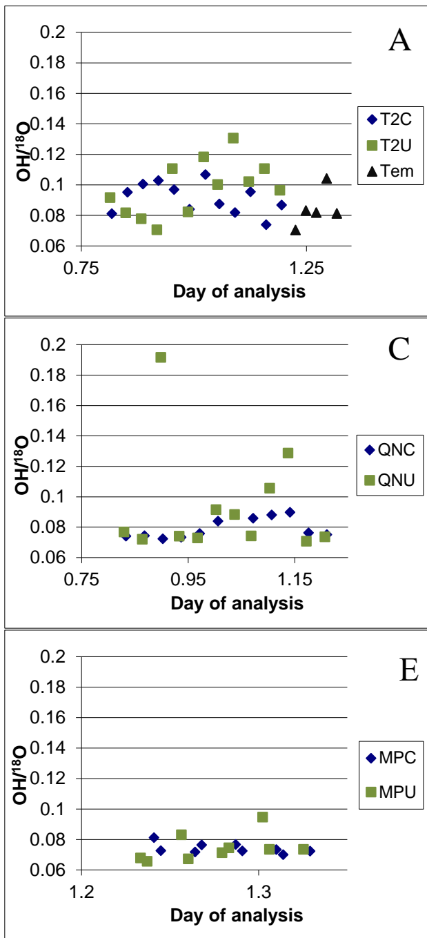
Figure 8. OH/ 18 O plots for various samples. All data have an epoxy degassing trend subtracted out. A: Untreated (green) and chemically abraded (blue) TEMORA-2. Black is untreated TEMORA-2 on the setup mount. B: Untreated (green) and chemically abraded (blue) 91500. Black is untreated TEMORA-2 on the setup mount. C: Untreated (green) and chemically abraded (blue) QGNG. D: Untreated (green) and chemically abraded (blue) OG1. E: Untreated (green) and chemically abraded (blue) Mount Painter Volcanic zircon rims.
