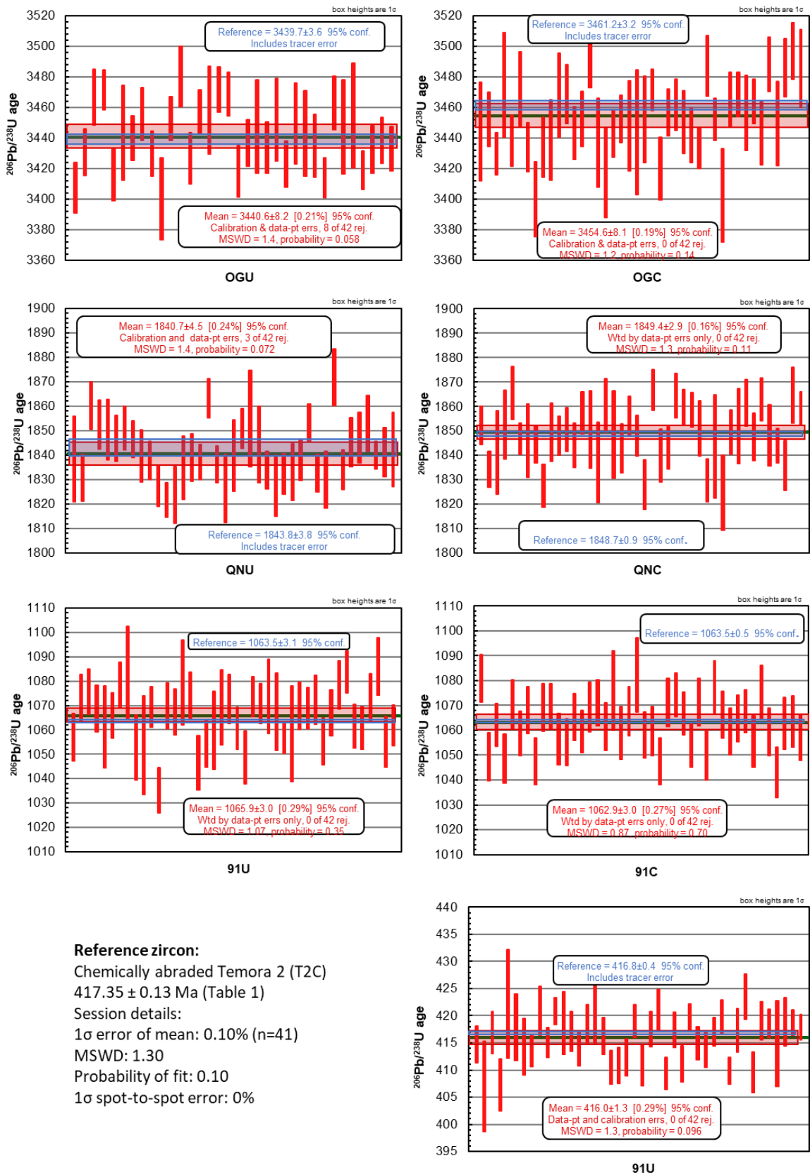
Figure 4: The values of SHRIMP data for OG1, QGNG, 91500, and T2U, referenced to T2C. SHRIMP data are in red, reference TMS ages are blue.
