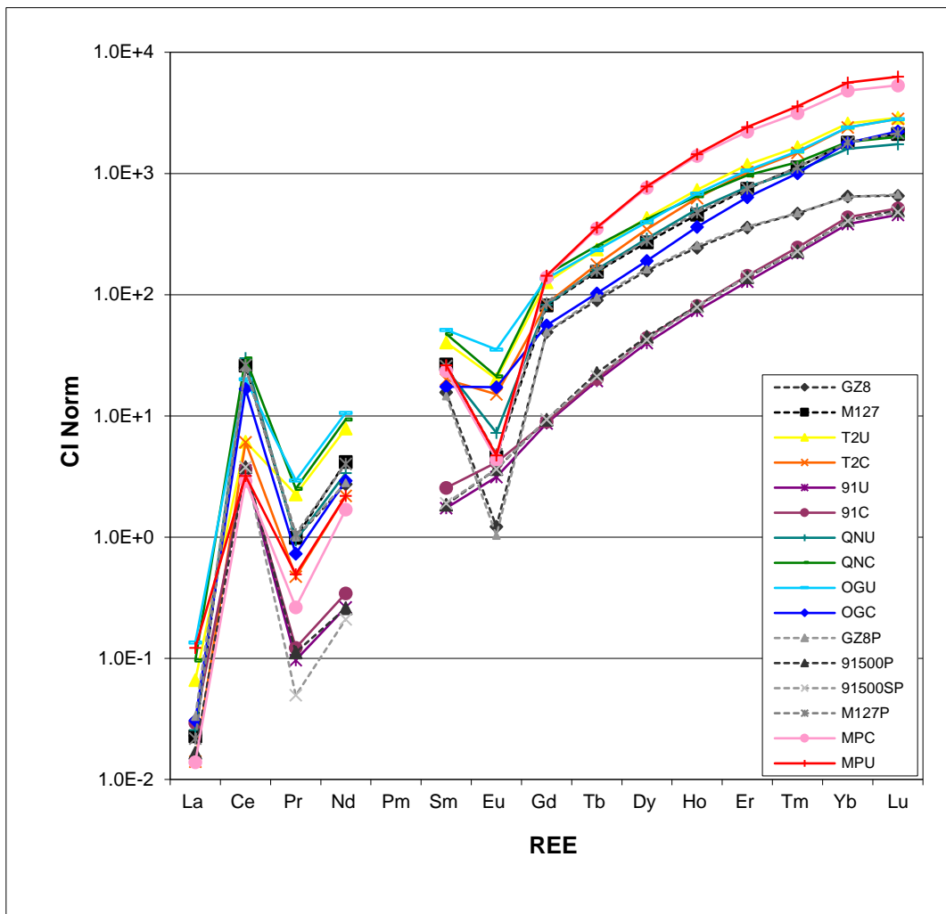
995 Figure 9. REE plots for the median REE content of the reference and Mt Painter zircons, normalized to chondritic abundances. Secondary (untreated) reference zircons G8 and M127 also shown. The Suffix 'P' indicates the secondary standard from the Mt Painter analytical session; The suffix 'SP' indicates 91500 grains from the setup mount run during the Mt Painter session. Secondary reference zircons have dotted lines, unknowns have solid lines.
