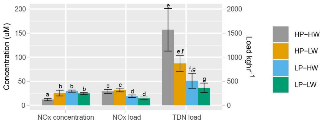
Figure 2. Average \text{NO}_x concentrations, \text{NO}_x loads, and average TDN loads on the day of maximum river discharge for each storm type. Letters indicate statistically significant differences between storm types.
