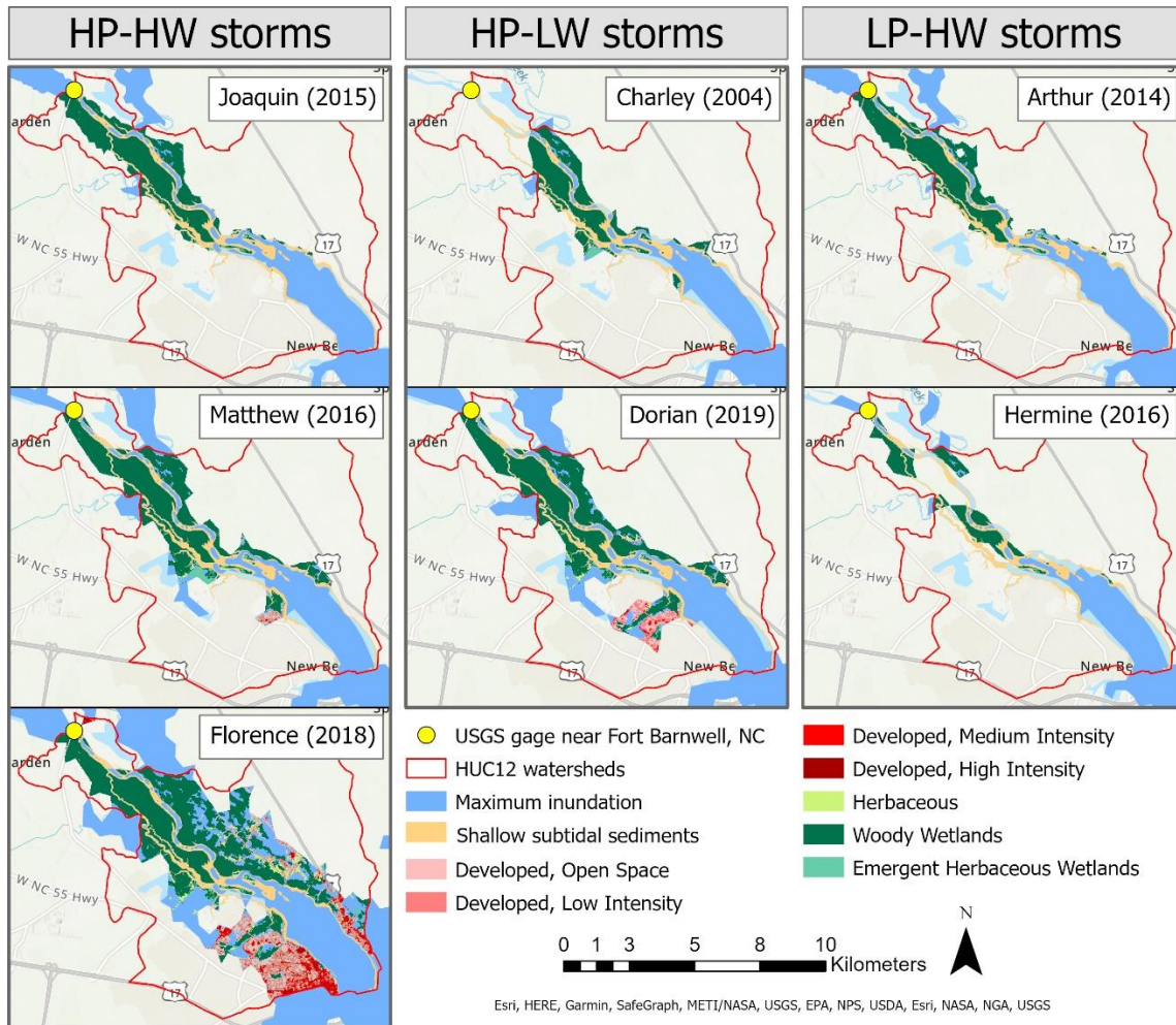
285 Figure 5. NLCD land cover classifications within HUC12 watershed boundaries and floodplain footprints for multiple storms affecting the Neuse River Estuary. Habitat treatments are derived from these land cover classifications.
