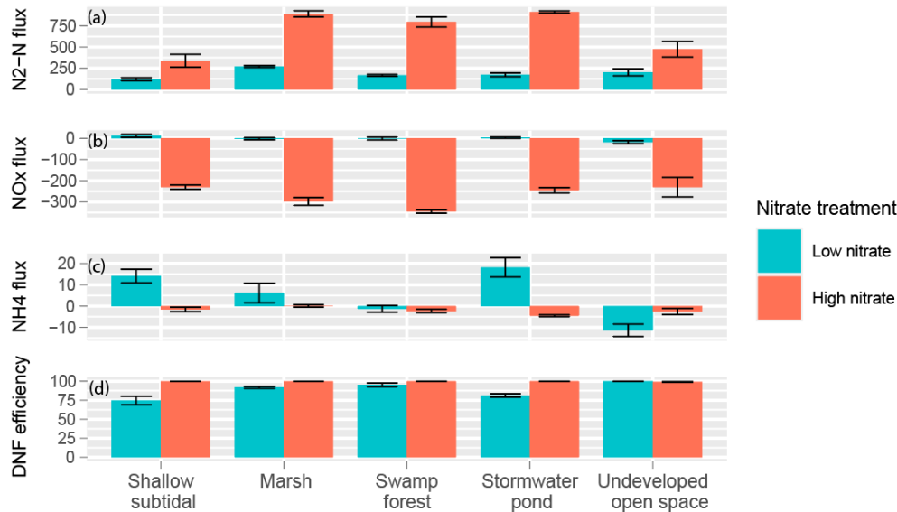
Figure 3. Fluxes ( \mu\text{mol m}^{-2} \text{h}^{-1} ) across the sediment water interface for multiple nitrogen species, including: (A) N_2 -N, (B) NO_x , and (C) NH_4 , as well as (D) DNF efficiencies (%). Positive fluxes indicate movement from the sediments to the overlying water column.
