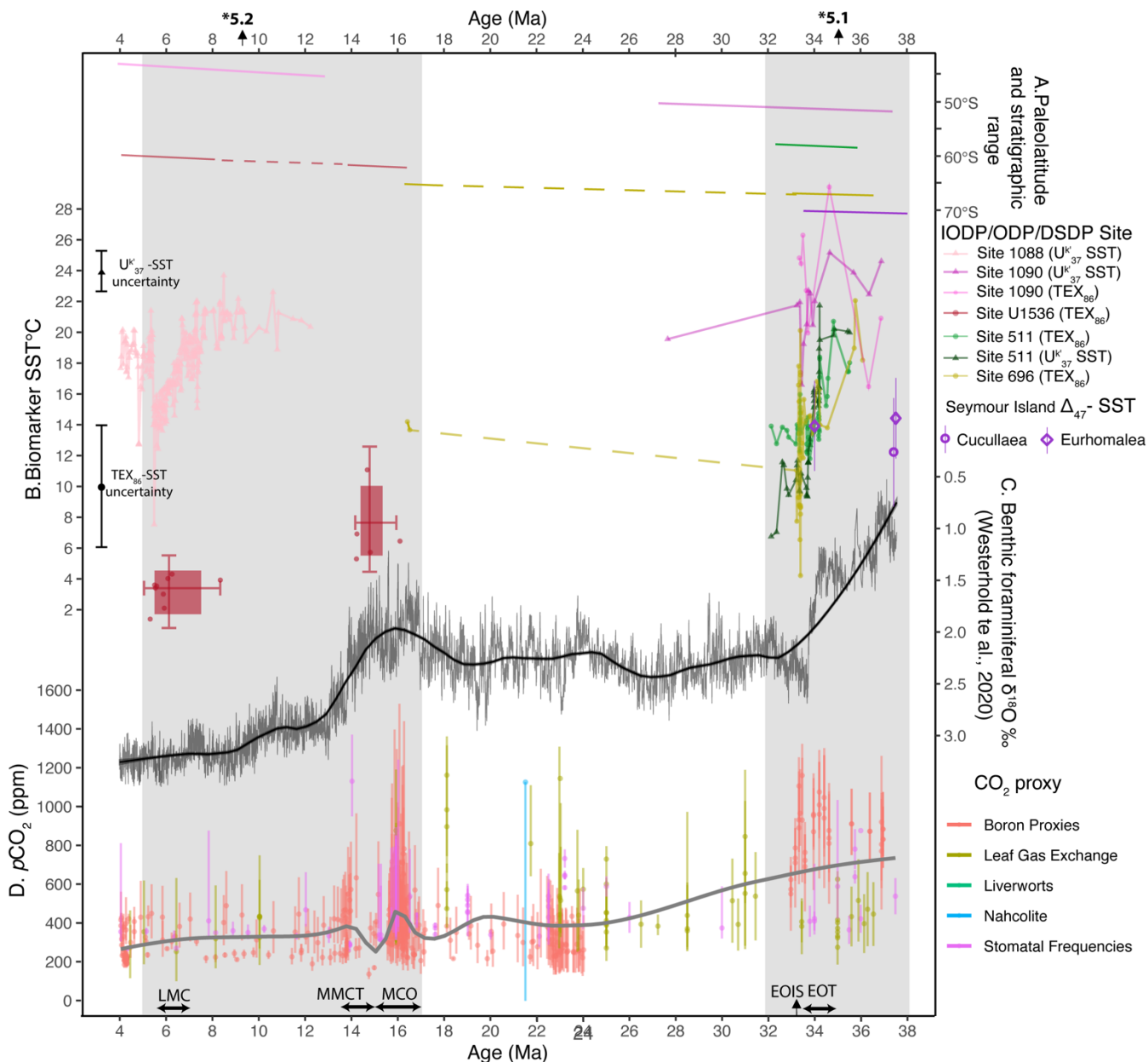
Figure 8. South Atlantic SST compilation A. Paleolatitude evolution of sites presented in this study (see legend; http://www.paleolatitute.org , version 2 by van Hinsbergen et al. (2015)). Stippled lines indicate hiatuses. B. The colored points and lines indicate the biomarker-based SSTs (see legend), excluding all samples with potential GDGT overprints (see Sect. 3.2). The bars on the left indicate the standard calibration error of the SST proxies. \text{TEX}_{86} -SST data from Site 696 (yellow; this study). \text{TEX}_{86} -SST data from Site 1090 (dark pink; Liu et al., 2009). \text{U}^{k'_{37}} - and \text{TEX}_{86} -SST from Site 511 (green; Houben et al., 2019). \text{U}^{k'_{37}} -SST from 1088 (pink; Herbert et al., 2016). \text{TEX}_{86} -SST from Site U1536 (red; this study). Clumped isotope ( \Delta_{47} ) SST estimates from La Meseta Fm., Seymour Island (purple; Douglas et al., 2014). C. Benthic foraminiferal \delta^{18}\text{O} compilation, with a locally weighted smooth over 20 kyr (black curve) (CENOGRID; Westerhold et al., 2020), and a LOESS smooth (blue; span = 0.2). D. Published paleo- \text{CO}_2 data from selected proxies named in legend ( https://www.paleo-co2.org ), with LOESS smooth (red; span = 0.3). LMC=Late Miocene
