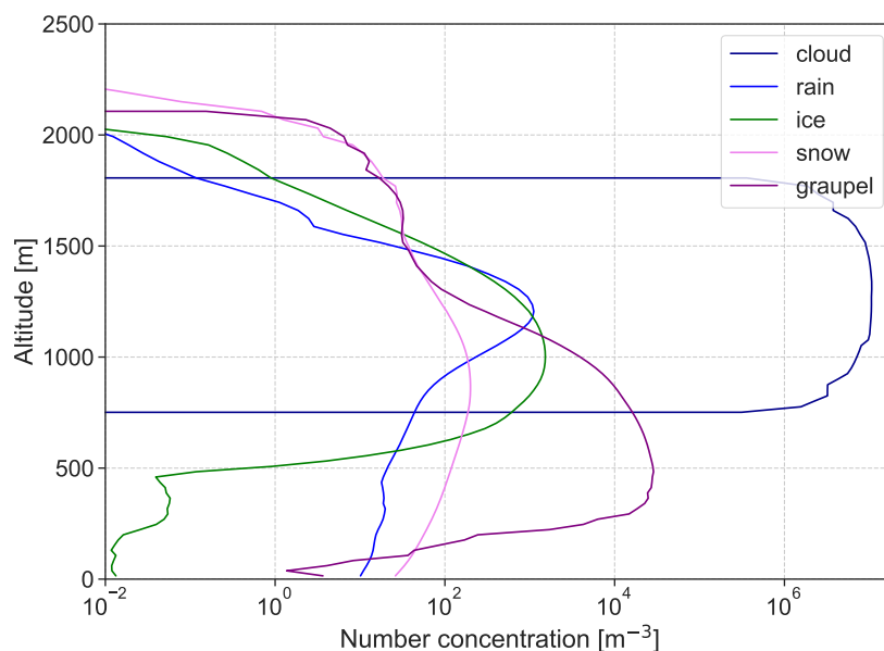
Figure 7. Number concentrations of individual hydrometeor categories in simulation MY_{\text{adap}} during the third flight.
