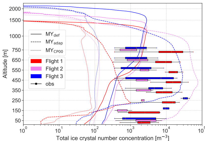
Figure B1. ICNC for the simulations MY_{def} , MY_{adap} and MY_{CP00} which is identical to MY_{adap} apart from the CCNC during updrafts: The ICNC is much lower when CCNC during updrafts is parametrized by Cohard and Pinty (2000) than when it is set to 9 \text{ cm}^{-3} .
