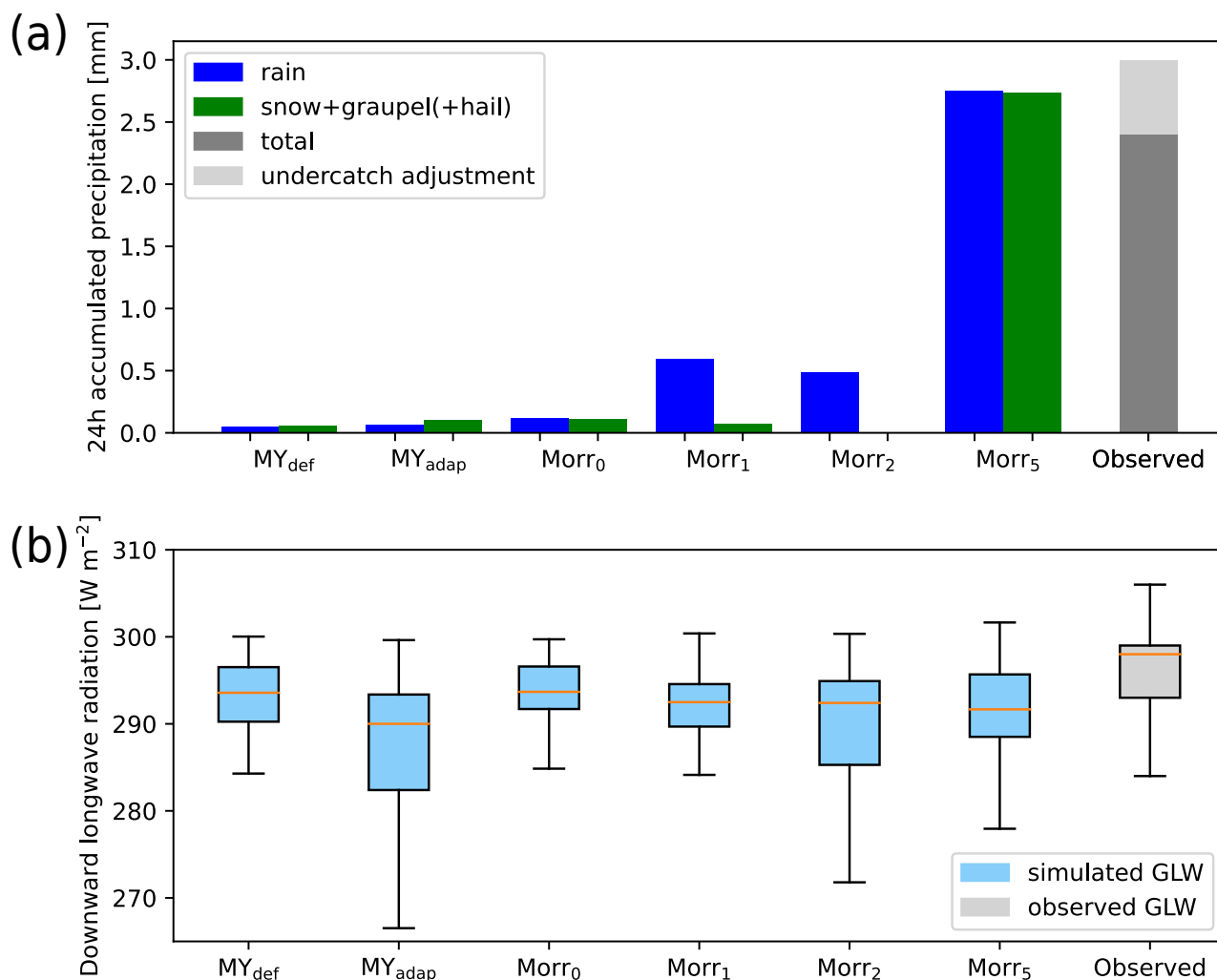
Figure 8. (a) Accumulated precipitation on 12 November, divided in liquid (blue) and frozen fraction (green) and (b) downward longwave radiation at the surface (GLW): Values are shown for the two simulations with the MY scheme, MY def and MY adap , selected simulations with the Morr scheme, and observations (total precipitation shown in grey). As the observed precipitation was measured using a single-fenced gauge, there is likely an under-catch in the amount. Here, we adjust for that by adding 24% following Kochendorfer et al. (2017) (see Sect. 3.2). In the radiation panel (b), the orange lines illustrate the median, the boxes extend from the first to the third quartile of the data and the whisker end points mark the farthest point inside 1.5-times the inter-quartile range from the box. The observed GLW was measured from the French-German AWIPEV Research Base (Maturilli, 2019).
