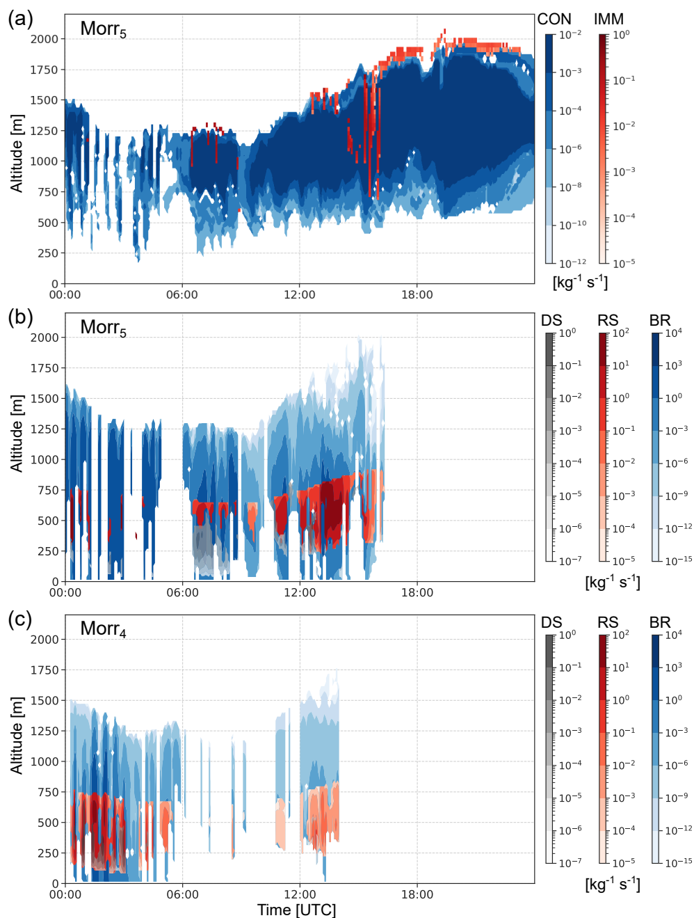
Figure 10. Ice crystal number concentration tendencies of (a) contact (CON, in blue) and immersion freezing (IMM, on top in red) and (b,c) collisional breakup (BR, in blue), rim splintering (RS, on top in red) and droplet shattering (DS, on top in grey): DS is shown partly transparent to visualize that BR is generally active simultaneously. The panels (a) and (b) show simulation Morr 5 while the lowermost panel (c) shows the SIP tendencies for simulation Morr 4 .
