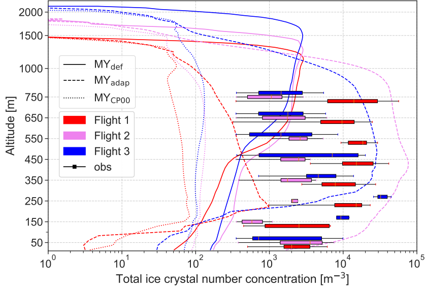
Figure B2. ICNC for the simulations MY_{\text{def}} , MY_{\text{adap}} and MY_{\text{CP00}} which is identical to MY_{\text{adap}} apart from the CCNC during updrafts: The ICNC is much lower when CCNC during updrafts is parametrized by Cohard and Pinty (2000) than when it is set to 9 \text{ cm}^{-3} .
