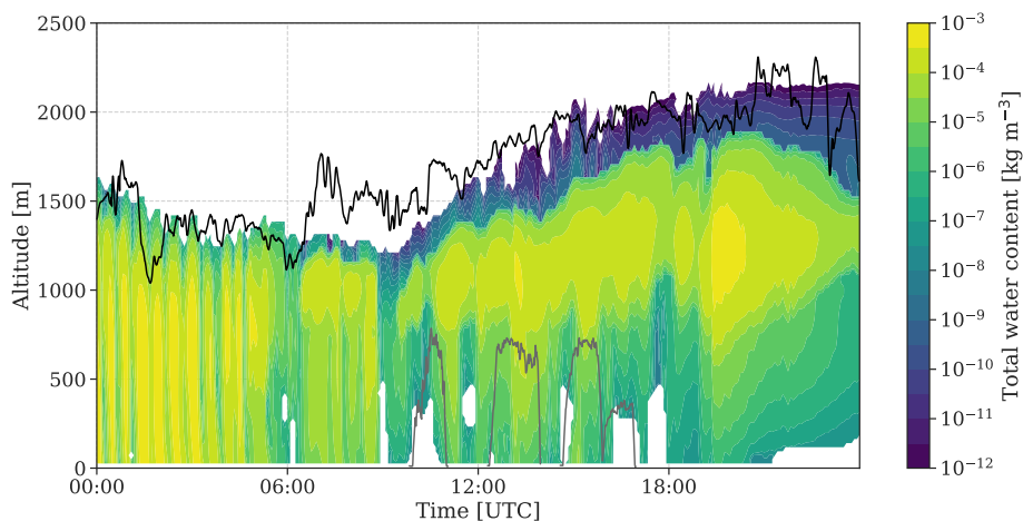
Figure 4. Total water content on 12 November as modeled by the final simulation \text{Morr}_5 . The macrophysical shape of the cloud agrees well with observations of radar reflectivity (see Pasquier et al. (2022b, Fig. 3c)). The black lines show the observed cloud top as retrieved from radar measurements (Ebell et al., 2022) while the three flights performed by HoloBalloon are shown as grey lines.
