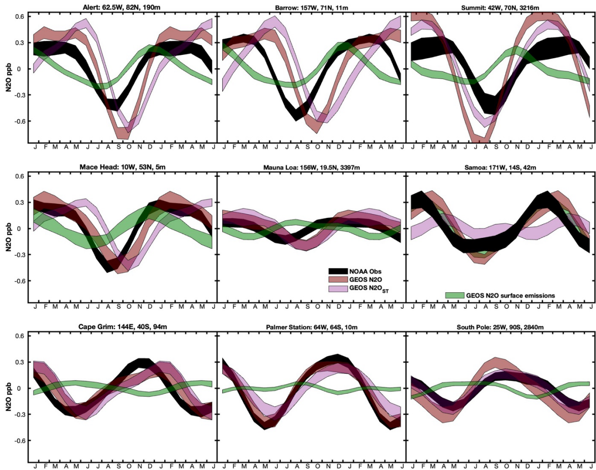
320 Figure 1: Detrended seasonal cycles in N_2O mixing ratio (ppb) modeled by GEOSCCM and compared to NOAA surface station data at 9 surface sites. Top row from left to right: Alert (Canada), Barrow (Alaska), Summit (Greenland); middle row from left to right: Mace Head (Ireland), Mauna Loa (Hawaii), Cape Matatula (Samoa); bottom row from left to right: Cape Grim (Tasmania), Palmer Station (Antarctica), South Pole (Antarctica). Black is observed N_2O from NOAA. For GEOSCCM, the total N_2O from all forcings is in red and the stratospheric tracer N_2O_{ST} is in magenta. Blue is N_2O due to fresh surface emissions, representing the combined net influence of the 325 natural soil, ocean, and anthropogenic atmospheric tracers.
