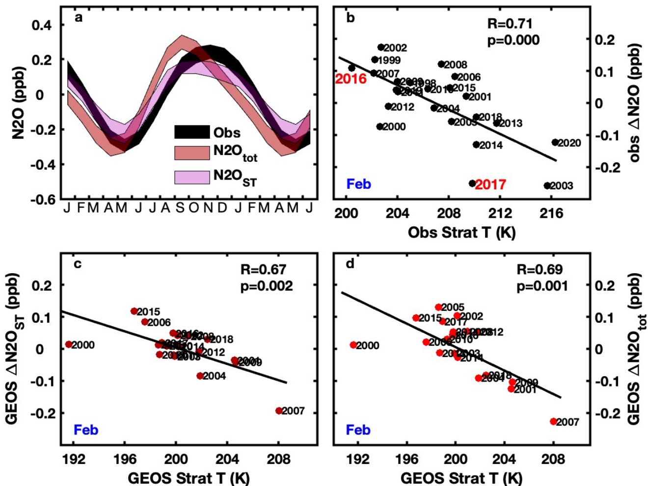
480 Figure 9: Top row shows a) mean seasonal cycles in N 2 O for NOAA surface station observations (Obs) and GEOSCCM surface 485 total N 2 O (N 2 O tot ) and stratospheric N 2 O (N 2 O ST ) and b) NOAA surface seasonal anomalies of N 2 O mixing ratio (ppb) in February at South Pole spanning 1998-2020, plotted vs. mean lower stratospheric MERRA-2 temperature at 100 hPa averaged over 60-90°S over the previous spring (September-November). The labeled anomalies in 2016 and 2017 correspond to the year of the ORCAS and ATom-2 aircraft surveys, respectively. Bottom row shows GEOSCCM surface seasonal anomalies of N 2 O mixing ratio (ppb) for c) N 2 O ST and d) N 2 O tot in February at South Pole spanning 2000-2019, plotted vs. mean GEOSCCM lower stratospheric temperature, which is sampled the same way as the MERRA-2 temperature.
