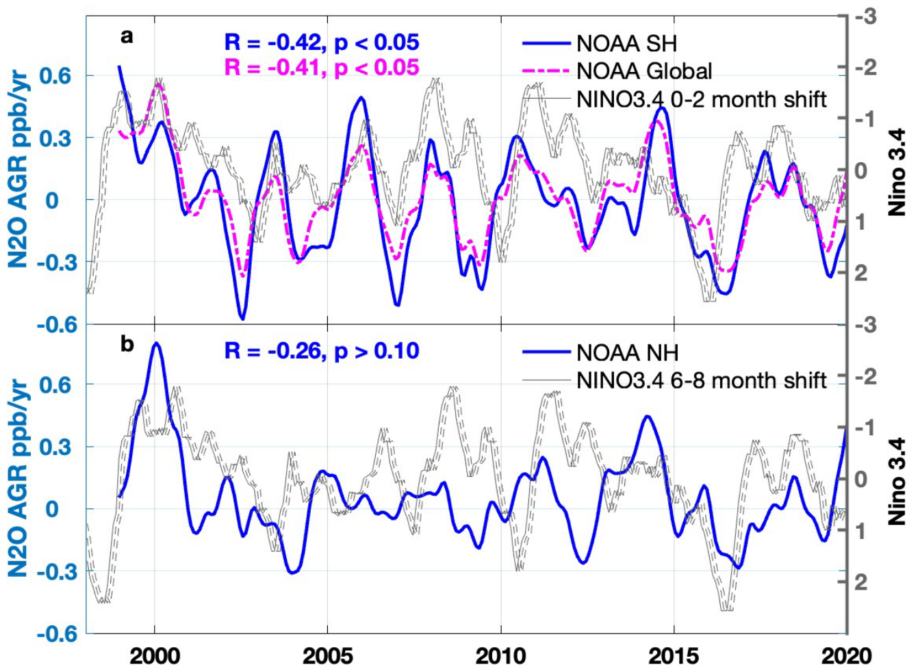
455 Figure 8: NOAA atmospheric growth rate (AGR in ppb/yr) plotted with the Niño 3.4 index for a) SH and global mean AGR with a 0-2 month shift in the index and b) NH AGR with a 6-8 month shift in the index.
