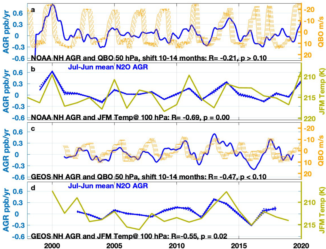
440 Figure 7: NH N_2O atmospheric growth rate (AGR in ppb/yr) for (a) NOAA and (c) GEOSCCM plotted with the QBO index at 50 hPa with a 10-14 month forward shift in the index. (b,d) NH N_2O AGR plotted with mean lower stratospheric temperature averaged over 60-90°N for January-March of the year labeled on the X axis. The AGR is averaged from monthly N_2O data over the encompassing 12 month period July-June (solid blue line), shifted plus or minus 1 month (dotted blue lines), for (b) NOAA and (d) GEOSCCM.
