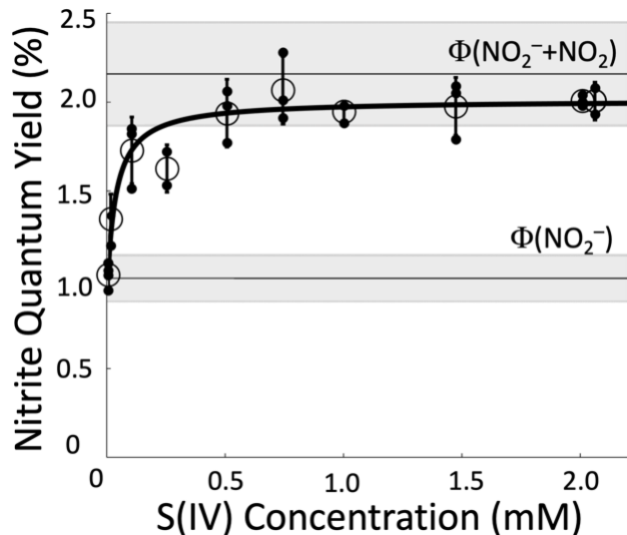
250 Figure 2. Measured apparent nitrite quantum yields for the photolysis of 50 \mu\text{M} nitrate solutions (293 K, pH 8) in the presence of different concentrations of S(IV). Hollow circles represent the average ( \pm 1 \sigma ) of individual experiments, which are shown as solid black points. The line through the data is a fit to equation 8. The lower grey area centered at 1.1% is the average of previously determined values of \phi(\text{NO}_2^-) \pm 1 \sigma , and the upper grey area centered at 2.2% is the sum of the quantum yields from both channels, \phi(\text{NO}_2^- + \text{NO}_2) \pm 1 \sigma , from the literature. 255 Literature values used to calculate these averages are in Table S1.
