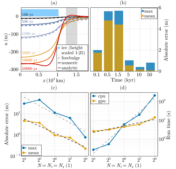
Figure 6. (a) Transient cross-sections of bedrock displacement along x -axis, from the center of the domain until x = 1800 km. The resolution used here is N_x = N_y = 2^8 , h \simeq 23 km. (b) Corresponding mean and maximal errors over time. (c) Resolution-dependence of maximum and mean error at equilibrium with respect to the analytical solution, with the light and dark grey dashed lines representing the corresponding linear regressions, respectively with slopes of -0.4 and -0.33 in \log_2 - \log_{10} space. (d) Resolution dependence of the computation time on CPU versus GPU, with the light and dark grey dashed lines representing the corresponding linear regressions, respectively with slopes of 0.73 and 0.17 in \log_2 - \log_{10} space.
