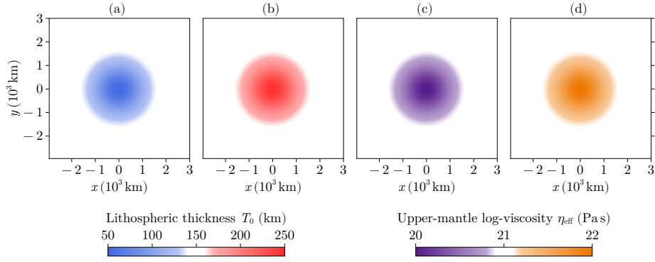
Figure D1. Gaussian-shaped LV used in Test 3 for (a) a lithospheric thinning, (b) a lithospheric thickening, (c) a viscosity decrease and (d) a viscosity increase towards the centre of the domain.
