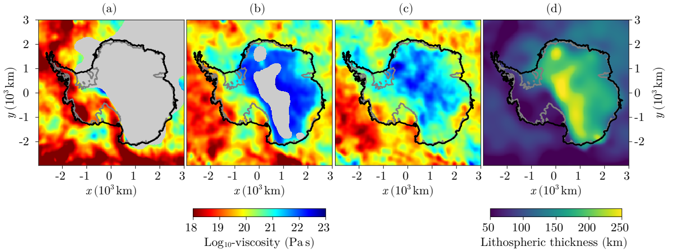
Figure 2. (a-c) Upper-mantle viscosity from Whitehouse et al. (2019) and Ivins et al. (2022) at 100, 200 and 300 km depth, respectively. If the lithospheric thickness (Pan et al., 2022), depicted in (d), is larger than the layer depth, a grey shading is applied. The black and dark grey contour lines respectively indicate the present-day ice-sheet and grounded ice margins (Morlighem et al., 2020).
