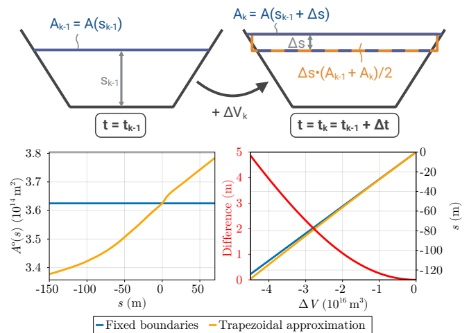
Figure 4. (Top) Schematic representation of the trapezoidal approximation used to solve the nonlinear dependence between BSL, s , and ocean surface, A . We hereby use A_k as shorthand for A(s_k) . (Bottom left) Present-day ocean surface and ocean-surface function, A(s) , as computed by the trapezoidal approximation of the basin evolution. (Bottom right) BSL computed for a change in ice volume equivalent to the LGM, for fixed boundaries compared to the trapezoidal approximation.
