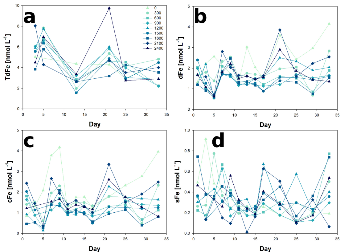
Figure 2. Temporal evolution of a) total dissolvable iron (TdFe), b) dissolved iron (dFe), c) colloidal iron ( c\text{Fe} = d\text{Fe} - s\text{Fe} ) and d) soluble iron (sFe) concentrations from day 0 to day 33 of the mesocosm experiment for the nine increased alkalinity mesocosms ranging from 0 (light blue) to 2400 \mu\text{mol L}^{-1} (dark blue). Symbols and color-codes as in figure 1C. The concentration range of the different size fractions is different. Three y-axis ranges have been used; up to 10 \text{ nmol L}^{-1} for TdFe, up to 5 \text{ nM} for dFe and cFe, and up to 1 \text{ nmol L}^{-1} for sFe.
