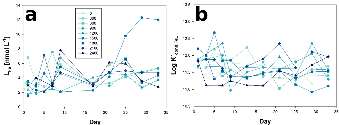
245 Figure 3. Temporal evolution of a) iron ligands ( L_{Fe} ), and b) Conditional constant ( K_{cond} ), from day 0 to day 33 of the mesocosm experiment for the nine increased alkalinity mesocosms ranging from 0 (light blue) to 2400 \mu\text{mol L}^{-1} (dark blue). Symbols and color-codes as in figure 1C.
