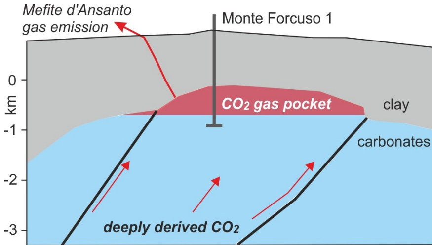
100 Figure 1. Section of the system feeding Mefite gas emission (redrawn with permission from Chiodini et al. (2010). Copyright 2010 by the American Geophysical Union. Geological section from Mostardini and Merlini (1986)).
