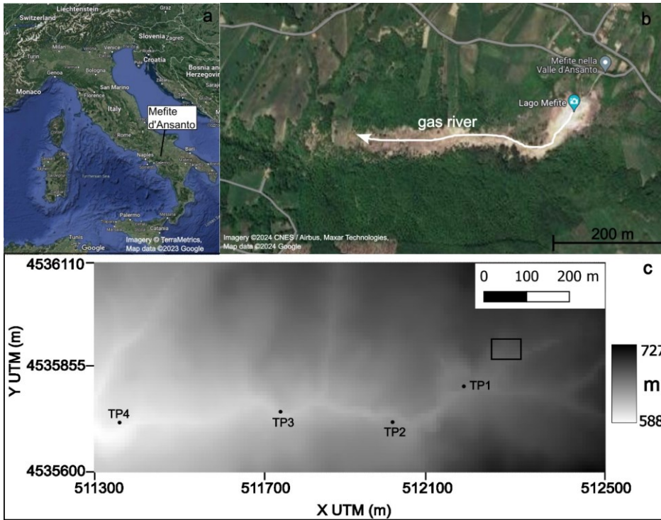
Figure 2: a) Location of Mefite d'Ansanto in Southern Italy. Imagery © TerraMetrics, Map data ©2023 Google. b) Aerial photo showing the gas emission area and the valley where the gas river forms, which is emphasized by the lack of vegetation. Imagery ©2024 CNES / Airbus, Maxar Technologies. Map data ©2024 Google. c) Computational domain with the elevation (m a.s.l.) shown in greyscale. The CO 2 emission area as approximated in the simulations is represented by the black rectangle. Black dots represent the locations of the four tracking points (TP) where the hazard curves are extrapolated from the simulation outputs; the coordinates of the tracking points are listed in Table 42.
