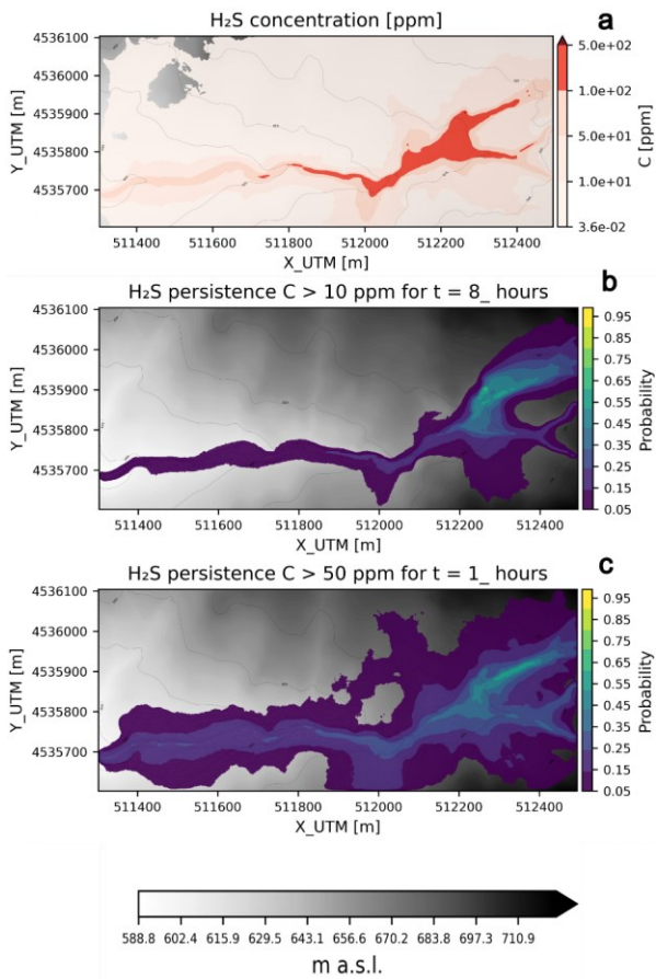
405 Figure 8. H 2 S probabilistic hazard maps at 2 m above the ground. a) 24 hours' time-averaged concentration at 5% exceedance probability. b) Persistence maps for PEL 10 ppm, exposure time = 8 hours. c) Persistence maps for PEL 50 ppm, exposure time = 1 hour.
