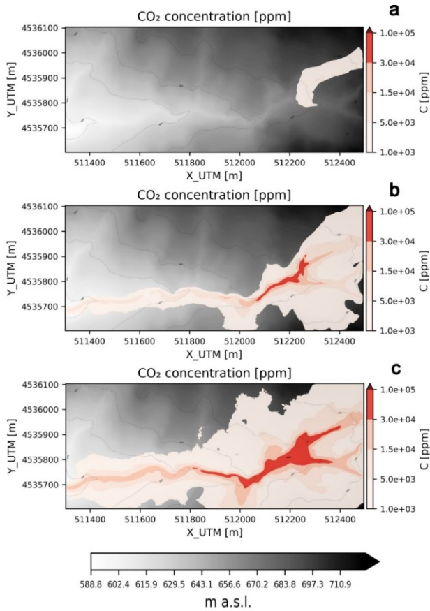
Figure 3. 24 hours time-averaged CO 2 concentration at 2 m above the ground at 50% (a), 16% (b) and 5% (c) exceedance probabilities
