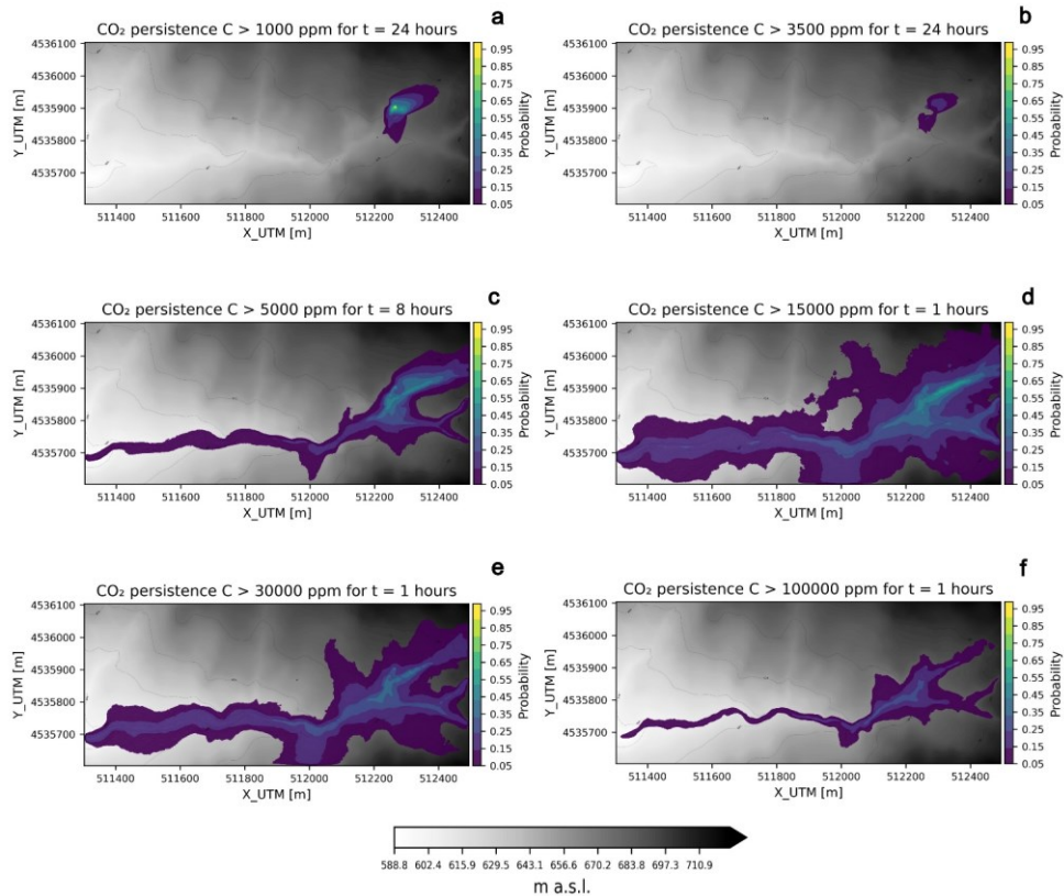
365 Figure 4. Persistence maps at 2 m above the ground. a) Concentration threshold = 1000 ppm, exposure time = 24 hours. b) Concentration threshold = 3500 ppm, exposure time = 24 hours. c) Concentration threshold = 5000 ppm, exposure time = 8 hours. d) Concentration threshold = 15000 ppm, exposure time = 1 hour. e) Concentration threshold = 30000 ppm, exposure time = 1 hour. f) Concentration threshold = 100000 ppm, exposure time = 1 hour.
