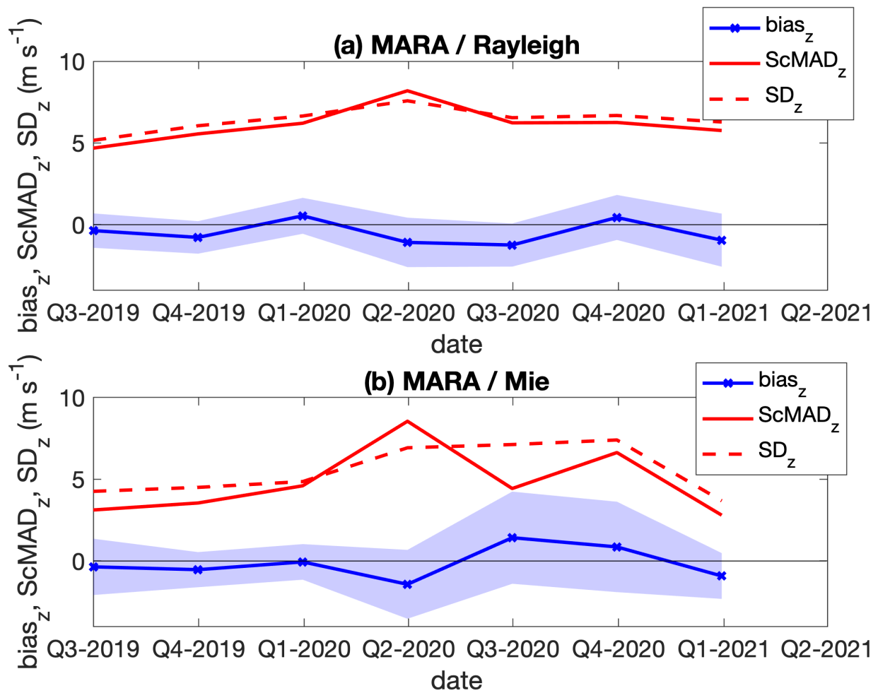
Fig 9. Variation over time of bias z , ScMAD z and SD z for the Aeolus-MARA comparison. The shaded area around bias z indicates 95% confidence limits. Each quarter (all seasons, all orbits) over the 2-year study period was processed separately. Insufficient data is available for the last quarter.
