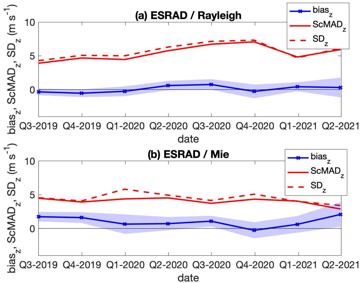
Fig 10. Variation over time of \text{bias}_z , \text{ScMAD}_z and \text{SD}_z for the Aeolus-ESRAD comparison. The shaded area around \text{bias}_z indicates 95% confidence limits. Each quarter (all seasons, all orbits) over the 2-year study period was processed separately.
