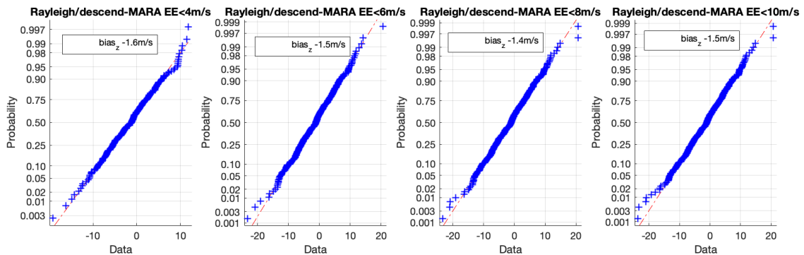
365 Figure 7: Normal probability plot for the difference between Aeolus Rayleigh HLOS wind and MARA wind (descending passes) for a series of EE thresholds, after rejecting points with ModZ > 3.5. See text for details.
