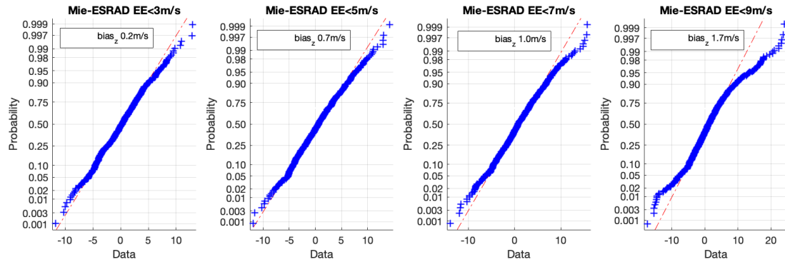
370 Figure 8: Normal probability plot for the difference between Aeolus Mie HLOS wind and ESRAD wind (all passes) for a series of EE thresholds, after rejecting points with \text{ModZ} > 3.5 . See text for details.
