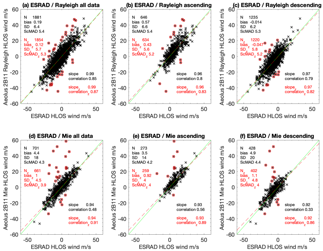
305 Figure 5: As Figure 3 but for ESRAD
