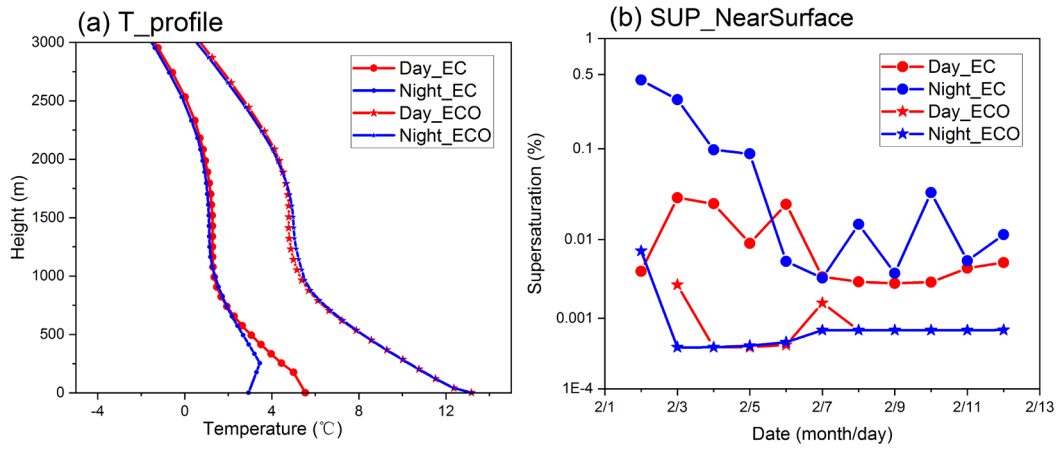
Figure S1. Diurnal variation of temperature profile (a, “Day” and “Night” refer to 7:00 to 18:00 and 19:00 to 06:00 of the next day in Beijing time respectively) and supersaturation (b)
