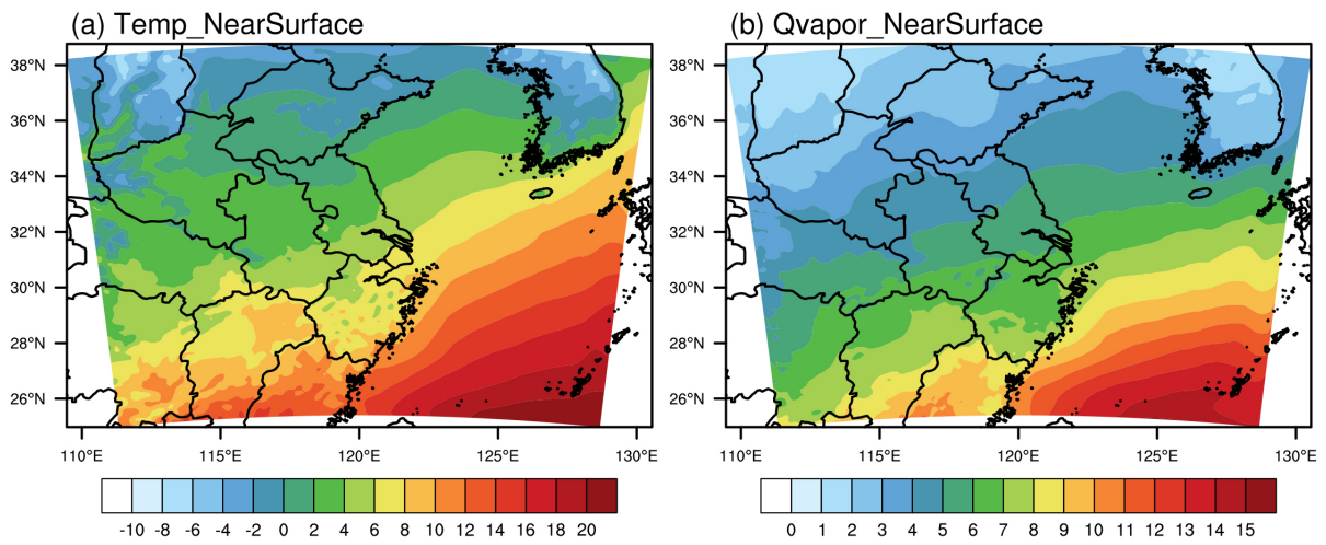
Figure S2. Distributions of near-surface average temperature (unit: °C, a) and water vapor content (unit: \text{g}\cdot\text{m}^{-3} , b)
