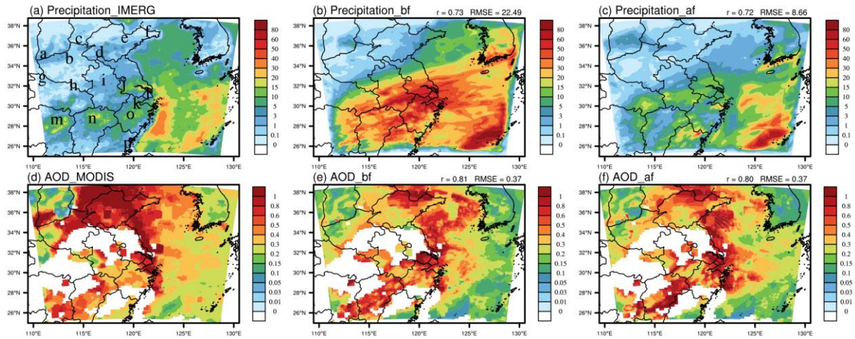
235 Figure 3. Distributions of accumulated precipitation (unit: mm, a-c) and average AOD (dimensionless, d-f) during the simulation period from the observation as well as before and after assimilation of the meteorological fields ( r and RMSE at the up-right corner represent the spatial correlation coefficient and root mean square error of the observed and the simulated, respectively, where RMSE is in the same unit as the variable in the figure. The subscripts "_bf" and "_af" in the subfigure 240 captions have the same meaning as in Fig. 2. The markers a-p in Fig. 3a represent the locations of the stations in Fig. 4)
