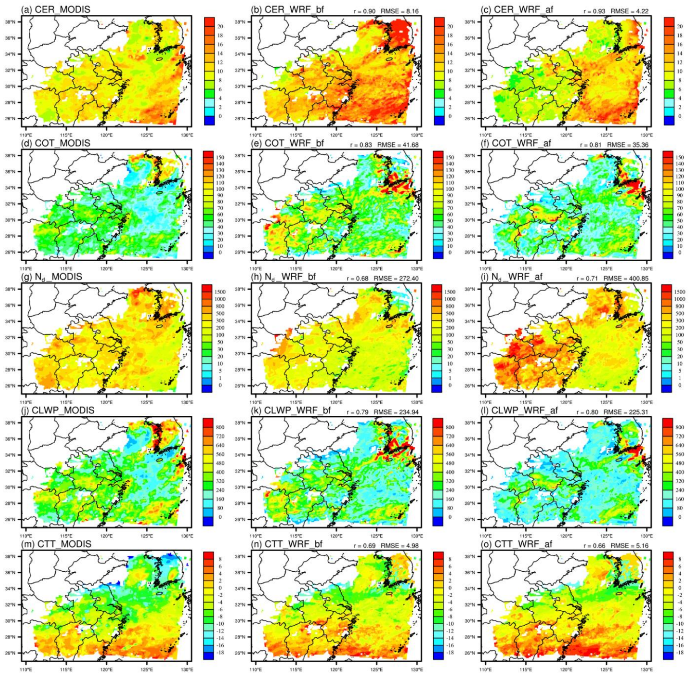
Figure 5. Spatial distribution of average CER (a-c, in \mu\text{m} ), COT (d-f, dimensionless), N_d (g-i, in \text{cm}^{-3} ), CLWP (j-l, in \text{g} \cdot \text{m}^{-2} ) and CTT (m-o, in ^{\circ}\text{C} ) from MODIS and WRF simulation before and after assimilations (The r and RMSE in the upper right corner and the subscripts "_bf" and "_af" in the subfigure captions have the same meaning as in the previous figure)
