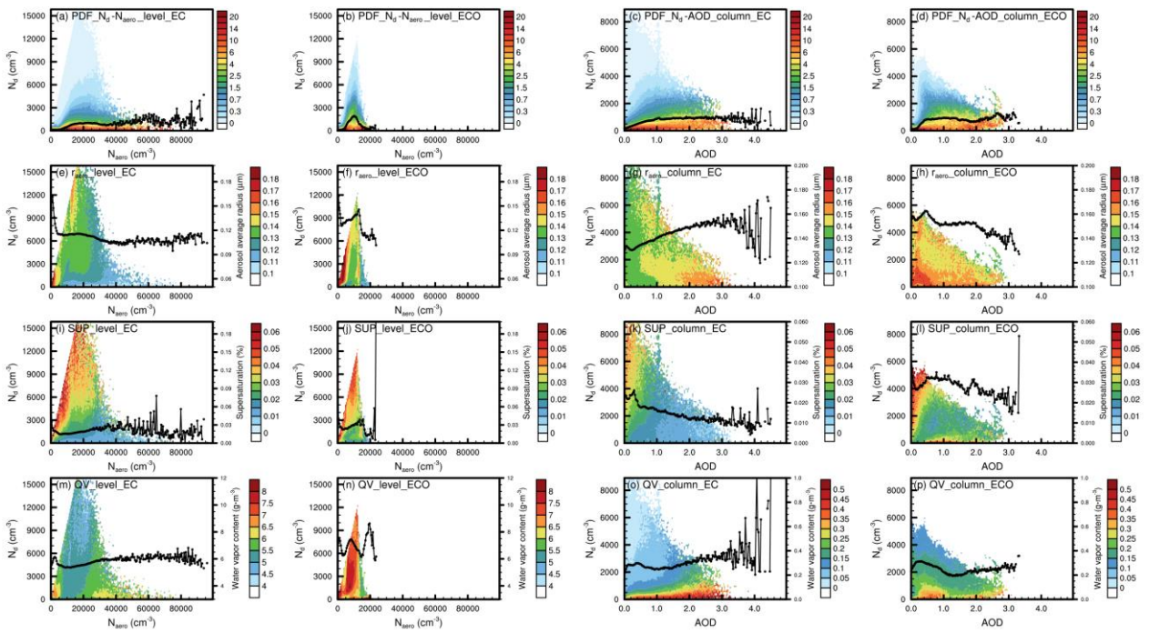
345 Figure 10. N_d varies with aerosol (a-d, the unit for colored dots is %, while the unit for the black lines is the left vertical axis unit), as well as the aerosol volume average radius (e-h, the colored dots and black lines of these figures and all subsequent figures correspond to the units on the right vertical axis unit), supersaturation (i-l) and water vapor content (m-p) varies with N_d and aerosol in EC and ECO based on statistics at each vertical layer (two columns on the left) and column (two columns on the right), respectively (samples were taken from each time and each grid point, and each sample contained N_{aero} or AOD, N_d , aerosol volume mean radius, supersaturation, and water vapor content values. These samples were placed into 200 aerosol \times 100 N_d bins according to the interval in which their N_{aero} or AOD values and N_d values were located. The colored dots in Figs. a-d represent the proportion of that bin's sample number to the total number of samples of the 100 bins corresponding to the N_{aero} or AOD interval, i.e., the total value of all colored dots corresponding to each N_{aero} or AOD interval is 100%. The black lines in Figs. a-d represent the average N_d of all samples at the corresponding N_{aero} or AOD intervals. The colored dots in Figs. e-p represent the average values of the variable for all samples in the bin corresponding to the aerosol and N_d intervals. The black lines in Figs. e-p represent the average value of this variable in all samples corresponding to this aerosol interval) 350 355
