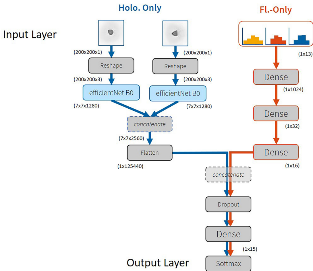
105 Figure S5: Machine learning model architecture for the study, where numbers indicate the previous layer's output dimensions. Three different model architectures are used with this existing structure. The left path ("Holo.-Only", colored blue) uses only the two holographic images as input. The right path ("FI.-Only", colored red) uses only the relative fluorescence spectra, here depicted as a plot of relative intensities. The third model combines both the two holographic images and the relative fluorescence spectra, which are concatenated together. The output layer is the Softmax prediction probability output, which classifies particle type by taking the maximum of this output. Here, as an example, the holographic image inputs and relative fluorescence spectra plot represent a single hazel pollen event.
