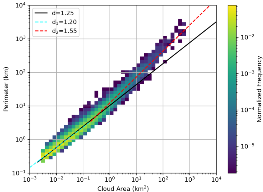
290 Figure 5: Density plot of cloud area against cloud perimeter using 50 logarithmic bins from 0.1 to 10000 km in the y-axis and 0.001 to 10000 km 2 in the x-axis for clouds larger than 12 pixels in the 170 ASTER scenes during the CAMP 2 Ex period with fractal dimension d without a scale break and d_1 and d_2 with a scale break.
