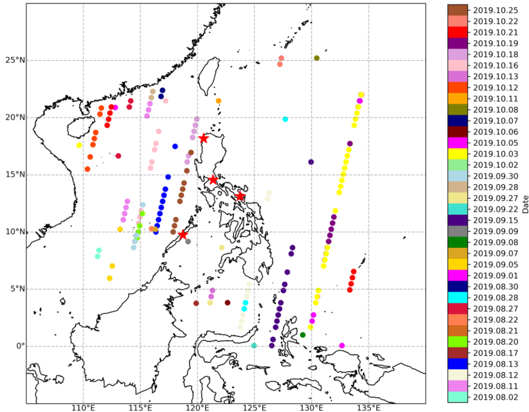
165 Figure 2: The center of each ASTER 60 km x 60 km scene used in the CAMP 2 Ex region, colored by date (YYYY.MM.DD). Red stars indicate operational sounding stations published by the University of Wyoming ( https://weather.uwyo.edu/upperair/sounding.html ).
