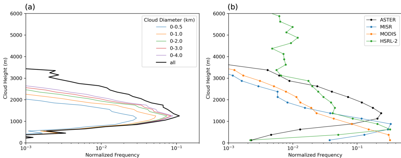
355 Figure 7: (a) Normalized distribution of cloud top heights with 100 m bin width from ASTER for different cloud equivalent diameters and (b) a comparison of the normalized distribution of cloud top heights with 250 m bin width obtained from ASTER, MISR, and MODIS corresponding to each ASTER scene and from the HSRL-2 onboard the P-3 aircraft.
