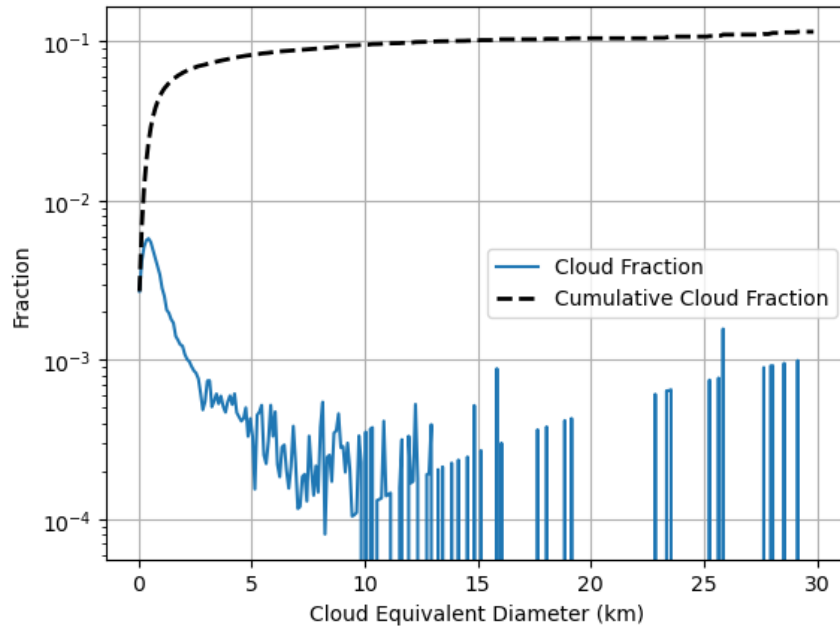
245 Figure 4: Cloud fraction and cumulative cloud fraction as a function of cloud equivalent diameter using bin width of 100 m for 170 ASTER scenes sampled over the western Pacific Ocean during CAMP 2 Ex.
