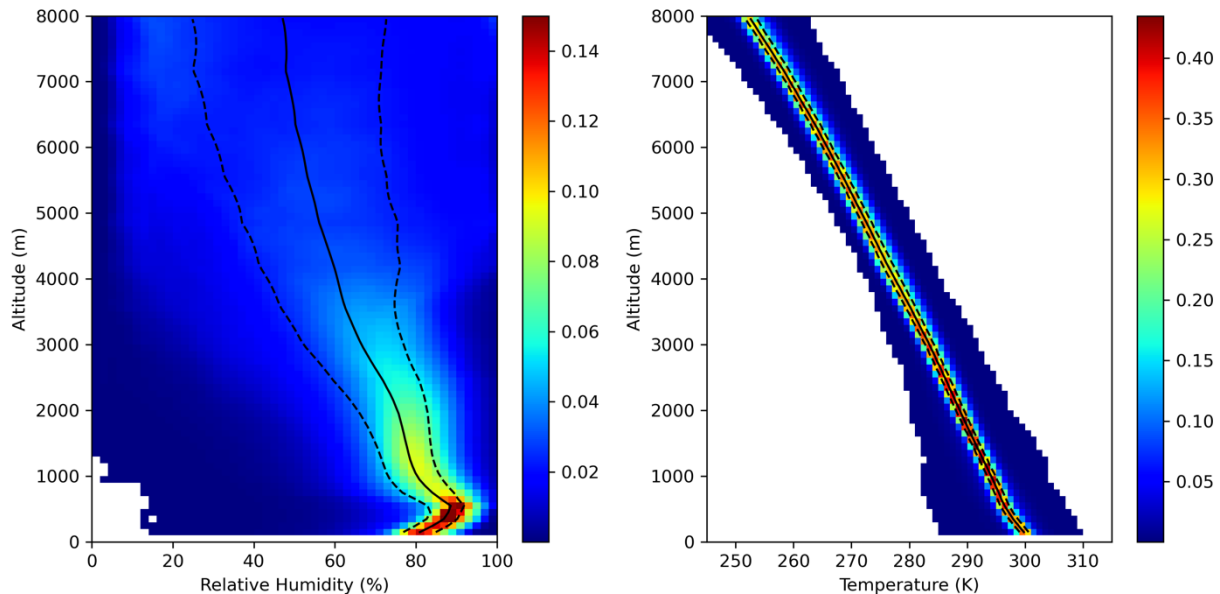
485 Figure 9: Contour frequency by altitude diagrams for relative humidity (left) and temperature (right) from the ERA5 reanalysis data. Relative humidity bins are 2 %, temperature bins are 1 K, and altitude bins are 100 m. The median is shown in the solid black line, while the 25 th percentile and 75 th percentile are shown in dotted black lines.
