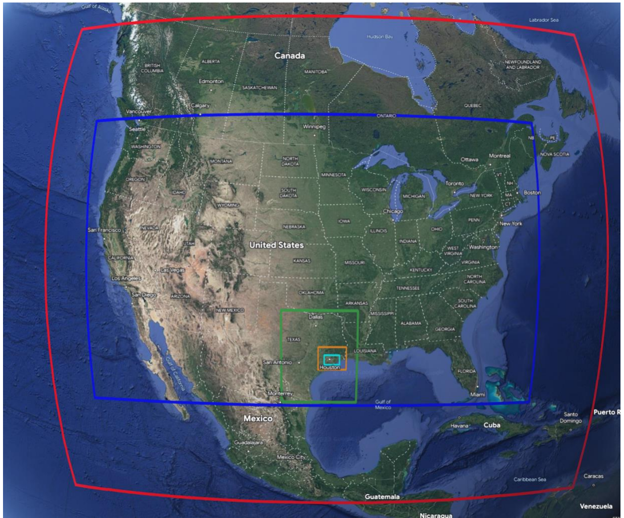
Figure 1: Modeling domains used in the CAMx simulation for the 36 km resolution (red), 12 km resolution (blue), 4 km resolution (green), 1.333 km resolution (orange), and the 0.444 km resolution (cyan). Maps data provided by Google © 2020, Landsat / CopernicusData SIO, NOAA, U.S. Navy, NGA, GEBCO, IBCAO, INEGI, and U.S. Geological Survey.
