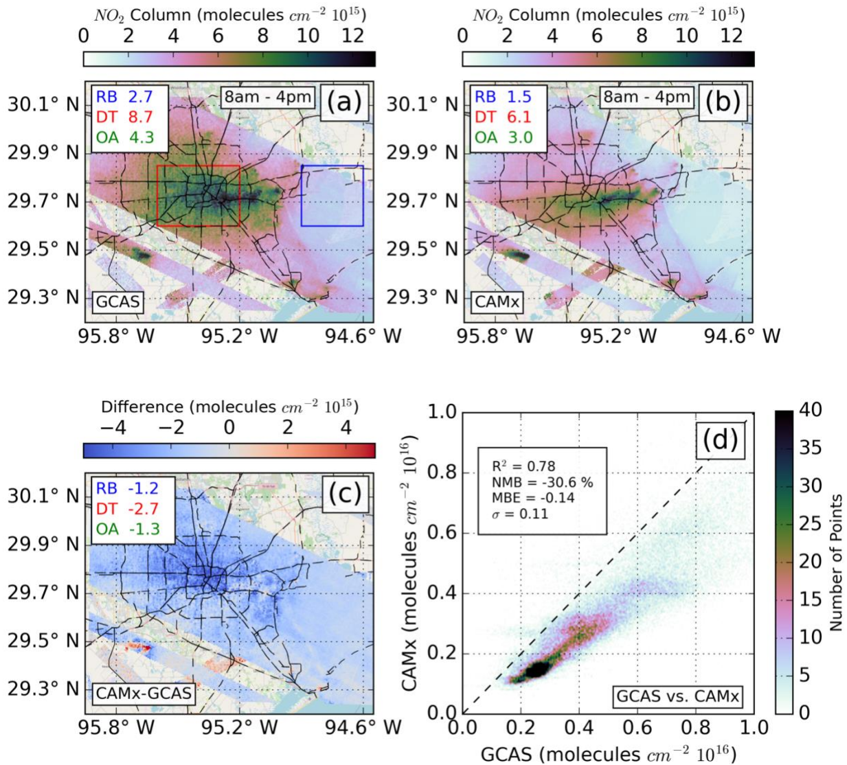
480 Figure 4: Comparison of GCAS observations to CAMx simulated NO 2 columns across all data during GCAS overpasses (generally 8 am – 4 pm). Temporally averaged GCAS NO 2 columns (A), temporally averaged simulated CAMx NO 2 columns (B), the absolute difference between GCAS and CAMx (C), and a scatter density plot comparing all observations between GCAS and CAMx (D). We identify three distinct areas: downtown or “DT” (red), the low emissions East Galveston rural Bay or “RB” (blue), and all other areas or 485 “OA” (green) and calculate the averages in the top left of each chart. © OpenStreetMap contributors 2023. Distributed under the Open Data Commons Open Database License (ODbL) v1.0.
