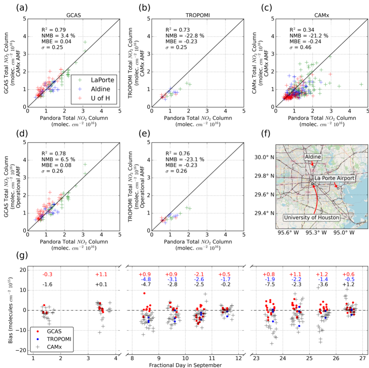
375 Figure 2: Comparison of Pandora total column NO 2 to GCAS using CAMx-based AMFs (A), TROPOMI v2.4.0 using CAMx-based AMFs (B), and CAMx (C) and GCAS (D) and TROPOMI v2.4.0 (E) with their operational AMFs. Tropospheric columns from GCAS and CAMx are bias corrected with a TROPOMI-derived stratospheric column factor as discussed in the methodology. Data from all possible overpasses
