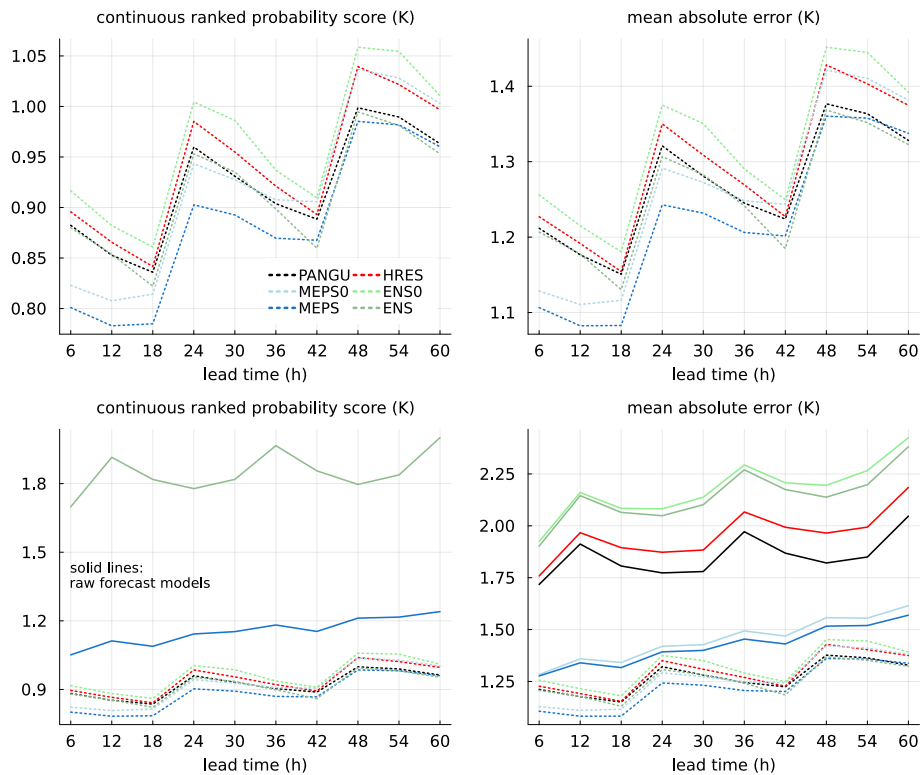
Figure 3. Continuous ranked probability score and mean absolute error for temperature at 2 meter as a function of lead time. In upper row scores for BQN calibrated forecasts only ( dotted lines ). In lower row raw forecast models ( dashed-solid lines ) are added for comparison.
