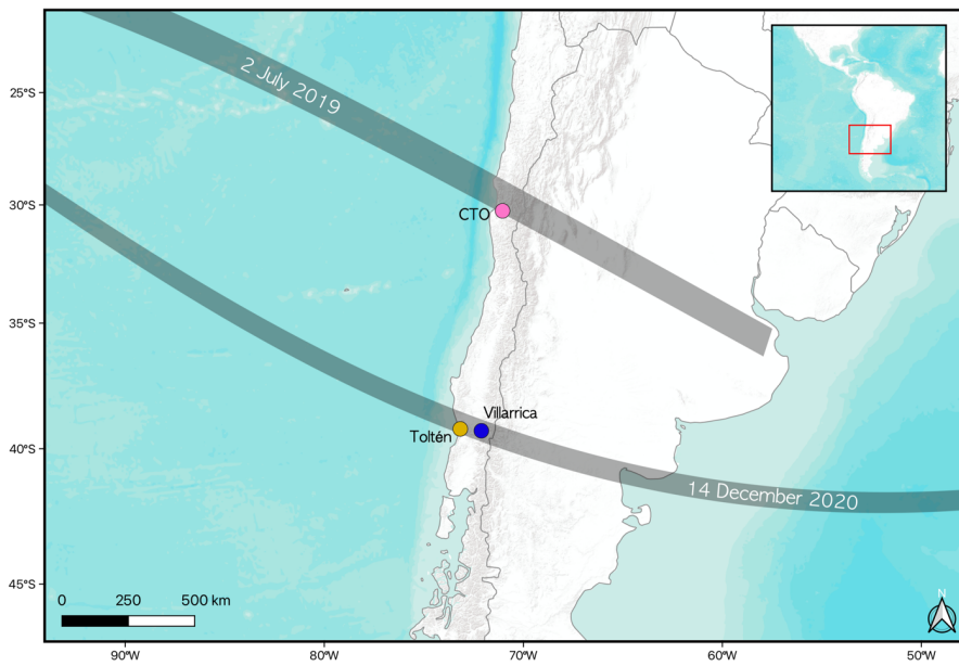
580 Figure 1: Map of eclipse totality paths (grey shaded areas) for the 2 July 2019 and 14 December 2020 TSEs. The 2019 launch 585 site at Colowara Tourism Observatory (CTO; pink point) and 2020 launch sites, Toltén (yellow point) and Villarrica (blue 590 point) are shown. Map created by Carl Spangrude using QGIS software ver. 3.22.0. Eclipse paths courtesy of Xavier M. Jubier ( xjubier.free.fr/en/site_pages/SolarEclipsesGoogleEarth.html ).
