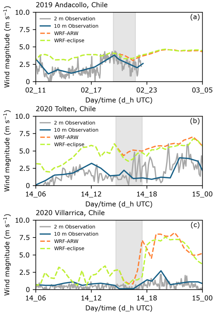
Figure 4: Comparison of wind speed (m s -1 ) observations at 2 m (solid grey lines), observations at 10 m (solid blue lines), and modeled results at 10 m for the 2 July 2019 eclipse (a) and from two sites (Toltén (b); Villarrica (c)) during the 14 December 2020 eclipse. Modeled results include WRF simulations with the eclipse enabled (dashed green lines) and disabled (dashed orange lines). Surface station observations are 3 min averages. Times of the eclipses are marked by the shaded grey area. Surface measurements from Andacollo, Chile in 2019 concluded at 22:30:00 UTC. Prior to the eclipse, WRF-ARW results are masked by WRF-eclipse results since both were identical until C1.
