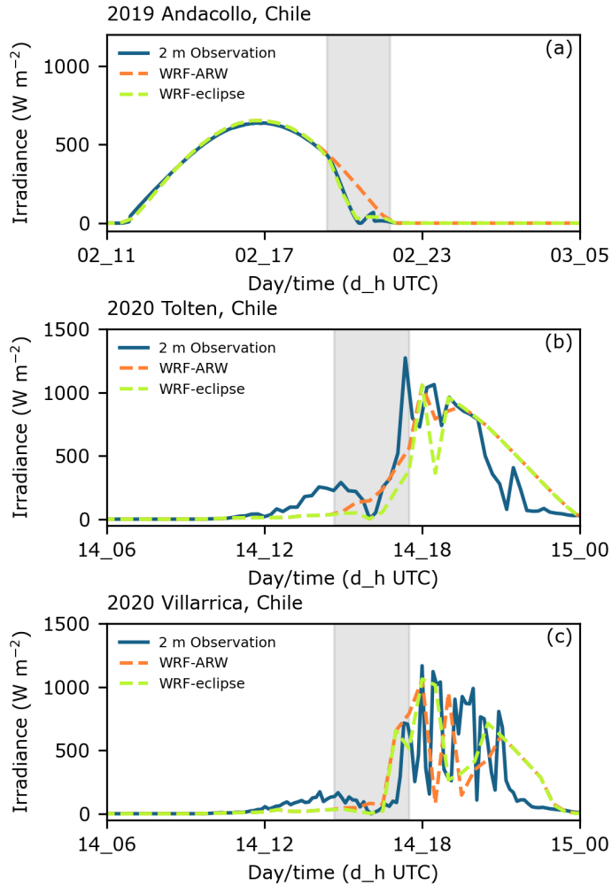
Figure 2: Comparison of irradiance ( \text{W m}^{-2} ) observations (solid blue lines) and modeled results at the surface for the 2 July 2019 eclipse (a) and from two sites (Toltén (b); Villarrica (c)) during the 14 December 2020 eclipse. Modeled results include WRF simulations with the eclipse enabled (dashed green lines) and disabled (dashed orange lines). Times of the eclipses are marked by the shaded grey area. Surface measurements from Andacollo, Chile in 2019 concluded at 22:30:00 UTC. Prior to the eclipse, WRF-ARW results are masked by WRF-eclipse results since both were identical until C1.
