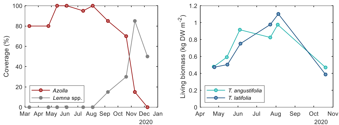
835 Figure A1 Coverage of Azolla and Lemna spp. (left) and estimated living biomass based on stem count and stem height in the chamber plots for Typha (right) for measuring year 2020.
