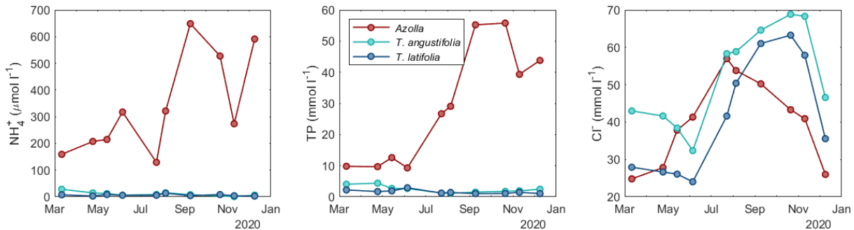
365 Figure 6 Pore water chemistry of ammonium ( \text{NH}_4^+ ), total phosphorus (TP), and chloride ( \text{Cl}^- ) measured in the soil of the different compartments of the three paludicrops at different moments in time.
