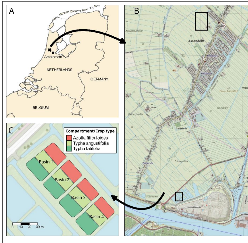
135 Figure 1 A) Overview of the research area located in the Netherlands (source map: SPOTinfo), with in B) the paludiculture location in the small lower square and the reference drained fen grassland in the big upper square (source map: GADM). C) Measurements for this research were conducted in Basin 2. The other basins were used to test treatments that are not discussed in this paper.
