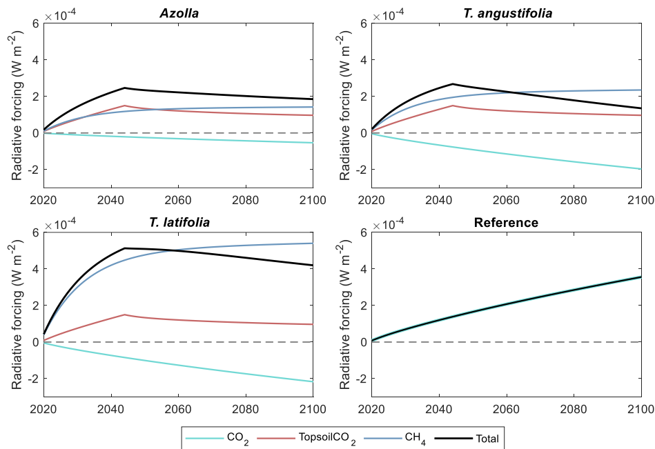
Figure 10 Contribution of paludicrops and reference site to radiative forcing for CO 2 flux (NEE + yield), estimated CO 2 emission from topsoil removal, and CH 4 emission. The topsoil is assumed to be completely decomposed within 257 years. The radiative forcing is calculated for a land surface area of 220,000 ha, which is the area of drained arable peatlands in the Netherlands.
