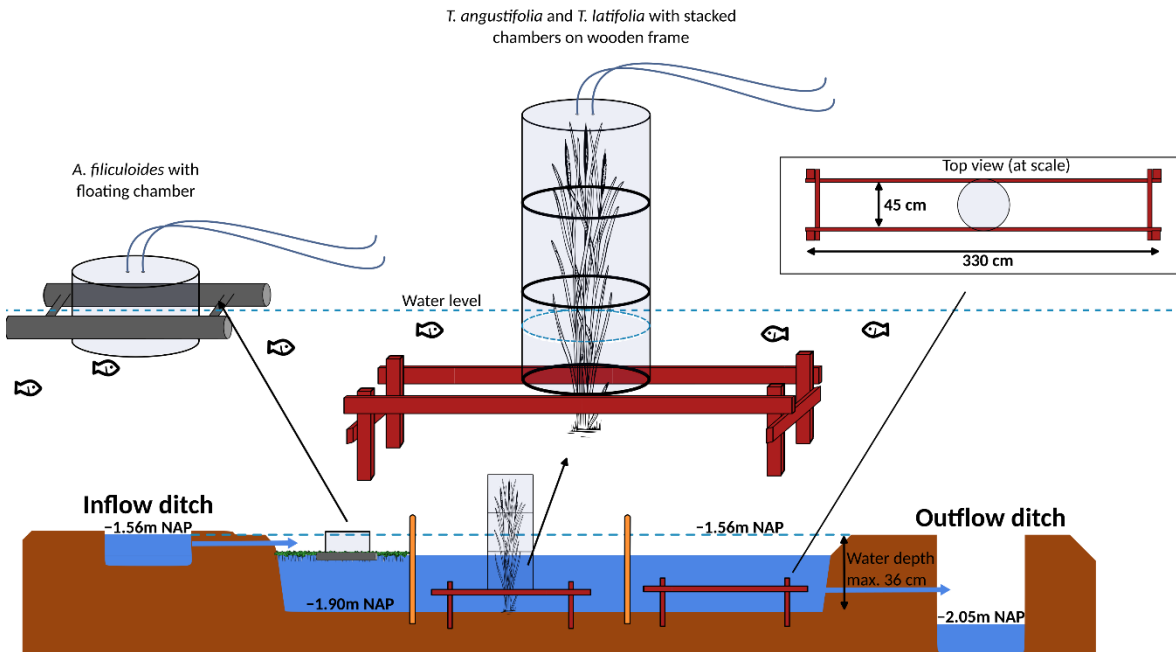
140 Figure 2 Set-up greenhouse gas flux measurement in experimental basin. With on the left the overview for Azolla and in the middle and right for Typha angustifolia and Typha latifolia , respectively. Water tables are relative to Amsterdam Ordnance Datum (NAP).
