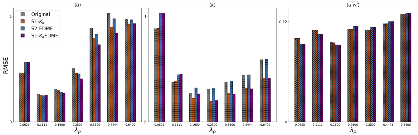
Figure 10. RMSE for four different scenarios of the 1D model from Table 2 against LES across seven densities in combination with seven height configurations from Table 1. Each column shows the lumped RMSE across seven different configurations.
