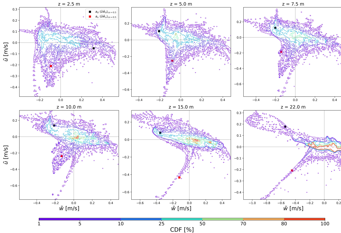
Figure 5. 2D CDF of the dispersive velocities at 2.5, 5, 7.5, 10, 15, and 22 m. The integral of the PDF within the area is delineated by isolines on the logarithmic scale. The black/red squares depict the averaged dispersive flux over the sampled regions to represent the strength of the gradient and counter-gradient transport that will be parameterized in MLUCM v3.0.
