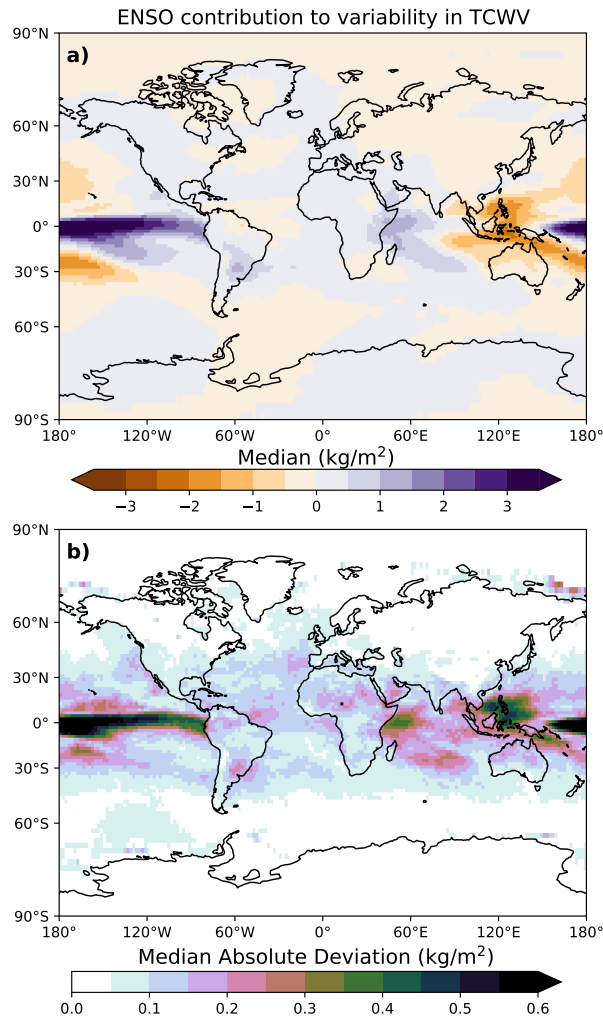
Figure 3. Archive ensemble median (a) Median ENSO contribution to the variability in TCWV for all archive ensemble members that cover the common long period (between 1988-2014) and. The median absolute deviation-Absolute Deviation (MAD) to for the ensemble median ENSO contribution is shown in (b).
