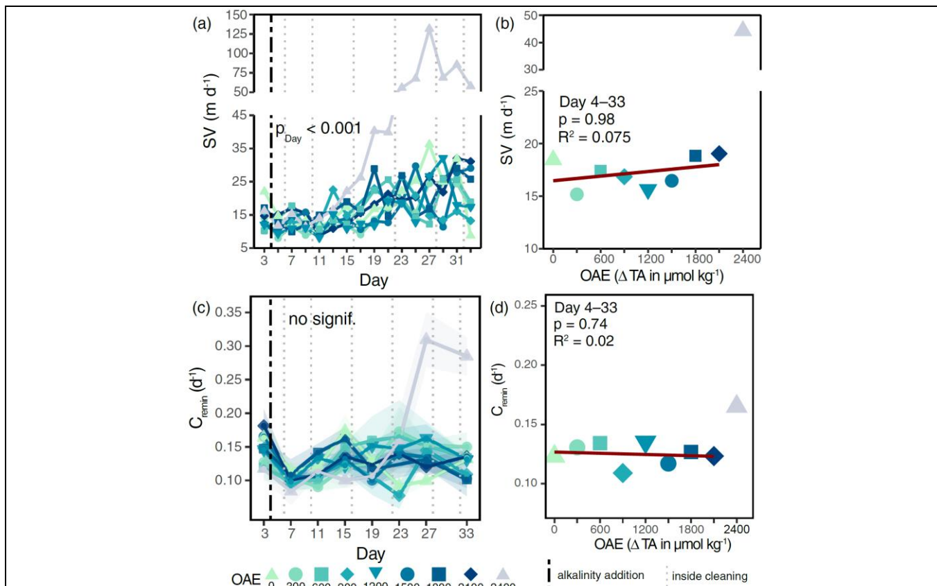
Figure 3| Depth attenuation of the organic matter flux under the application of OAE. Development of average particle sinking velocities under OAE over time (a) and as averages over the treatment period (b). Carbon specific remineralization rates (c) and averages under OAE (d). Shaded areas in (c) indicate standard deviations of measurements ( n_{\text{min}} = 3 ). p-values in (a) and (c) represent the output of linear mixed effects models (Table S3f,m). The vertical black line indicates the alkalinity addition and the grey lines the inside cleaning of the mesocosm walls (a,c). 295
