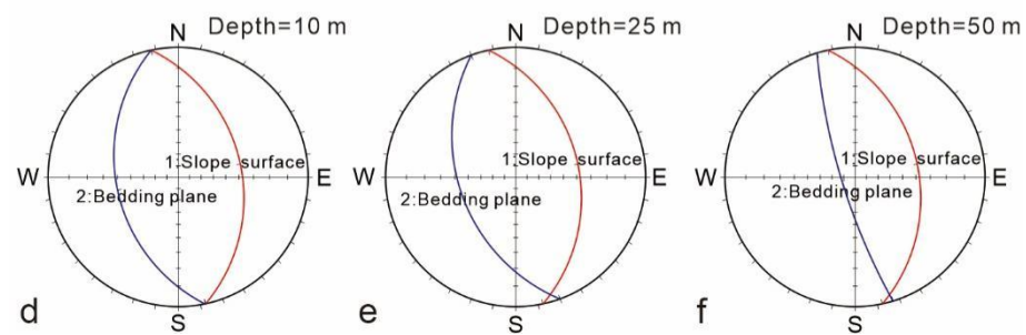
1 2 Figure 6: Rock cores and stereographic projections at different depths. a–c Rock cores at the depth of 10 m, 25 m, and 50 m, 3 respectively in borehole zk20. The diameters of the drilling hole are 100 mm and 60 mm at the depth of 0–15 m and 15–70 m, 4 respectively. d–f Stereographic projections at the depths of 10 m, 25 m, and 50 m, respectively.
