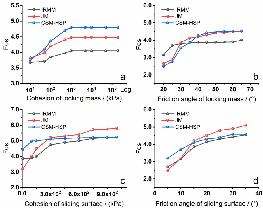
1 2 Figure 16: 3D Fos curves under different strength parameters.
