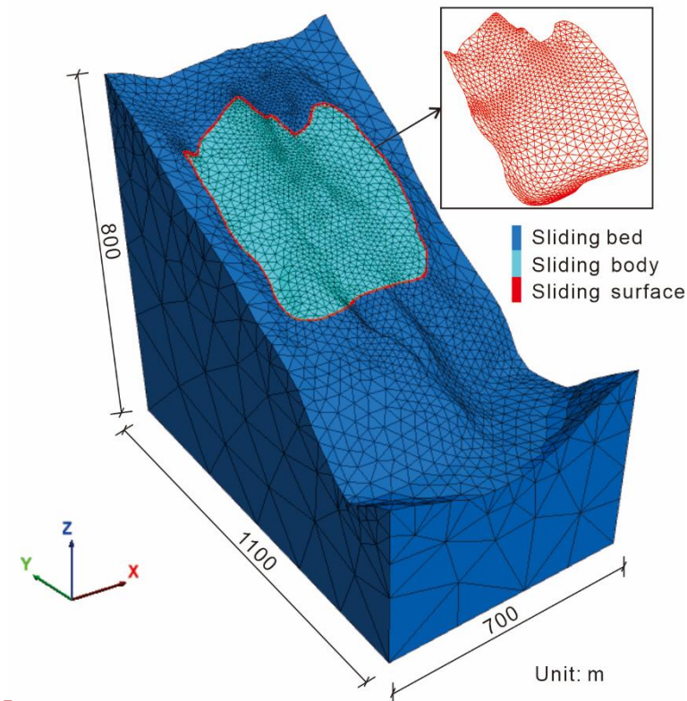
Figure 10: The mesh model and geometry of the Tizicao landslide.
