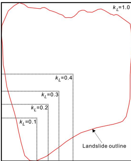
Figure 14: Locking areas under different locking ratios.
