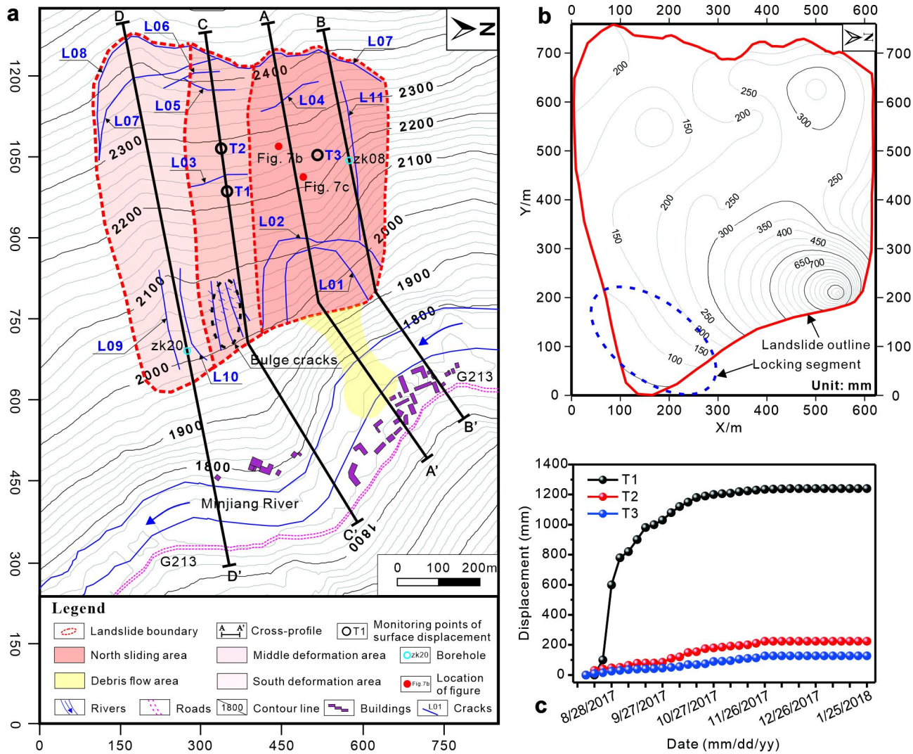
3 Figure 3: The topographic plan, isoline map of surface displacement, and displacement monitoring curves of the Tizicao landslide. 4 a Topographic plan of the deformation areas, the crack distribution, and the locations of engineering-geotechnical sections (after 5 Zhou et al., 2022). b Isoline map of the surface displacement of the Tizicao landslide from August 13, 2017, to January 25, 2018 6 (Zhou et al., 2022); c Displacement monitoring curves of the landslide surface (from August 13, 2017, to January 25, 2018).
