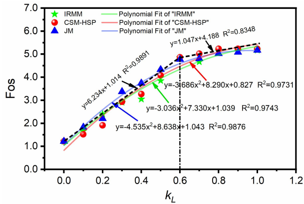
Figure 15: 3D Fos curves under different locking ratios, obtained using three rock bridge models.
