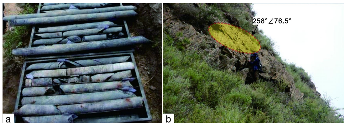
5 6 Figure 5: Rock cores drilled from borehole zk20 and exposed phyllites at the back of the landslide. a Intact rock cores (Zhou et al., 7 2022). b Exposed phyllites with an attitude of 258°∠76.5°.
