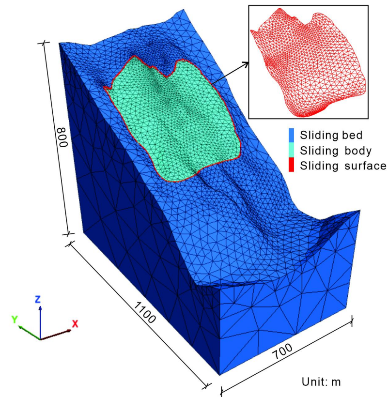
7 Figure 10: The mesh model and geometry of the Tizicao landslide.
