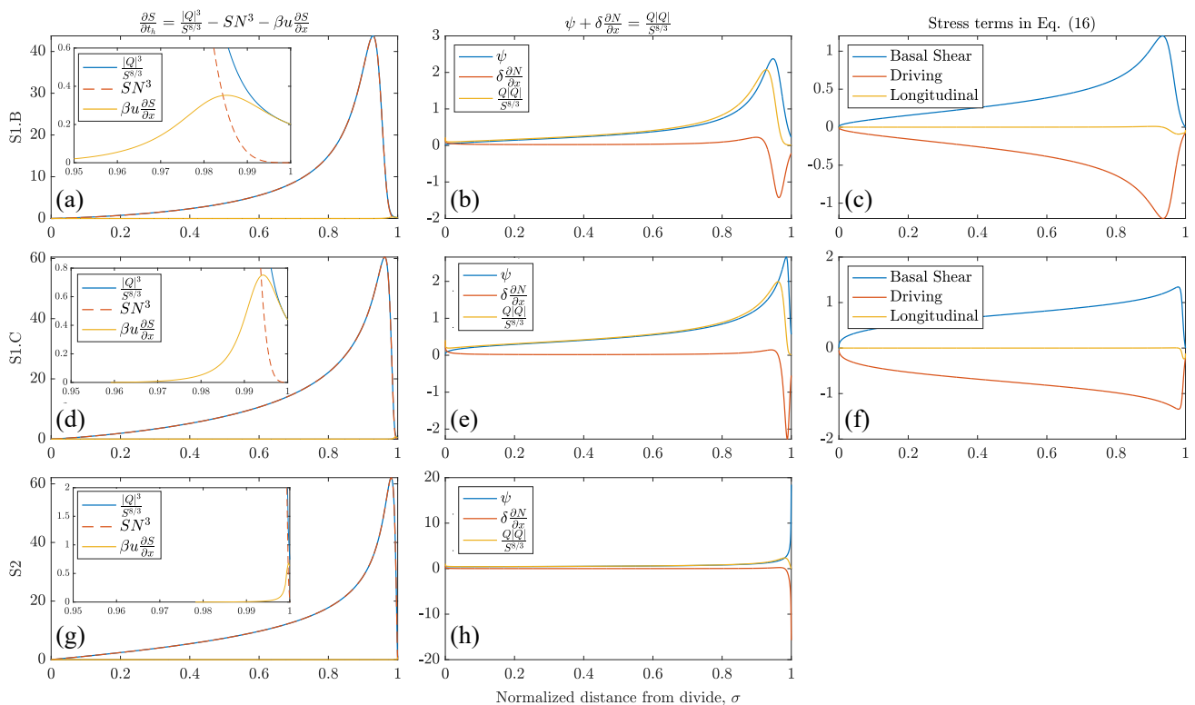
Figure 5. Term-by-term plots of the steady-state solution to the coupled model (S1). The terms in the equation for channel evolution (left column: a, d, g), in the equation for conservation of momentum in the channel (middle column: b, e, h), and in the equation for conservation of momentum in the ice (right column: c, f) for the steady-state coupled model solution using a Budd sliding law (top row: a-c), the solution using a regularized Coulomb law (middle row: d-f), and the one-way forced solution using an imposed quadratic ice geometry (bottom row: g, h).
