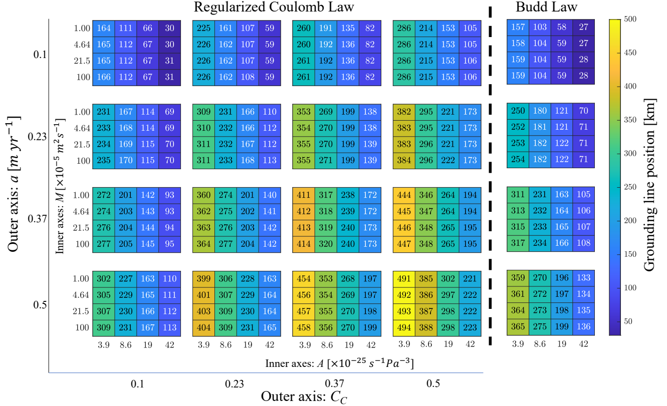
Figure 3. The sensitivity of the coupled model steady-state with a regularized Coulomb law's steady-state grounding line position to (each column, from left to right) the depth-averaged flow law constant A (inner x-axis), the accumulation rate a , the additional water source term M (inner y-axis), the water flux at the divide Q_m , and the sliding-law-specific constants A_s and C_C . The top row accumulation rate a (a-fouter y-axis) shows. Each column of plots corresponds to a different value of C_C for the steady-state grounding line position, the middle row model using a regularized Coulomb law (g-louter x-axis) shows the ice thickness h , while except for the bottom row (m-r) shows the effective pressure N . The parameter values held constant in the other rightmost column which contains results from experiments are marked by the dashed black lines that used a Budd law.
