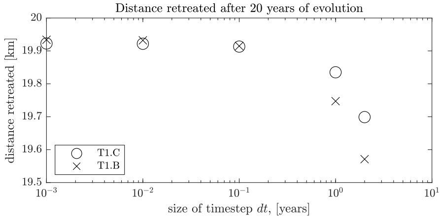
Figure D2. Grounding-line retreat after 20 years simulated by the transient, coupled model using a range of time-step sizes and each sliding law. Other than the time steps, all other parameters are the same as used in T1.B and T1.C.
