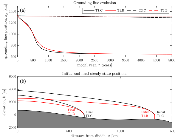
Figure 6. (a) The grounding-line position and (b) the initial and final ice-thickness profiles of the coupled model with a regularized Coulomb law (T1.C, black solid curves) and a Budd law (T1.B, red solid curves) over 5000 years of evolution after a perturbation to a fully removing ice-shelf buttressing (by changing B from 0.9 \times 10^{-25} \text{ s}^{-1} \text{ Pa}^{-3} to 2.9 \times 10^{-25} \text{ s}^{-1} \text{ Pa}^{-3} ) over 10 years. The dashed curves show the evolution of the static- N model experiment using a regularized Coulomb law (T2.C, black dashed curve) and a Budd law (T2.B, red dashed curve). The upper boundary of lower shaded region is the ice-sheet bed.
