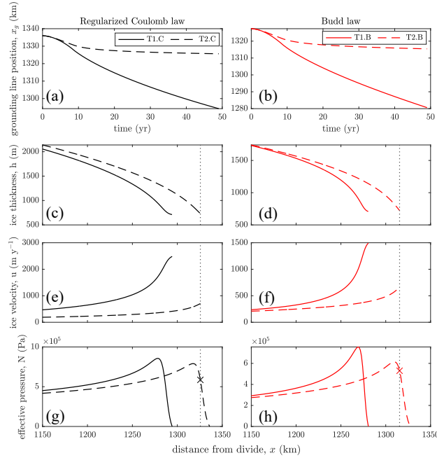
Figure 7. The grounding-line position over 40–50 years of evolution for the coupled model-experiment (T1, solid curves) and static- N model-experiment (T2, dashed curves) using a (a) regularized Coulomb law (black curves) and (b) Budd law (red curves). The (c,d) ice thickness, (e,f) ice velocity, and (g,h) effective pressure profiles after 40–50 years of evolution for the models described above. The vertical dotted lines show the position of the static- N grounding lines after 40–50 years. For the static- N effective-pressure profiles, we plot the initial steady-state profiles and the crosses indicate the effective pressure immediately upstream of the grounding line after 40–50 years of evolution.
