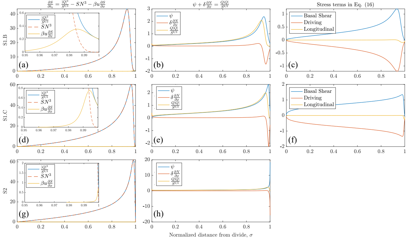
Figure 5. Term-by-term plots of the steady-state solution to the coupled model (S1). The terms in the nondimensional steady-state equation for channel evolution (left column: a, d, g), in the equation for channel -conservation of momentum in the channel (middle column: b, e, h), and in the equation for ice -conservation of momentum in the ice (right column: c, f) for the steady-state coupled model solution using a Budd sliding law (top row: a-c), the solution using a regularized Coulomb law (middle row: d-f), and the one-way coupled-forced solution using an imposed quadratic ice geometry (bottom row: g, h).
