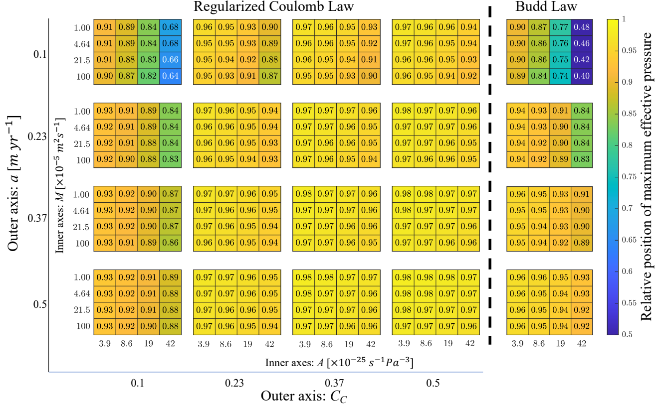
Figure 4. The sensitivity of the coupled model steady-state with a Budd law to a 's relative location (each column 0 is the divide, from left to right 1 is the grounding line) of peak effective pressure to the depth-averaged flow law constant A (inner x-axis), the accumulation rate \alpha , the additional water source term M (inner y-axis), and the water flux at the divide Q_m , and the sliding-law-specific constant C_B . The top row accumulation rate a (a-e outer y-axis). Each column of plots corresponds to a different value of C_C for the steady-state grounding line position, the middle row model using a regularized Coulomb law (f-j outer x-axis) plots the ice thickness h , while except for the bottom row (k-o) plots the effective pressure N . The parameter values held constant in the other rightmost column which contains results from experiments are marked by the dashed black lines that used a Budd law.
