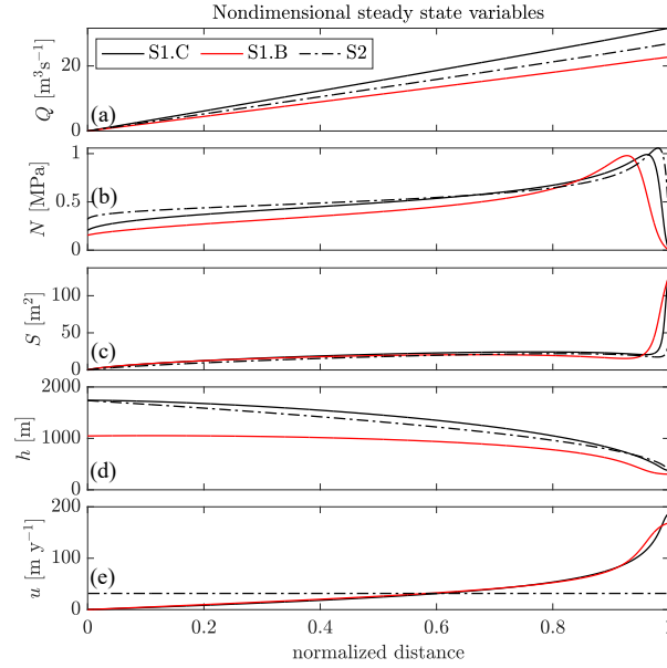
Figure 2. The steady-state profiles for: (a) channel discharge, (b) effective pressure, (c) channel cross-sectional area, (d) ice thickness, and (e) ice velocity. The results of the coupled simulations with the regularized Coulomb law (S1.C) are in black, the results from simulations using the Budd law (S1.B) are in red, and the results from the one-way coupled model with imposed thickness and velocity (S2) are in black dash-dotted curves.
