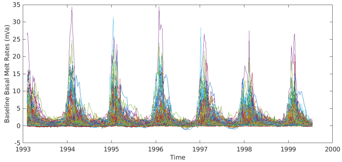
Figure A8. The baseline MITgcm basal melt rates for the identified sensitive regions (greater than 2e - 11 \text{ m}^{-2} ) on the RIS. Each coloured line represents a basal melt at different sensitive region regions (i.e., different nodes of the mesh).
