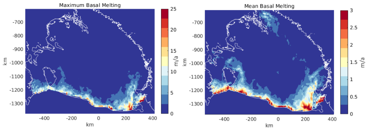
Figure 5. MITgcm short-term summer maximum and mean basal melt rates (in m/a) on the RIS.
