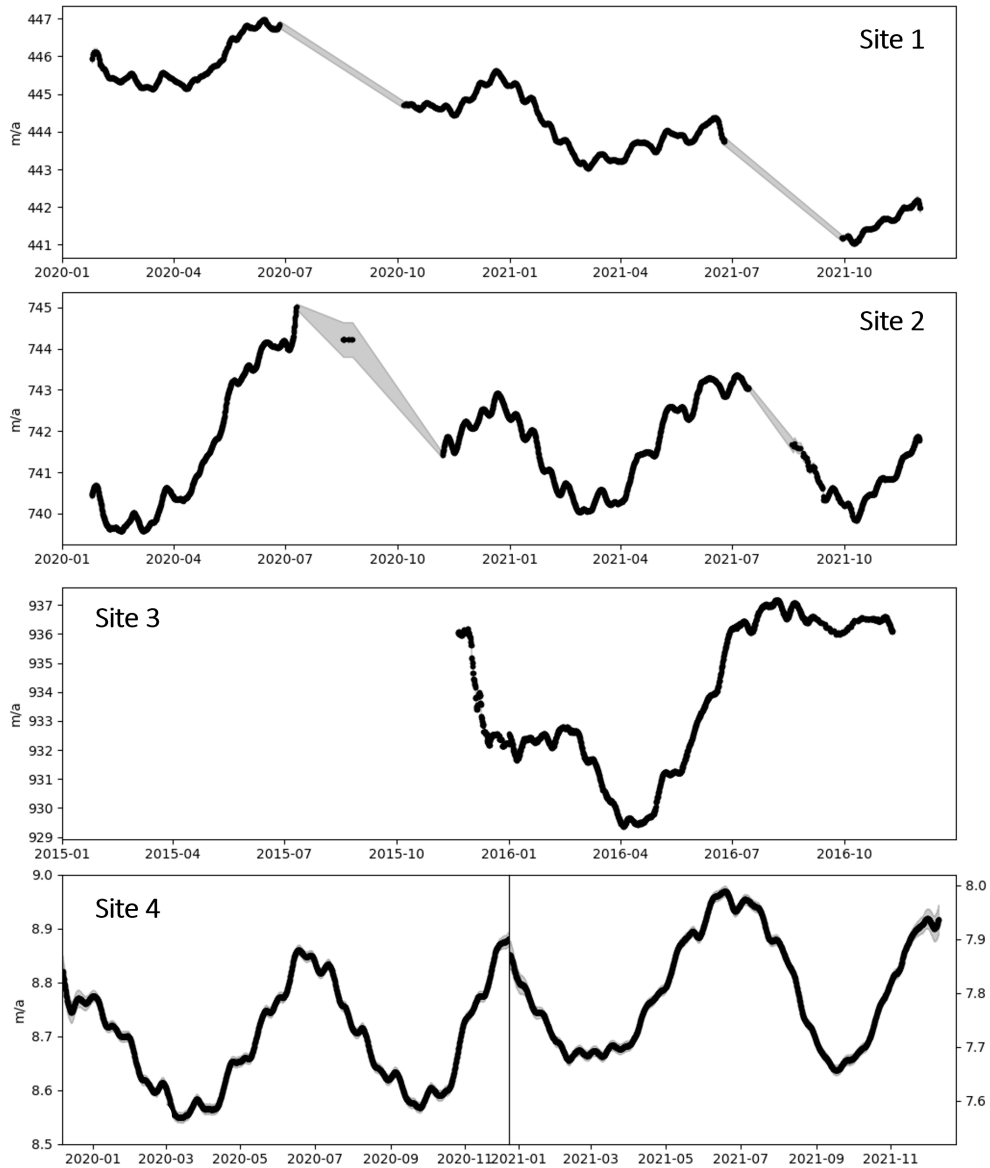
Figure 2. The GNSS velocities (in m/a) at Site 1 (shear margin region close to Ross Island), Site 2 (Coulman High region close to the calving front), Site 3 (mid-shelf region), and Site 4 (Kamb Ice Stream-KIS grounding linezone). The errors uncertainties are provided in the grey windows enclosing the black lines. These errors uncertainties are not visible in a few places, as the errors they are very small. Detrended position and direction for each site is shown in Figures A1-A4
