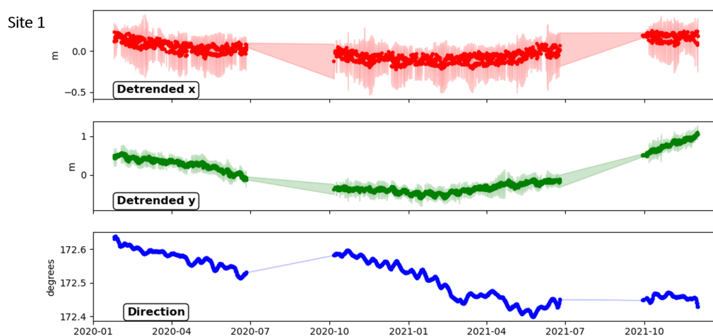
Figure A1. Site 1 GNSS detrended position (x, y) and direction (clockwise from from-grid north).
