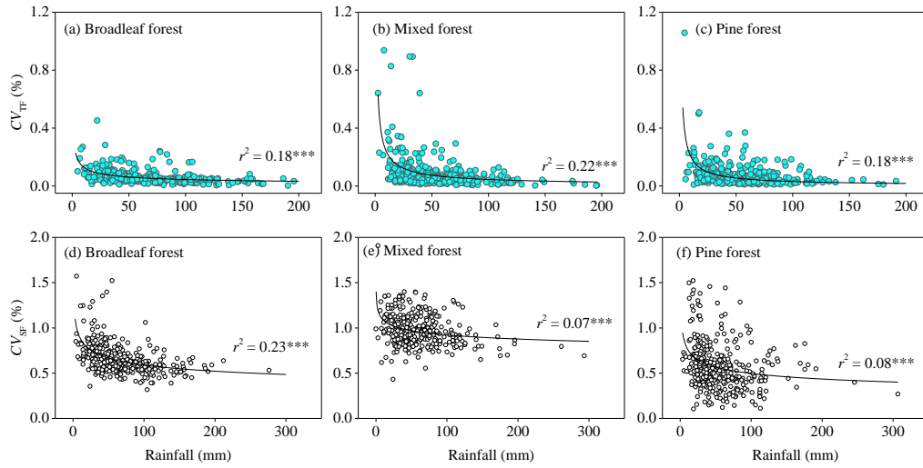
Fig. S1 Coefficient of variation changing of throughfall ratio (a~c) and stemflow ratio (d~f) with rainfall volume. r : Pearson coefficient of correlation; *: P < 0.05 , **: P < 0.01 , ***: P < 0.001
