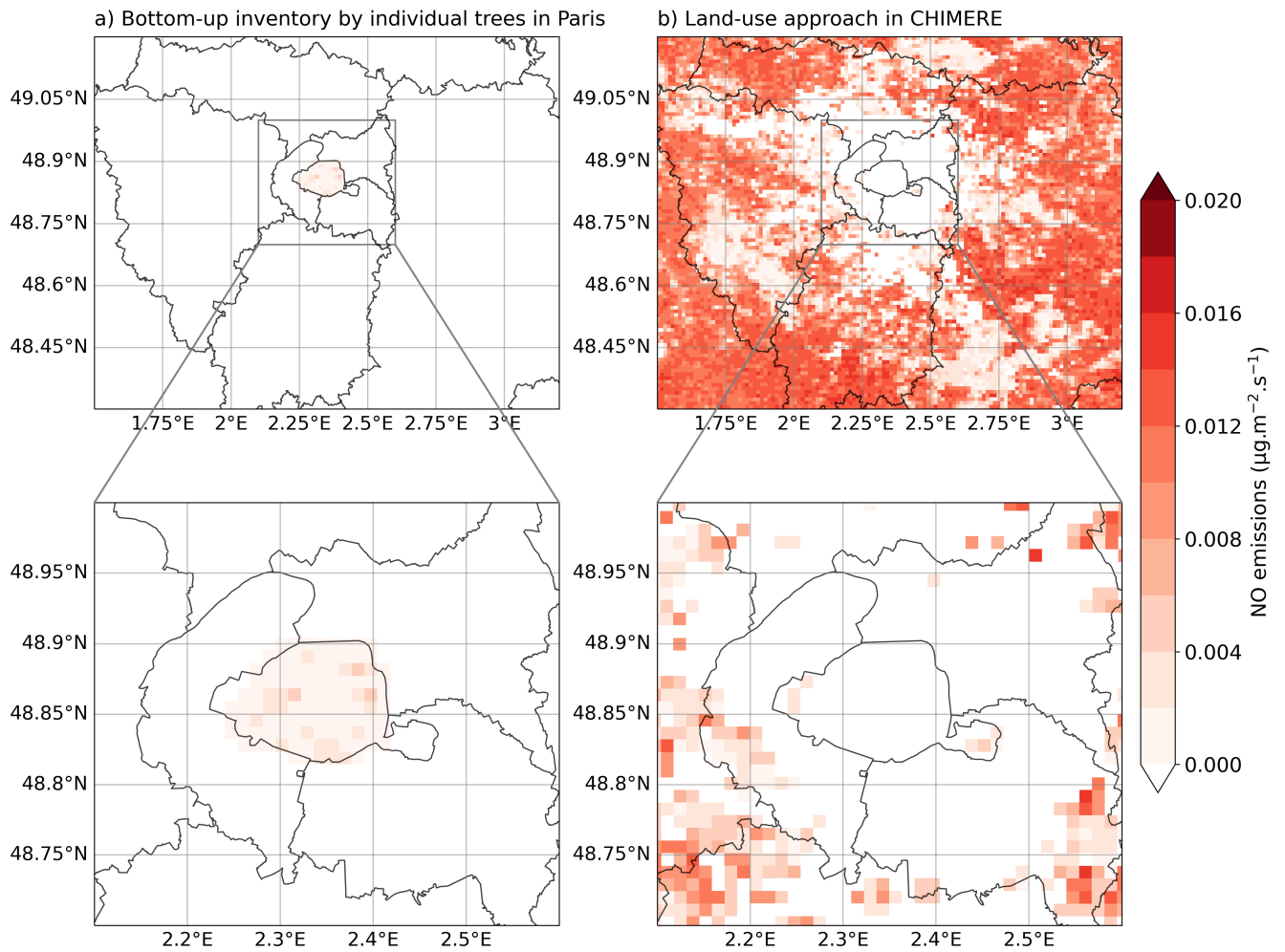
Figure D5. Comparison of the 2 months nitrite oxide (NO) emissions computed with (a) the "bottom-up" inventory and (b) with the land-cover approach in CHIMERE over Île-de-France and Greater Paris.
