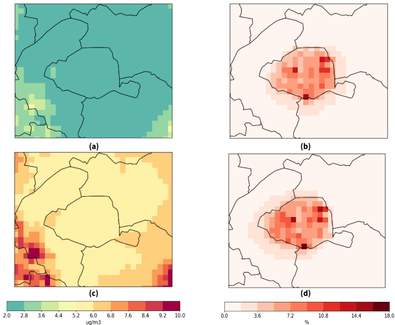
Figure 10. Average OM concentrations ( \mu\text{g.m}^{-3} ) simulated by CHIMERE (REF-TX2) during (a) the whole period and (c) the heatwave and relative difference of OM concentrations with the urban-tree biogenic emissions (bioparis-TX2) during (b) the whole period and (d) the heatwave.
