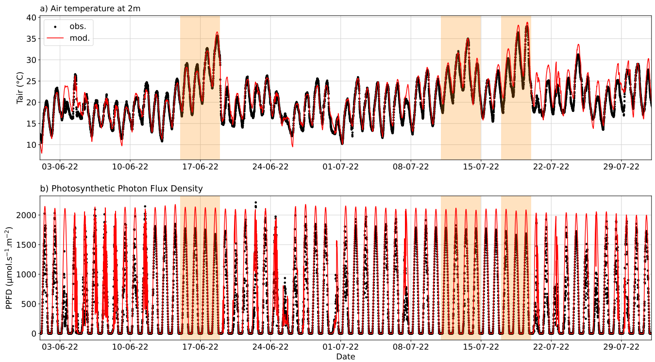
Figure E1. Comparison of the temporal variation of (a) air temperature at 2 m height and (b) photosynthetic photo flux density modeled by WRF (mod) and observed (obs) at the SIRTA observatory site ( 48.717347^\circ N, 2.208868^\circ E). Heatwave periods are indicated by orange shaded areas.
