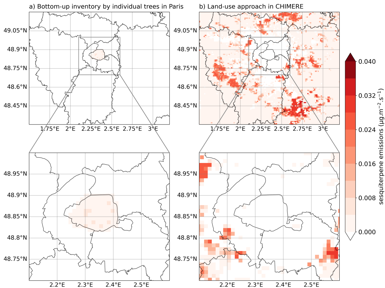
Figure D4. Comparison of the 2 months sesquiterpene emissions computed with (a) the "bottom-up" inventory and (b) with the land-cover approach in CHIMERE over Île-de-France and Greater Paris.
