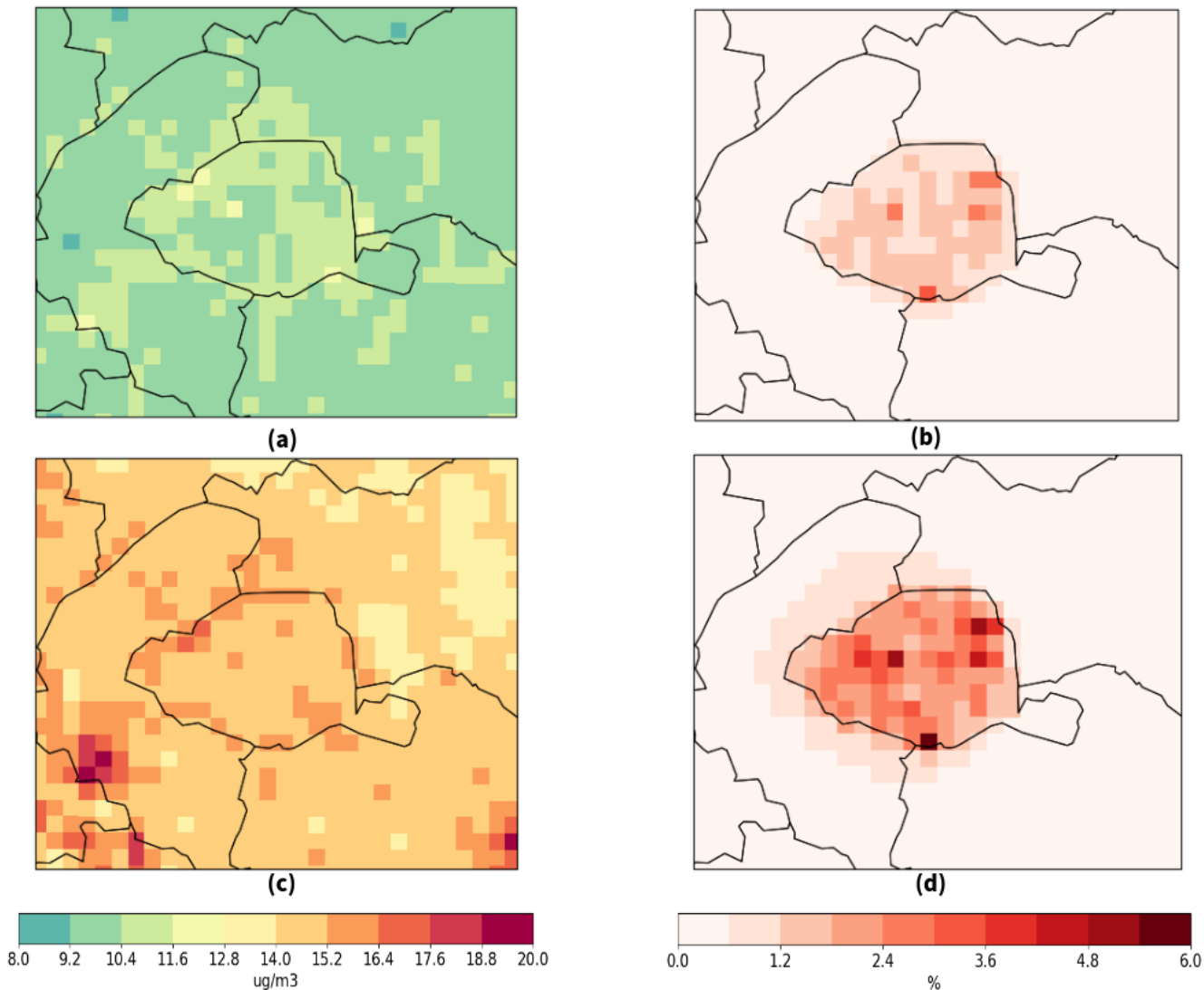
Figure 11. Average \text{PM}_{2.5} concentrations ( \mu\text{g}\cdot\text{m}^{-3} ) simulated by CHIMERE (REF-TX2) during (a) the whole period and (c) the heatwave and relative difference of \text{PM}_{2.5} concentrations with the urban-tree biogenic emissions (bioparis-TX2) during (b) the whole period and (d) the heatwave.
