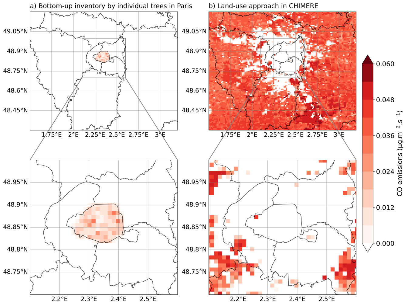
Figure D6. Comparison of the 2 months carbon monoxide (CO) emissions computed with (a) the "bottom-up" inventory and (b) with the land-cover approach in CHIMERE over Île-de-France and Greater Paris.
