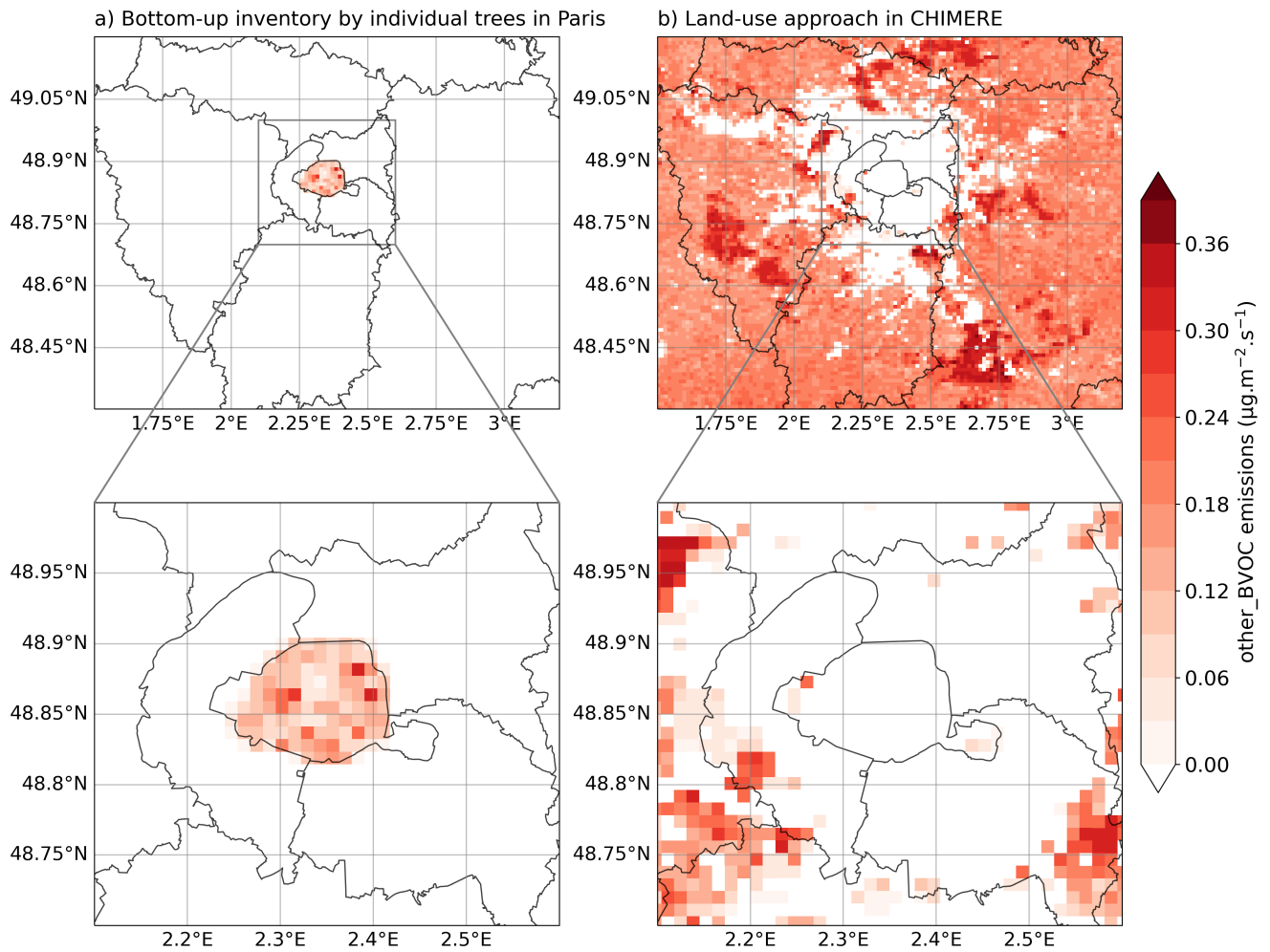
Figure D7. Comparison of the 2 months other VOC (OVOC) emissions computed with (a) the "bottom-up" inventory and (b) with the land-cover approach in CHIMERE over Île-de-France and Greater Paris.
