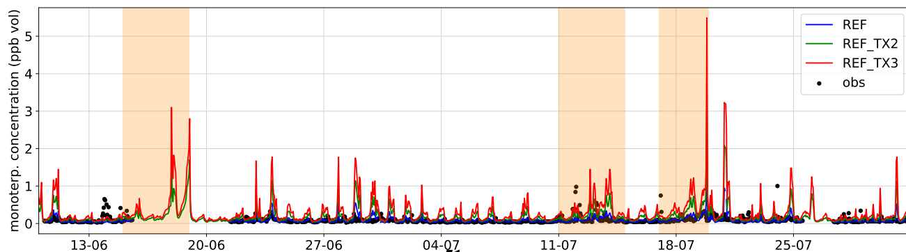
Figure F2. Observed and simulated hourly concentrations of (a) isoprene and (b) monoterpenes at the PRG station and (c) isoprene and (d) monoterpenes at the SIRTA station. Heatwave periods are indicated by orange shaded areas.
