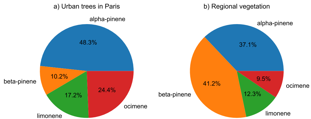
Figure D3. Distribution of monoterpene species emitted, summed over the two months (a) for the urban trees in Paris computed with the bottom-up inventory and (b) for the vegetation over Île-de-France region computed with the land-use approach.
