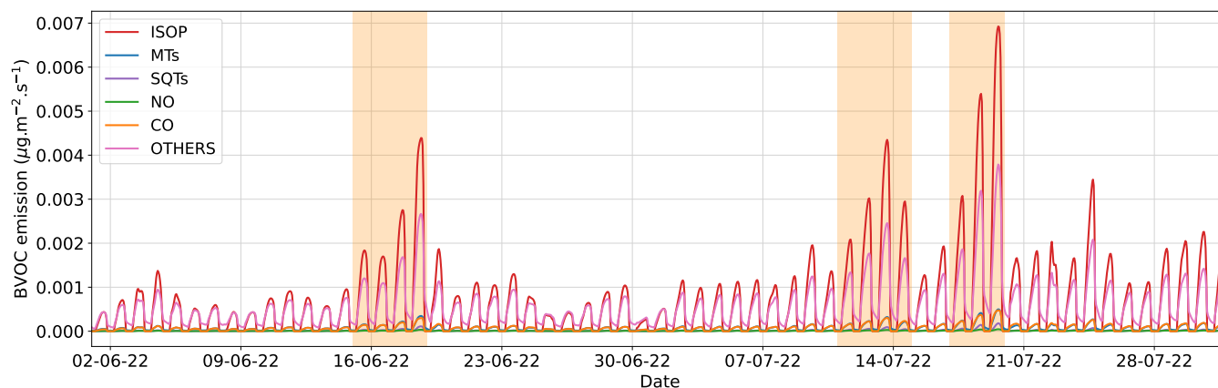
Figure 7. Temporal variation of the spatially averaged biogenic emissions computed over Paris with the bottom-up inventory. Heatwave periods are indicated by orange shaded areas.
