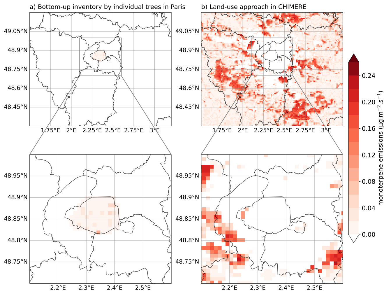
Figure D2. Comparison of the 2 months averaged monoterpene emissions computed with (a) the "bottom-up" inventory and (b) with the land-cover approach in CHIMERE over Île-de-France and Greater Paris.
