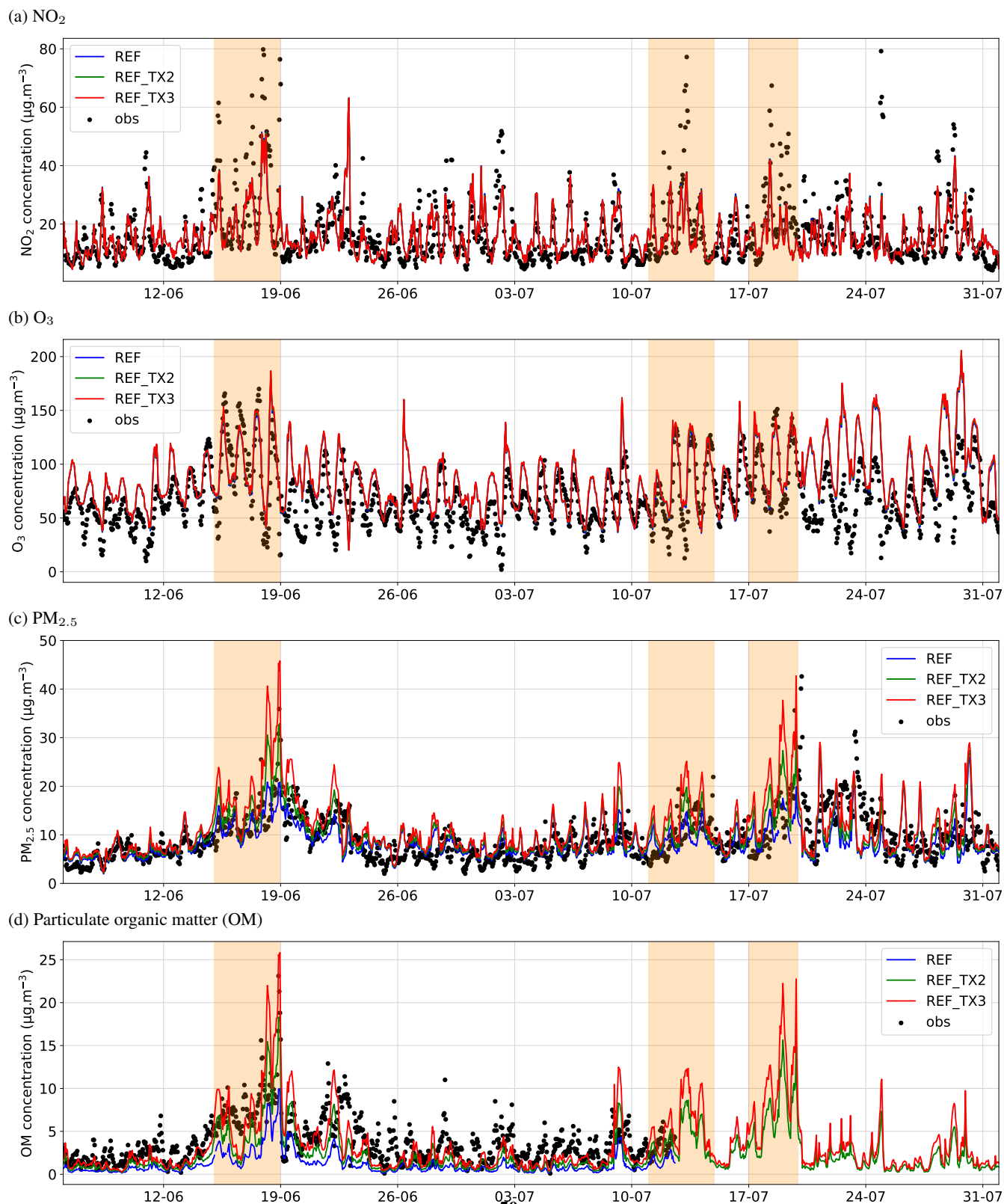
Figure F1. Observed and simulated hourly concentrations of (a) \text{NO}_2 , (b) \text{O}_3 (c) \text{PM}_{2.5} and (d) OM at the Halles station. Heatwave periods are indicated by orange shaded areas.
