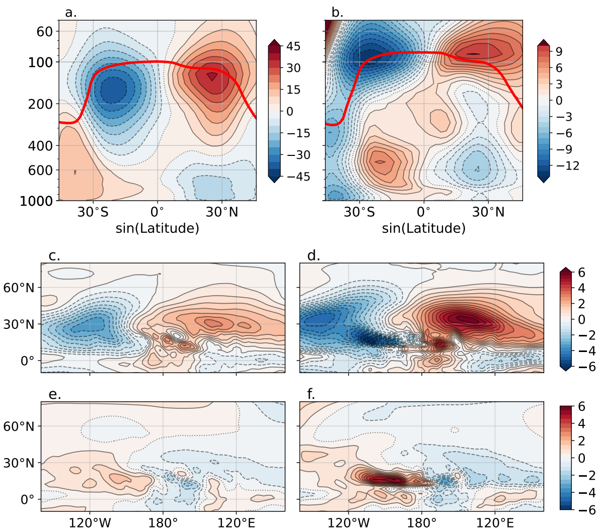
Figure 11. Steady-state statistics for the aquaplanet runs averaged over year 3 of the simulation. (Top; a,b) Vertical structure of eddy streamfunction ( \psi ; units: 10^6 \text{ m}^2 \text{ s}^{-1} ) for (a) control simulation and (b) difference between forced and control simulations. (Middle; c,d) Eddy pressure velocity ( \omega ; units: \text{hPa} \cdot \text{day}^{-1} ) distribution for (c) control and (d) forced simulations. (Bottom; e,f) Eddy divergence field ( \nabla \cdot \mathbf{u} ; units: 10^6 \text{ s}^{-1} ) distribution for (c) control and (d) forced simulations. The results in panels (a,b) are averaged over 120^\circ\text{E} - 120^\circ\text{W} because the peak of the SST forcing lies in this longitude band. The results in panels (c,d,e,f) are all averaged over 60 - 100 mbar.
