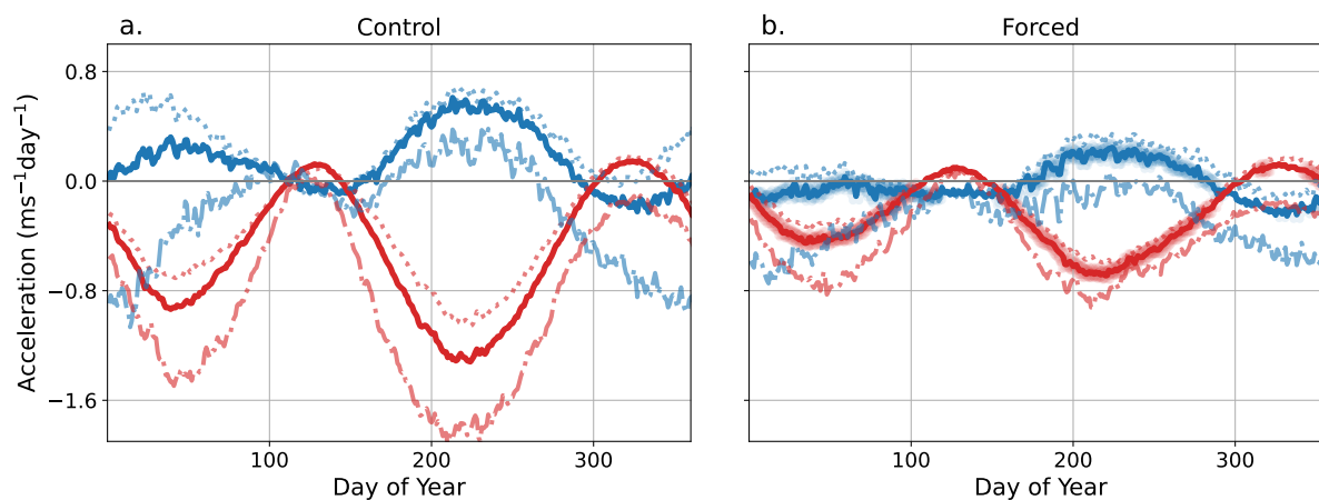
Figure 5. Same as Figure 3a, except for CMIP6 (left) control and (right) forced sets. The blurring of the curves, in panel b, indicates days where the full eddy and mean terms related to the forced simulations are statistically different from those for control at the 95% level of significance.
