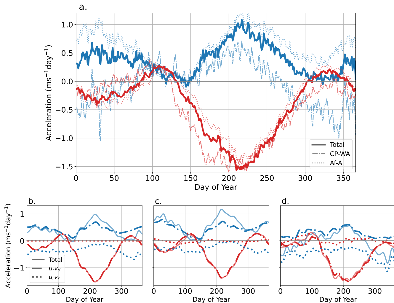
Figure 3. Panel (a) shows the climatological Day of Year variation of the horizontal eddy and mean terms of the upper-level momentum balance computed over the global longitudes and over the Af-A and CP-WA sectors. The eddy momentum flux convergence is presented in blue, and the mean meridional advection is presented in red. The eddy and mean momentum terms computed over the Af-A and CP-WA regions are shown in dotted and dash-dotted lines, respectively. The eddy and mean fluxes shown in thick blue and red lines are the same quantities that were shown in Figure 1, shown here again for reference. The quantities in panels (b), (c), and (d) show the rotational-divergent partition of the eddy and mean terms computed over the global longitudes, Af-A, and CP-WA sectors, respectively. The divergent component ( u_r v_d ) is shown in dash-dotted lines, while the rotational component ( u_r v_r ) is shown in dotted lines. The u_d v_d and u_d v_r fluxes were found to be small and have not been considered. All quantities are averaged over 150-300 mbar, and \pm 5^\circ about the equator. A 20-day low-pass filter is applied to the quantities in panels b, c, and d prior to presentation. In all panels, the x -axis is Day of Year and the y -axis is Acceleration ( \text{ms}^{-1}\text{day}^{-1} ), as in Figure 1. Legend marked in panel (b) also applies to panels (c) and (d).
