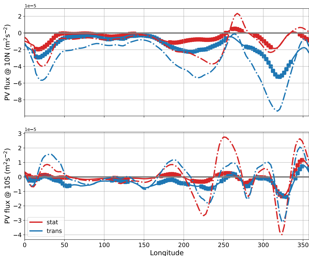
Figure 13. Stationary (red) and transient (blue) fluxes of PV along (top) 10°N and (bottom) 10°S on the 350 K isentrope averaged over winter (DJF). The solid (dash-dotted) curve represents the forced (control) set. Points marked with squares are statistically significant at the 95% level.
