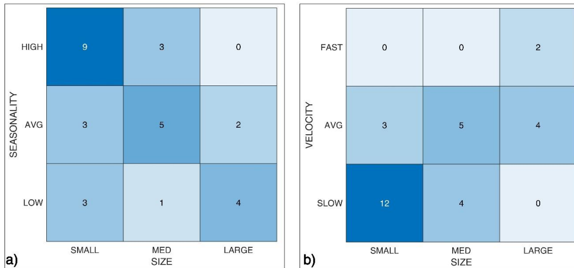
394 Fig. 10 Glacier classification according to their size (SMALL: <1 km 2 ; MED: 1-4 km 2 ; LARGE: >4 km 2 ) and a) 395 seasonal velocity behaviour (qualitatively estimated) and b) median velocity (SLOW: <100 m yr -1 ; AVG: 100-300 m 396 yr -1 ; FAST: >300 m yr -1 ). The digits within the grid tiles indicate the number of glaciers belonging to each group. 397
