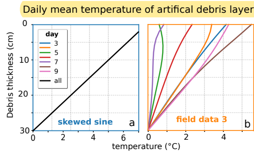
Figure 5. Daily averaged debris layer temperature profile based on figure 4.
