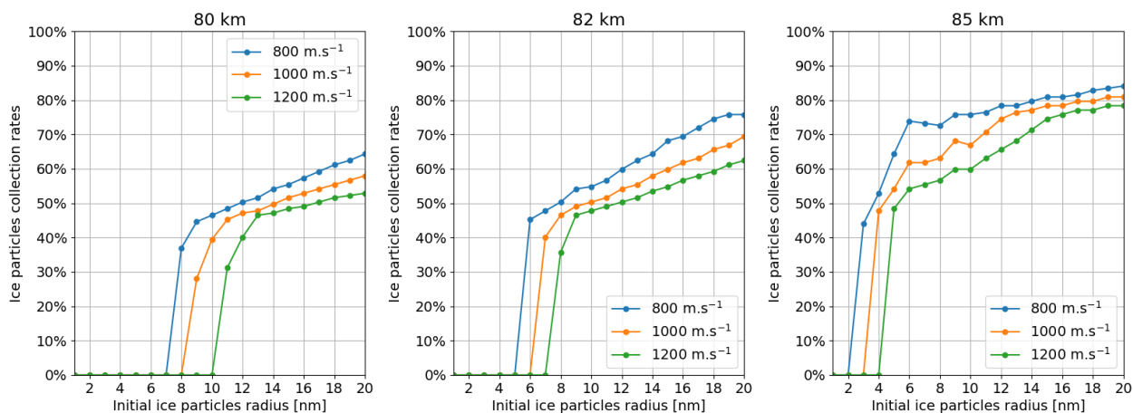
Figure 8. Ice particles collection rates as a function of their initial radius for three different rocket speeds 800 \text{ m.s}^{-1} , 1000 \text{ m.s}^{-1} and 1200 \text{ m.s}^{-1} and three different altitudes 80km, 82km and 85km. Each point of the graphs has been obtained by calculating the trajectories of about 150 ice particles.
