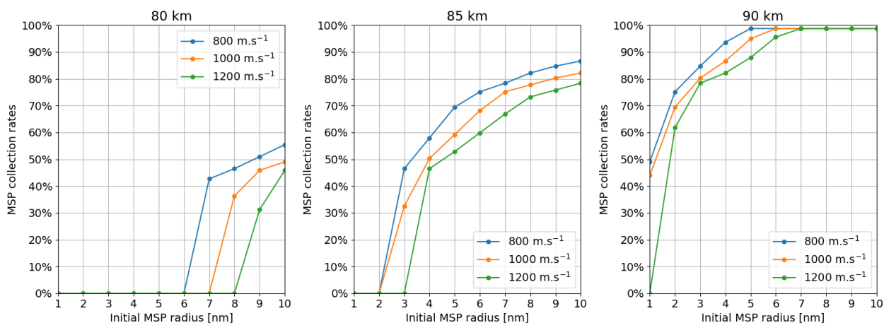
Figure 9. MSP collection rates as a function of their initial radius for three different rocket speeds 800 \text{ m.s}^{-1} , 1000 \text{ m.s}^{-1} and 1200 \text{ m.s}^{-1} and three different altitudes 80km, 85km and 90km. Each point of the graphs has been obtained by calculating the trajectories of about 150 MSP.
