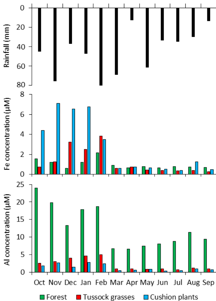
Figure S4: Mean monthly rainfall (mm) and mean monthly Al and Fe concentrations ( \mu\text{M L}^{-1} ) in soil solutes under forests, tussock grasses and cushion-forming plants.
