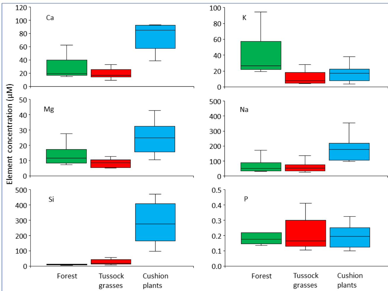
Figure S2: Major element concentrations in soil pore water ( \mu\text{M L}^{-1} ) under forests (n=7), tussock grasses (n=15) and cushion plants (n=9).
