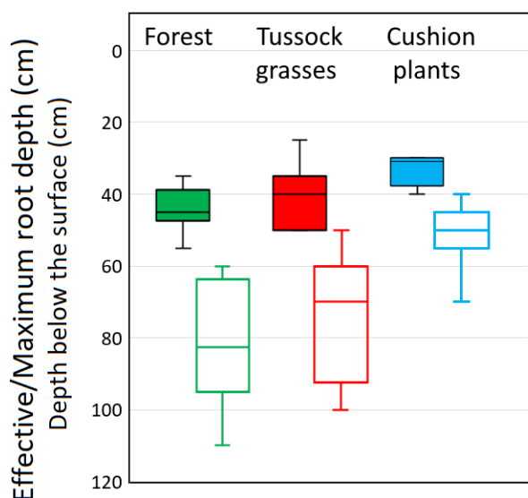
270 Figure 2: Depth-distribution of root development in forests (n=9, green), under tussock grasses (n=15, red) and cushion-forming plants (n=9, blue). The effective rooting depth (colour-filled boxplots) contains > 90% of the root biomass and corresponds to the maximum depth at which vegetation effectively uses plant-available water. The maximum rooting depth (unfilled boxplots) refers to the deepest rooting depth observed in the C horizons. The boxplots show the median, the 25 th and 75 th percentile, and the whiskers the minimum and maximum observed values.
