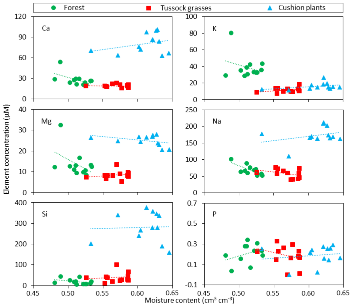
395 Figure 8: Relation between the mean monthly soil solute concentrations of Ca, K, Mg, Na, Si and P and mean monthly volumetric soil moisture contents under forest, tussock grasses and cushion plants. The mean monthly values are calculated from the biweekly measurements realised under forest (n=7), tussock grasses (n=15) and cushion plants (n=9).
