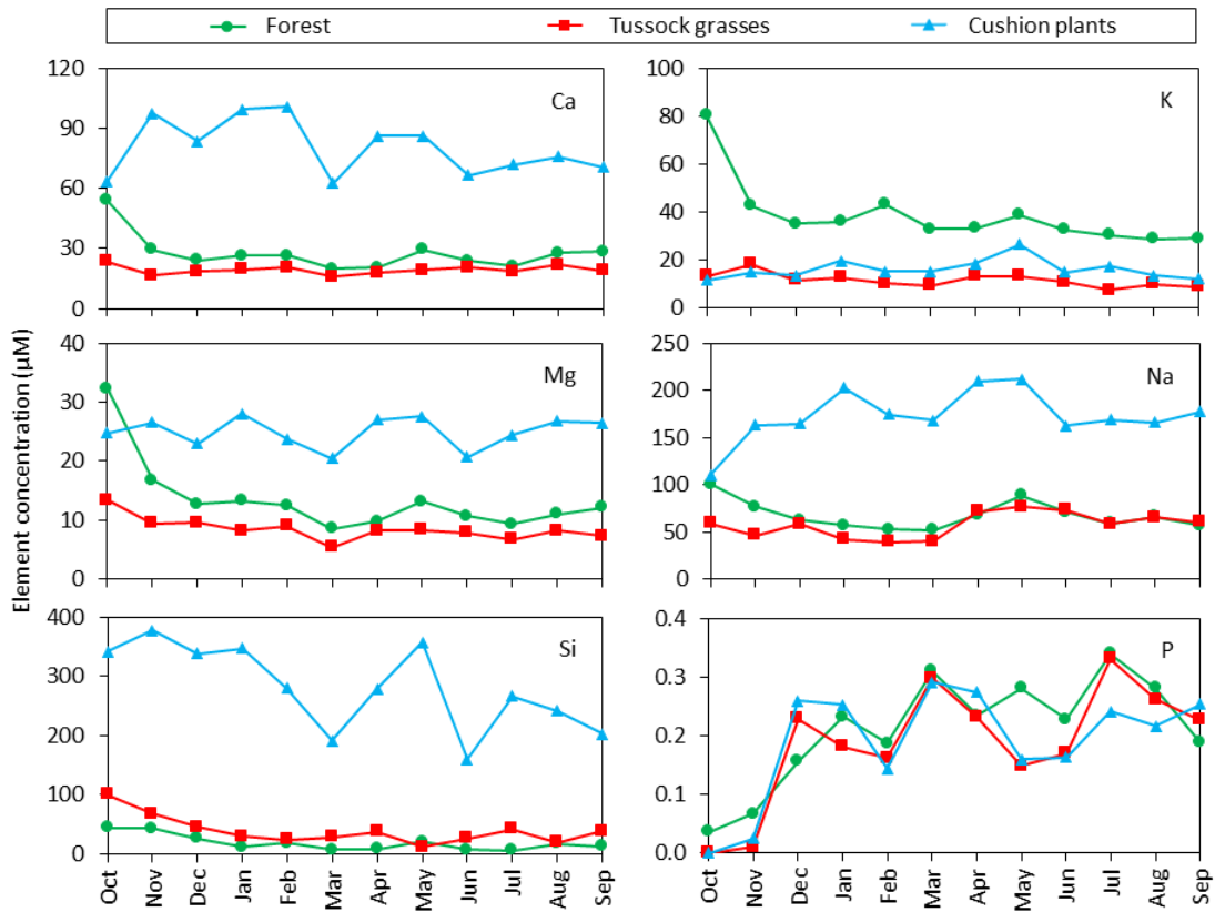
Figure 7: Temporal variation in soil solute concentrations under forest ( n=7 ), tussock grasses ( n=15 ) and cushion plants ( n=9 ). The mean monthly values for the period October 2012 till September 2013 are plotted in the graphs. Even after a 2-month equilibration period, we cannot entirely exclude that the first cation concentration measurements under forest (October 2012) are higher-than-expected due to incomplete stabilization of the lysimeters after installation (e.g. preferential flow because of lysimeter insertion).
