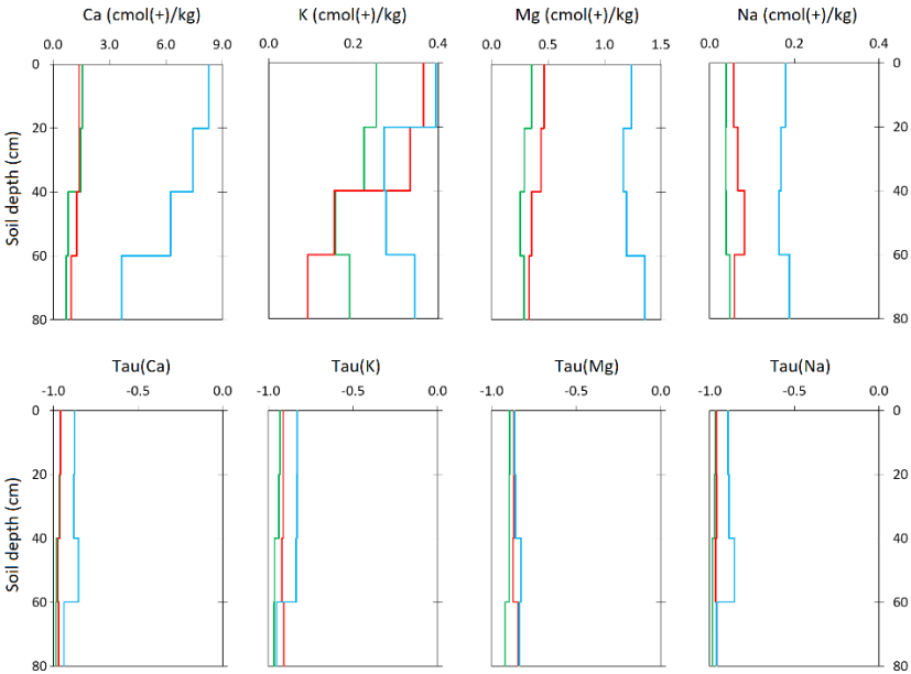
Figure 3: Depth-variation of the mean exchangeable Ca, K, Mg, and Na concentrations, and the mean elemental mass transfer coefficients in soils under forests (n=7, green line), tussock grasses (n=15, red line) and cushion-forming plants (n=9, blue line). The plots show the average values derived from the measurements at the individual soil profiles.
