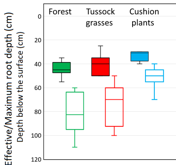
265 Figure 2: Depth-distribution of root development in forests (n=9, green), under tussock grasses (n=15, red) and cushion-forming plants (n=9, blue). The effective rooting depth contains > 90% of the root biomass and corresponds to the maximum depth at which vegetation effectively uses plant-available water. The maximum rooting depth refers to the deepest rooting depth observed in the C horizons.
