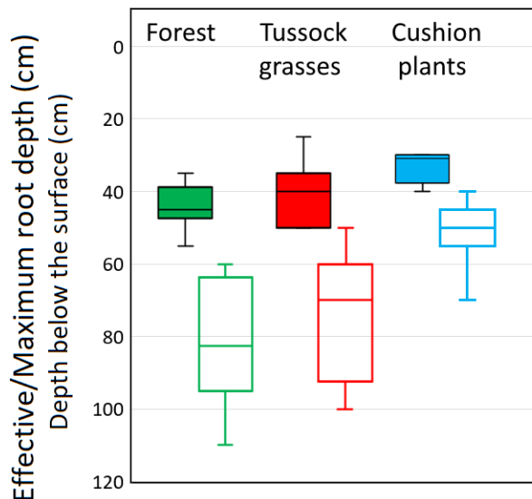
Figure 2: Depth-distribution of root development in forests (n=9, green), under tussock grasses (n=15, red) and cushion-forming plants (n=9, blue). The effective rooting depth contains > 90% of the root biomass and corresponds to the maximum depth at which vegetation effectively uses plant-available water. The maximum rooting depth refers to the deepest rooting depth observed in the C horizons.
