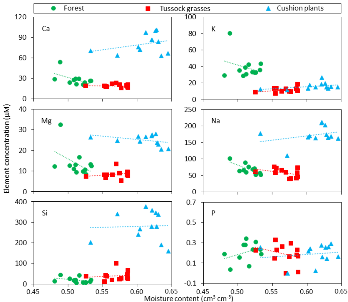
Figure 8: Relation between the mean monthly soil solute concentrations of Ca, K, Mg, Na, Si and P and mean monthly volumetric soil moisture contents under forest, tussock grasses and cushion plants. The mean monthly values are calculated from the biweekly measurements realised under forest (n=7), tussock grasses (n=15) and cushion plants (n=9).
