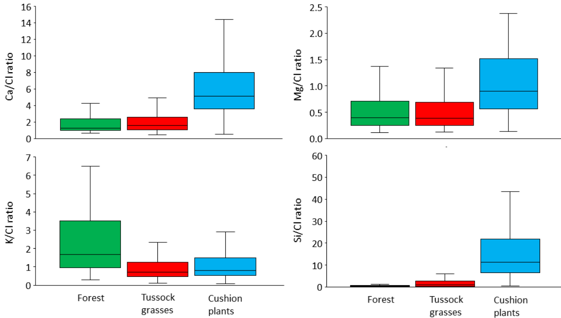
370 Figure 6: Ratio of Ca, Mg and K nutrients to Chloride in the soil solutions under forests (n=7), tussock grasses (n=15) and cushion plants (n=9), based on the biweekly sampling from October 2012 to September 2013. An increase in the ratio indicates an enrichment of the nutrient relative to Cl, and a decrease a removal of the nutrient compared to Cl. The boxplots show the median, the 25 th and 75 th percentile, and the whiskers the minimum and maximum observed values.
