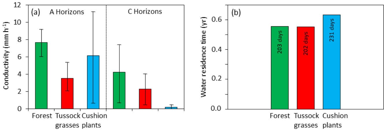
Figure 5: Mean saturated hydraulic conductivity (mm h -1 ) and mean water residence time (yr) under forest, tussock grasses and cushion-forming plants for period between October 2012 and September 2013.
