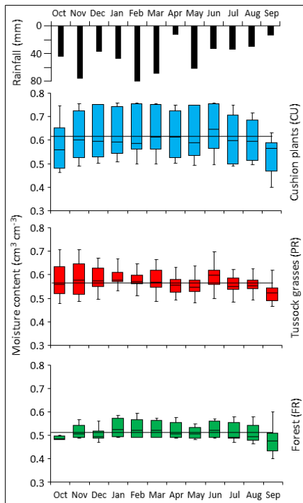
315 Figure 4: Mean monthly rainfall (mm) and mean monthly soil moisture content ( \text{cm}^3.\text{cm}^{-3} ) in soils under cushion-forming plants (mean annual SWC \pm 1 SD: 0.61 \pm 0.08 \text{ cm}^3.\text{cm}^{-3} ), tussock grasses ( 0.57 \pm 0.04 \text{ cm}^3.\text{cm}^{-3} ) and forest ( 0.51 \pm 0.03 \text{ cm}^3.\text{cm}^{-3} ).
