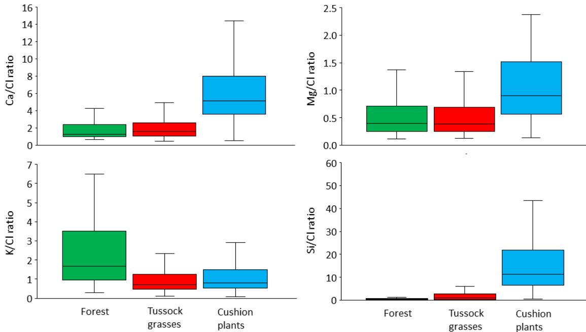
355 Figure 6: Ratio of Ca, Mg and K nutrients to Chloride in the soil solution of forests (n=7), tussock grasses (n=15) and cushion plants (n=9). An increase in the ratio indicates an enrichment of the nutrient relative to Cl, and a decrease a removal of the nutrient compared to Cl.
