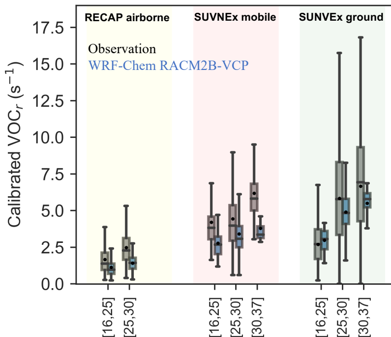
Figure 7. The comparison of the temperature dependence of VOC reactivity ( VOC_r ) between observations (gray) and WRF-Chem simulation configured with RACM2B-VCP chemical mechanism (blue). The comparison to the RECAP airborne measurement in yellow shade; SUNVEx mobile measurements in red shade and SUNVEx ground site measurements in green shade. The distribution is shown by a whisker plot; the black dot denotes the mean value and the line denotes the median value.
