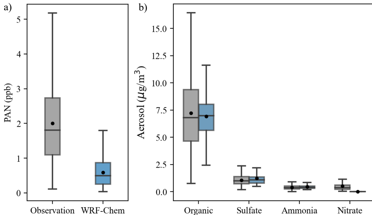
Figure 8. The comparison of PAN (a) and speciated aerosols (b) between ground observations at Pasadena (gray) and WRF-Chem simulation with RACM2B-VCP mechanism (blue). The distribution is shown by a whisker plot; the black dot denotes the mean value and the line denotes the median value.
