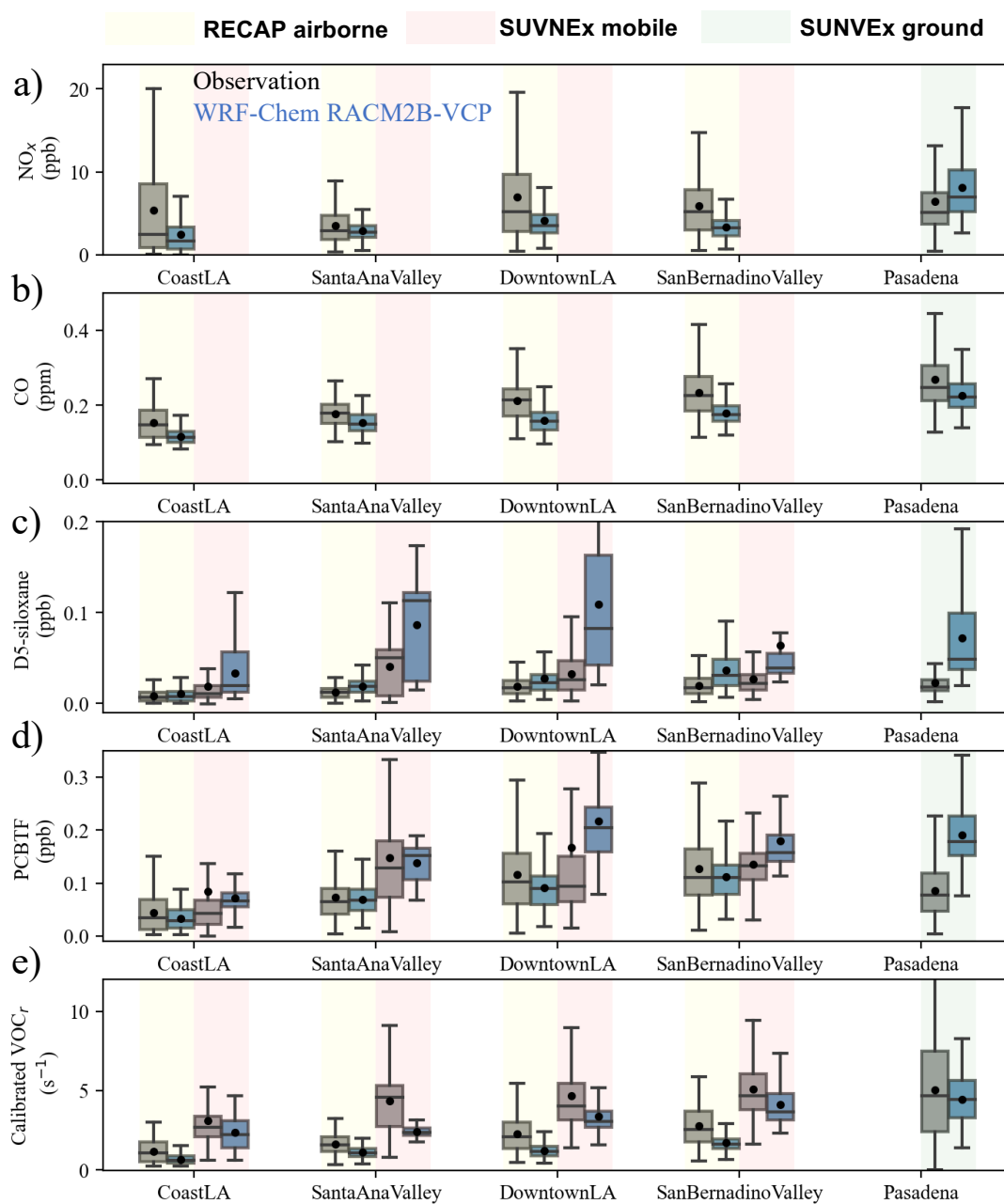
Figure 5. The comparison of \text{NO}_x (a), CO (b), D5-Siloxane (c), PCBTF (d) and calibrated \text{VOC}_r between observations and WRF-Chem simulation configured with RACM2B-VCP chemical mechanism. The comparison to the RECAP airborne measurement in yellow shade; SUNVEx mobile measurements in red shade and SUNVEx ground measurements in green shade. The distribution is shown by a whisker plot; the black dot denotes the mean value and the line denotes the median value.
