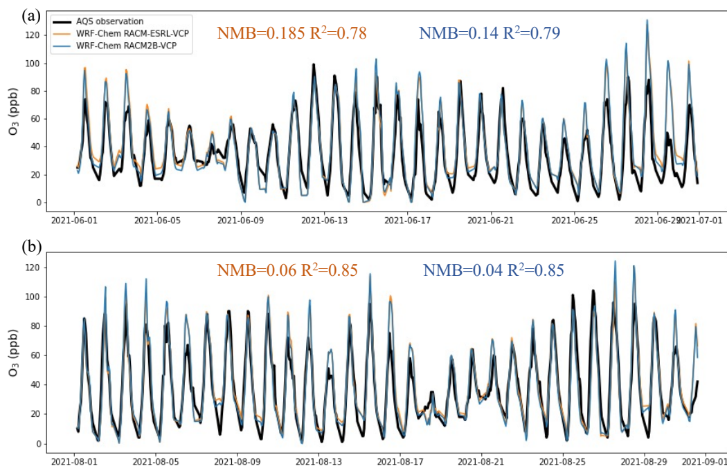
Figure 2. The comparison of time series of hourly O_3 between AQS site and two WRF-Chem simulations, one with RACM-ESRL-VCP and another one with RACM2B-VCP chemical mechanism at AQS site at Pasadena. The corresponding NMB and R^2 between model simulations and observations of hourly O_3 are shown on each plot.
